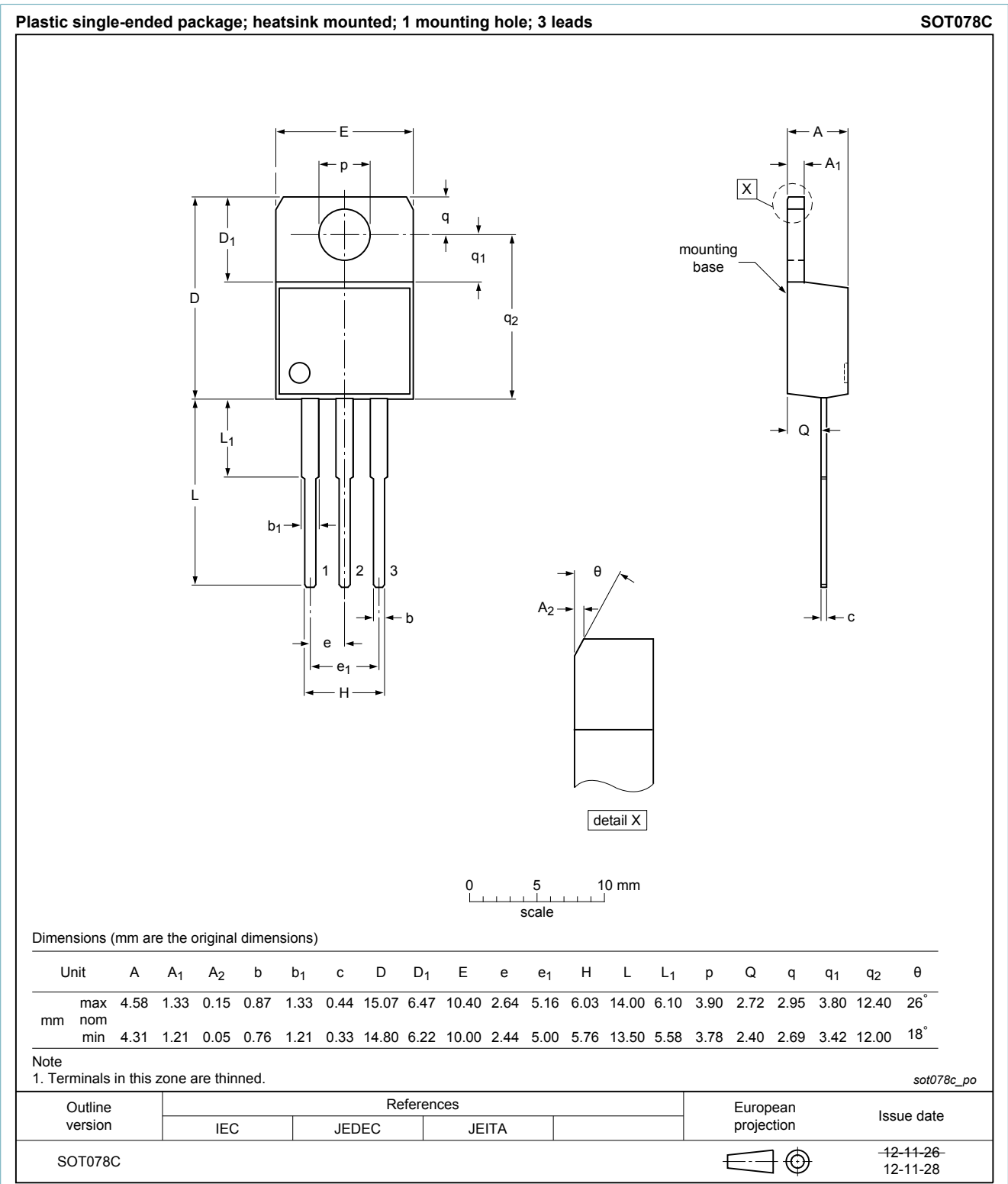
Fig. 1. Package outline TO-220AB (SOT78C)
