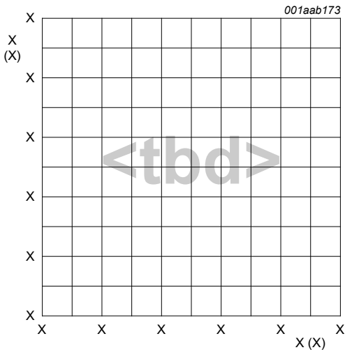
Fig. 2. Reflow soldering footprint for TO-220AB (SOT78C)
