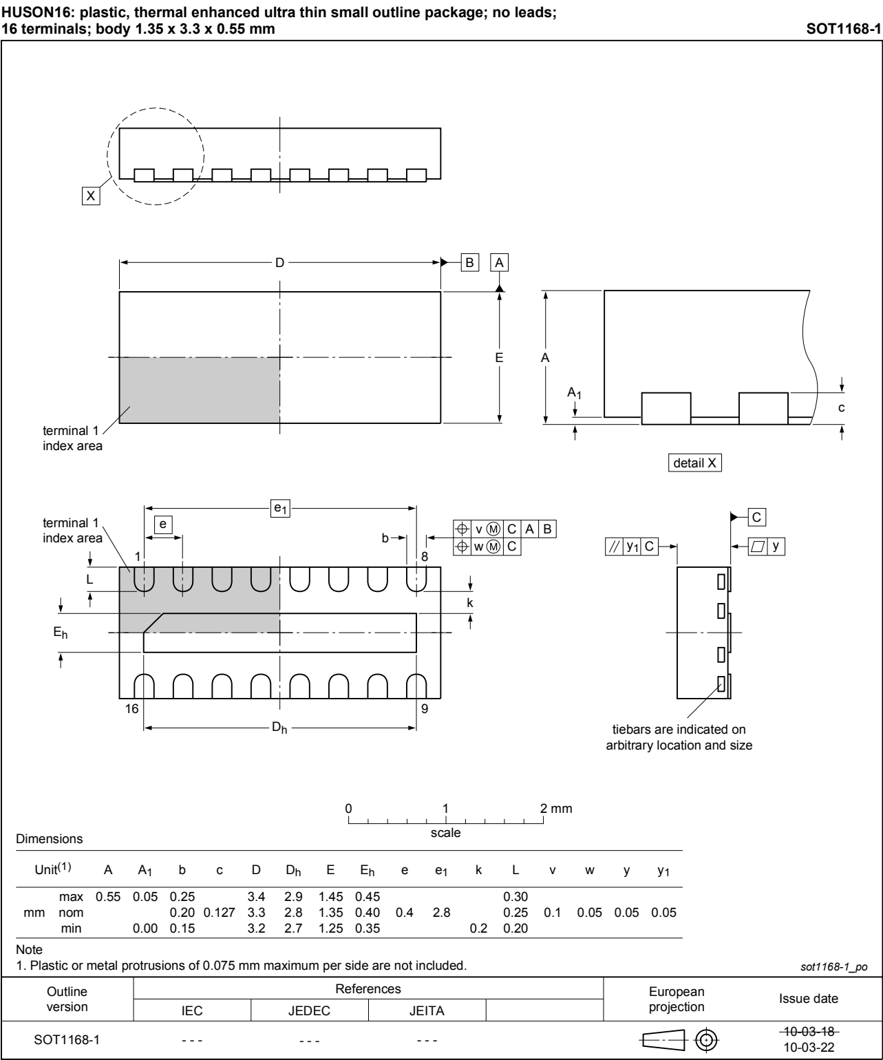
Fig. 1. Package outline DFN3314-16 (SOT1168-1)
