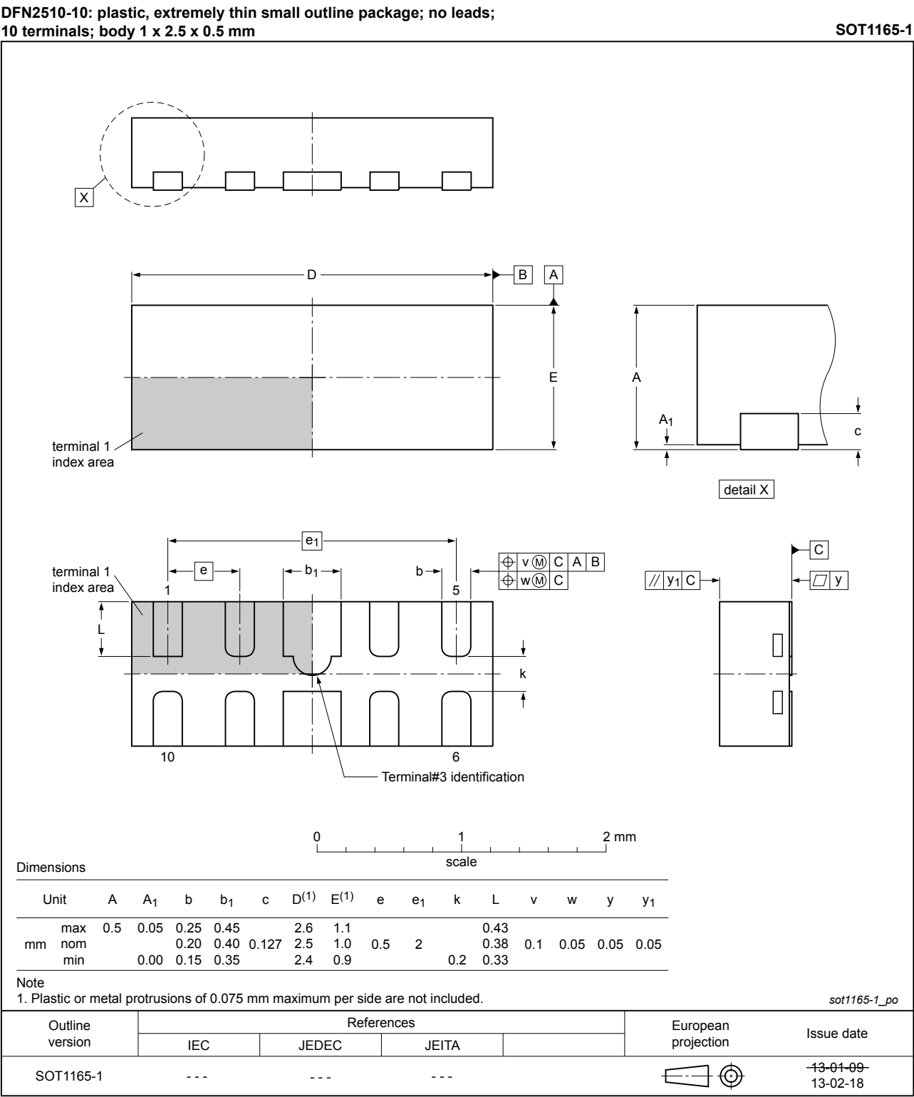
Fig. 1. Package outline DFN2510-10 (SOT1165-1)
