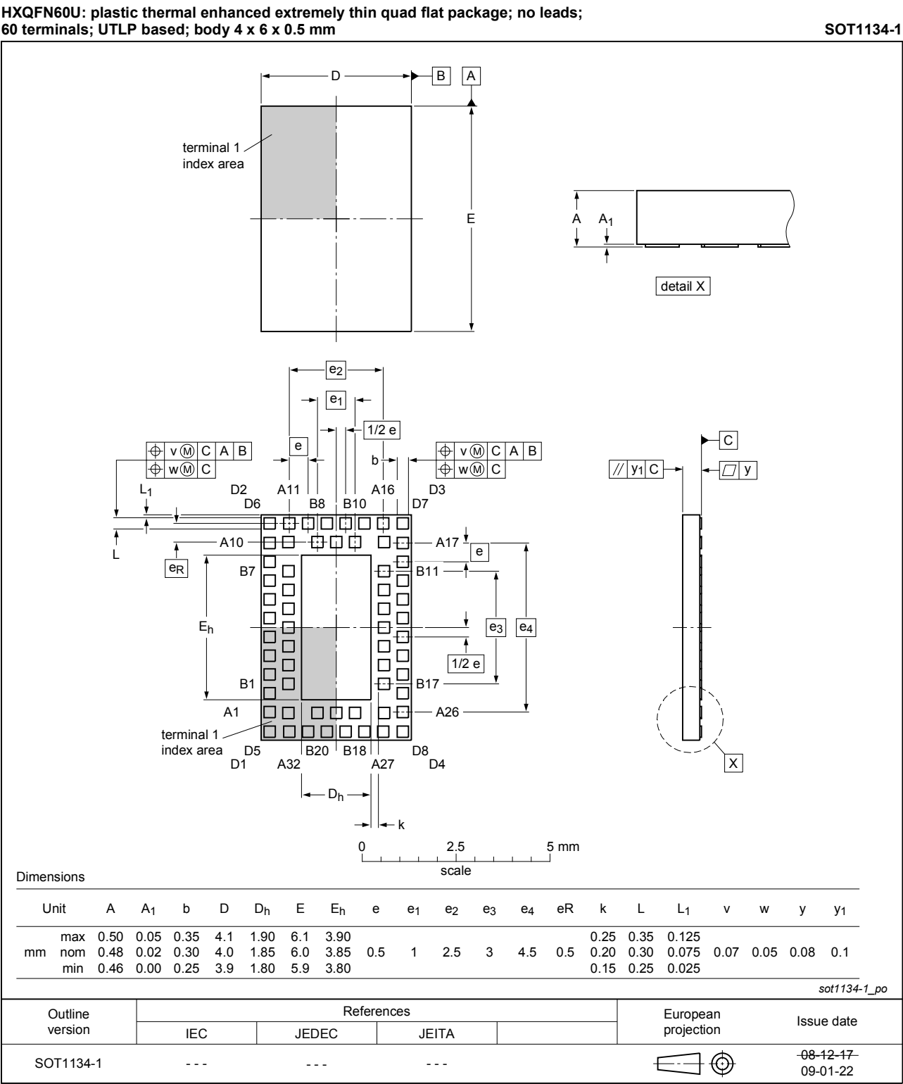
Fig. 1. Package outline HXQFN60U (SOT1134-1)
