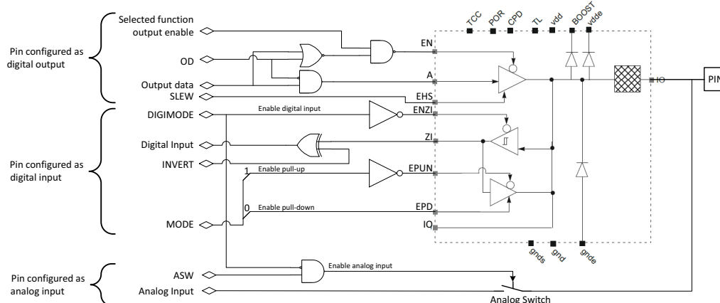
Fig 44. Standard GPIO pin configuration
