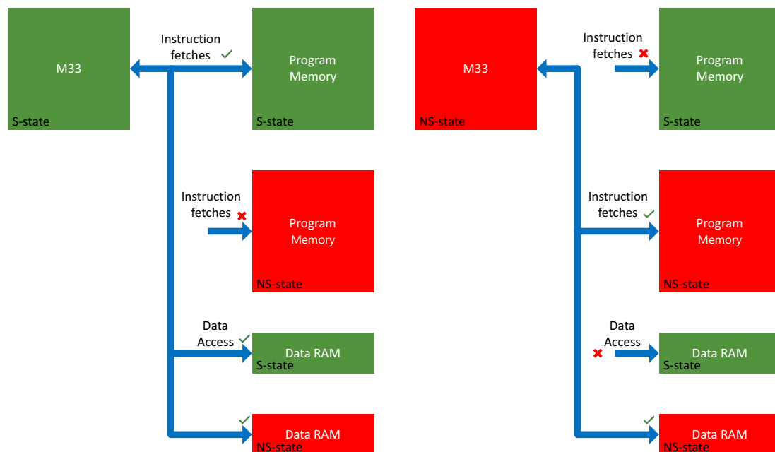
Fig 149. Secure state and Non-secure state view for TrustZone for ARMv8
