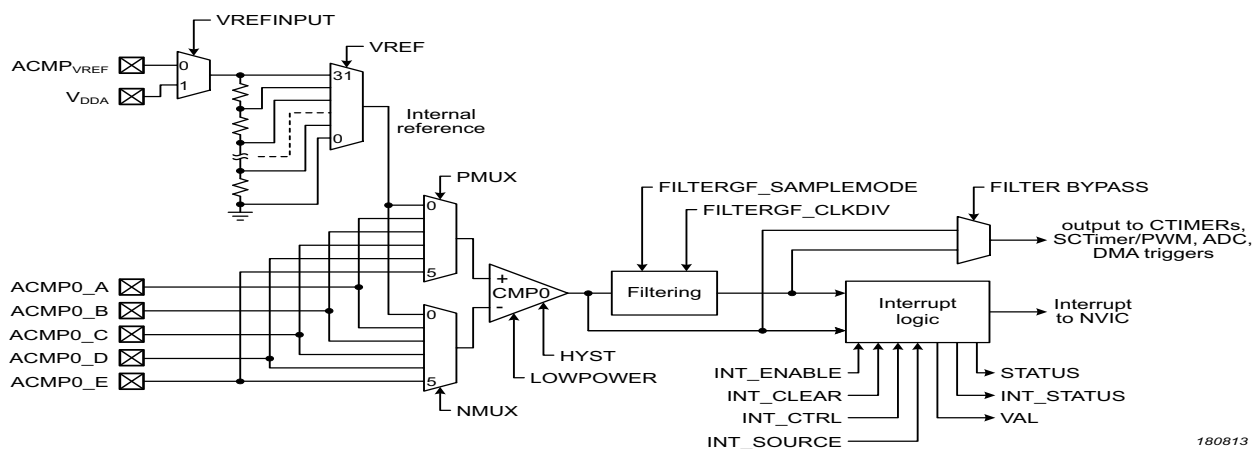
Fig 129. Comparator block diagram
