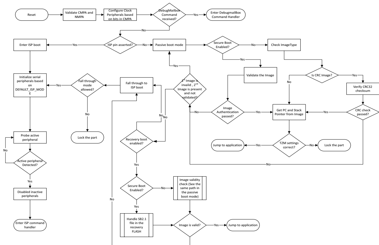
Fig 8. LPC55S0x/LPC550x boot flow chart
