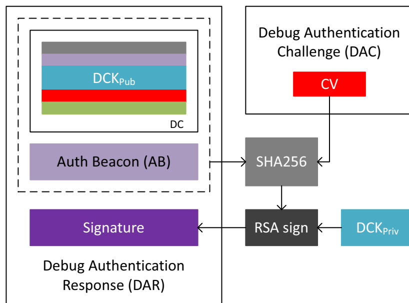
Fig 177. Debug Authentication Response (DAR) fields
