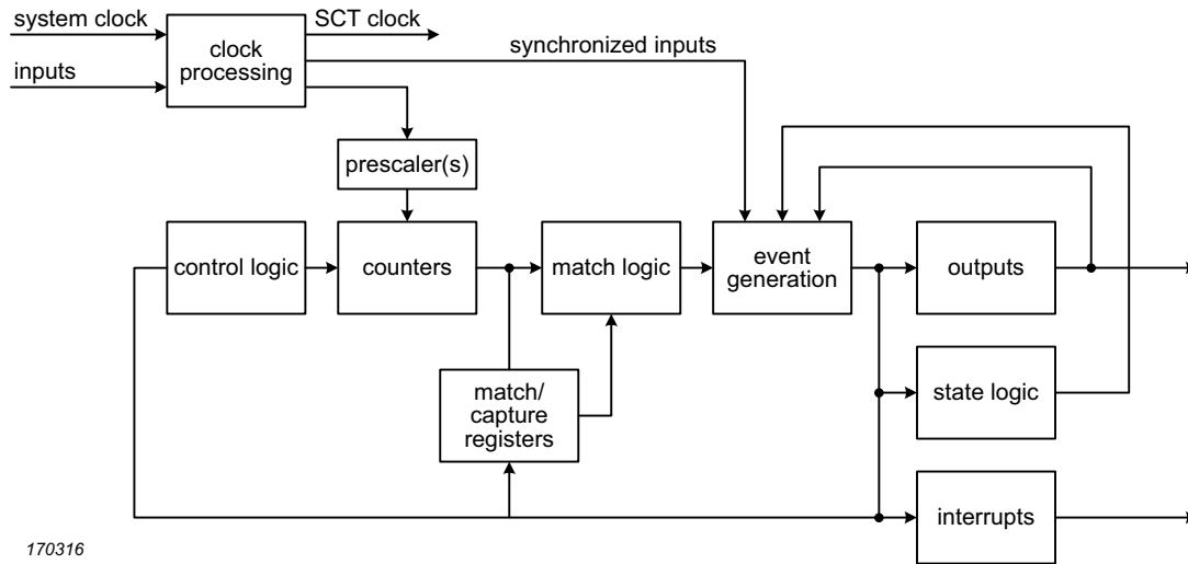
Fig 68. SCTimer/PWM block diagram
