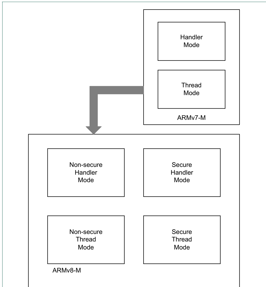
Fig 148. Cortex-M4 (or M3) vs Cortex-M33
