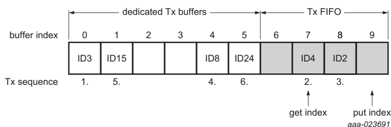
Fig 144. Example of mixed configuration dedicated Tx buffers / Tx FIFO
