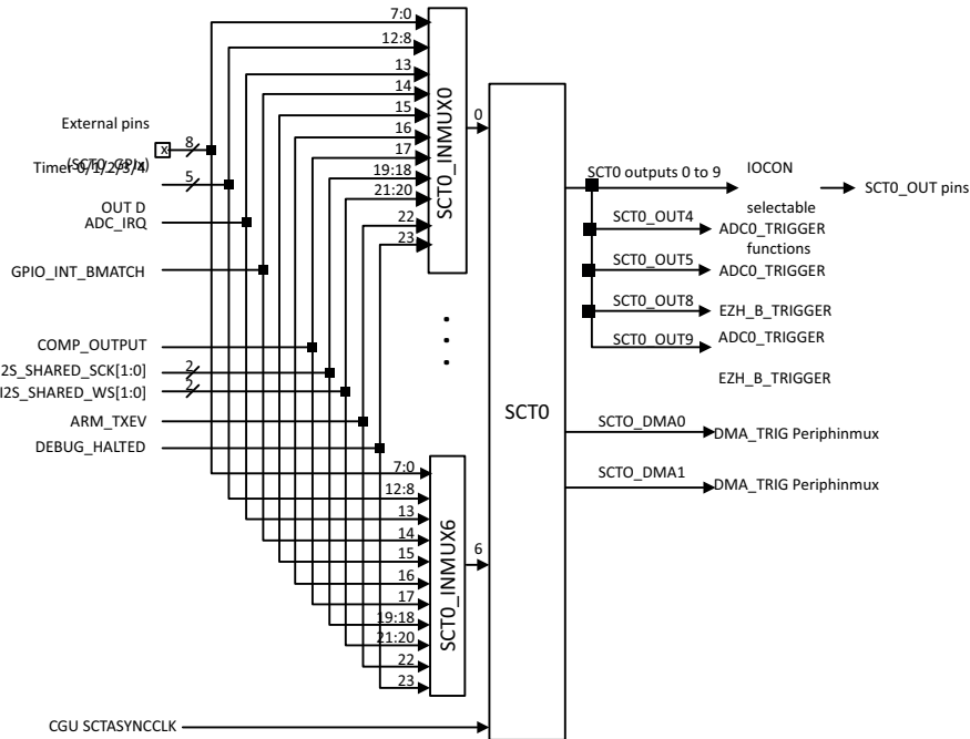
Fig 48. SCT0 input multiplexing
