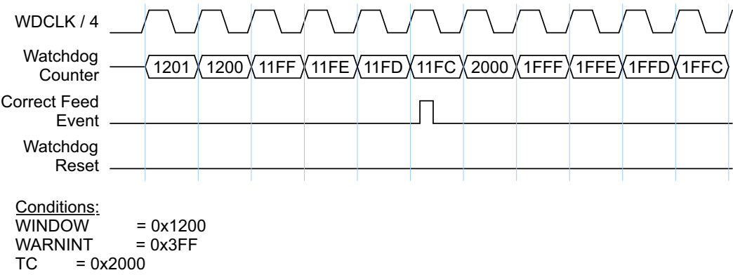
Fig 89. Correct watchdog feed with windowed mode enabled
