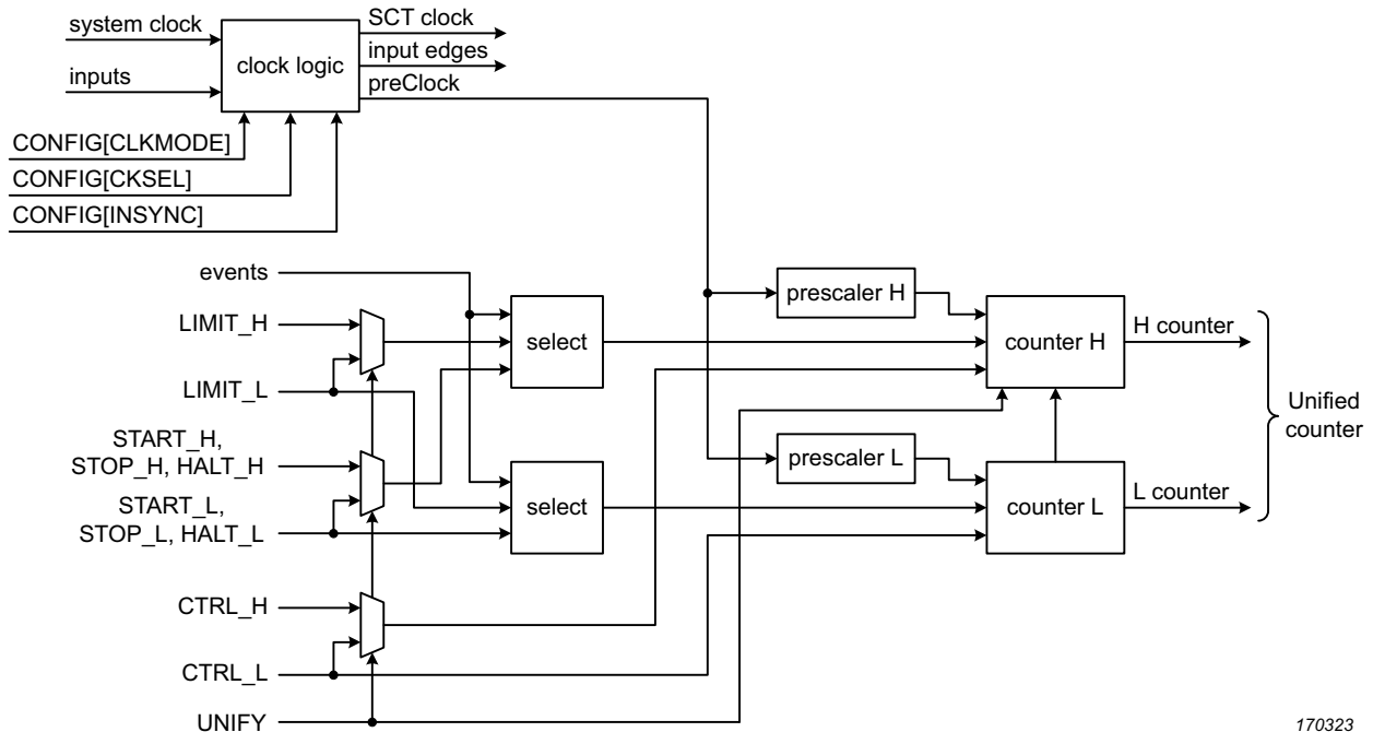
Fig 69. SCTimer/PWM counter and select logic
