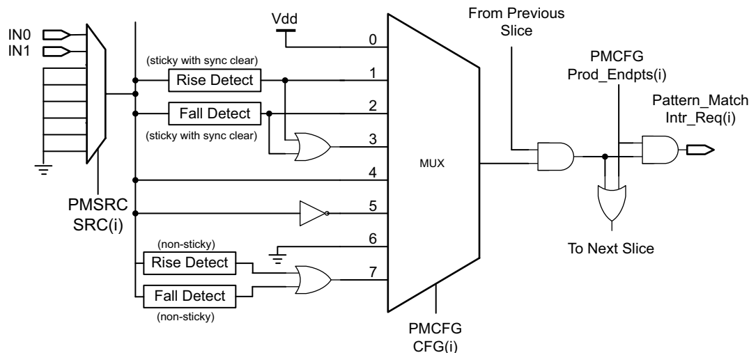
Fig 60. Secure pattern match bit slice with detect logic
