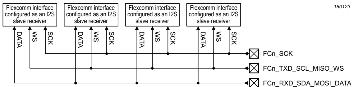
Fig 107. I 2 S signal sharing example, multiple slave receivers
