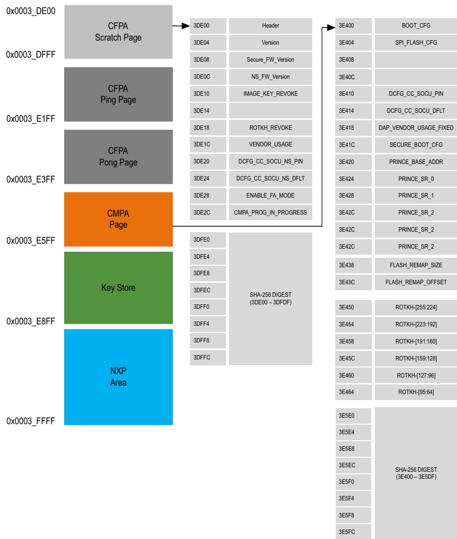
Fig 10. Protected Flash Region
