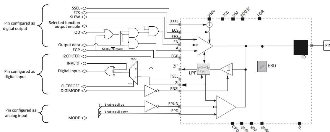
Fig 45. Combo I 2 C/GPIO pin configuration
