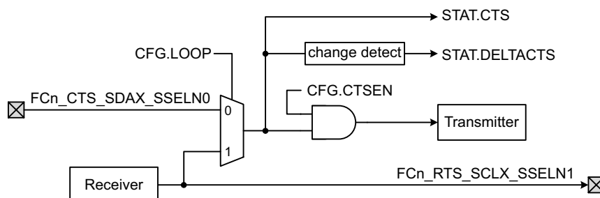
Fig 97. Hardware flow control using RTS and CTS
