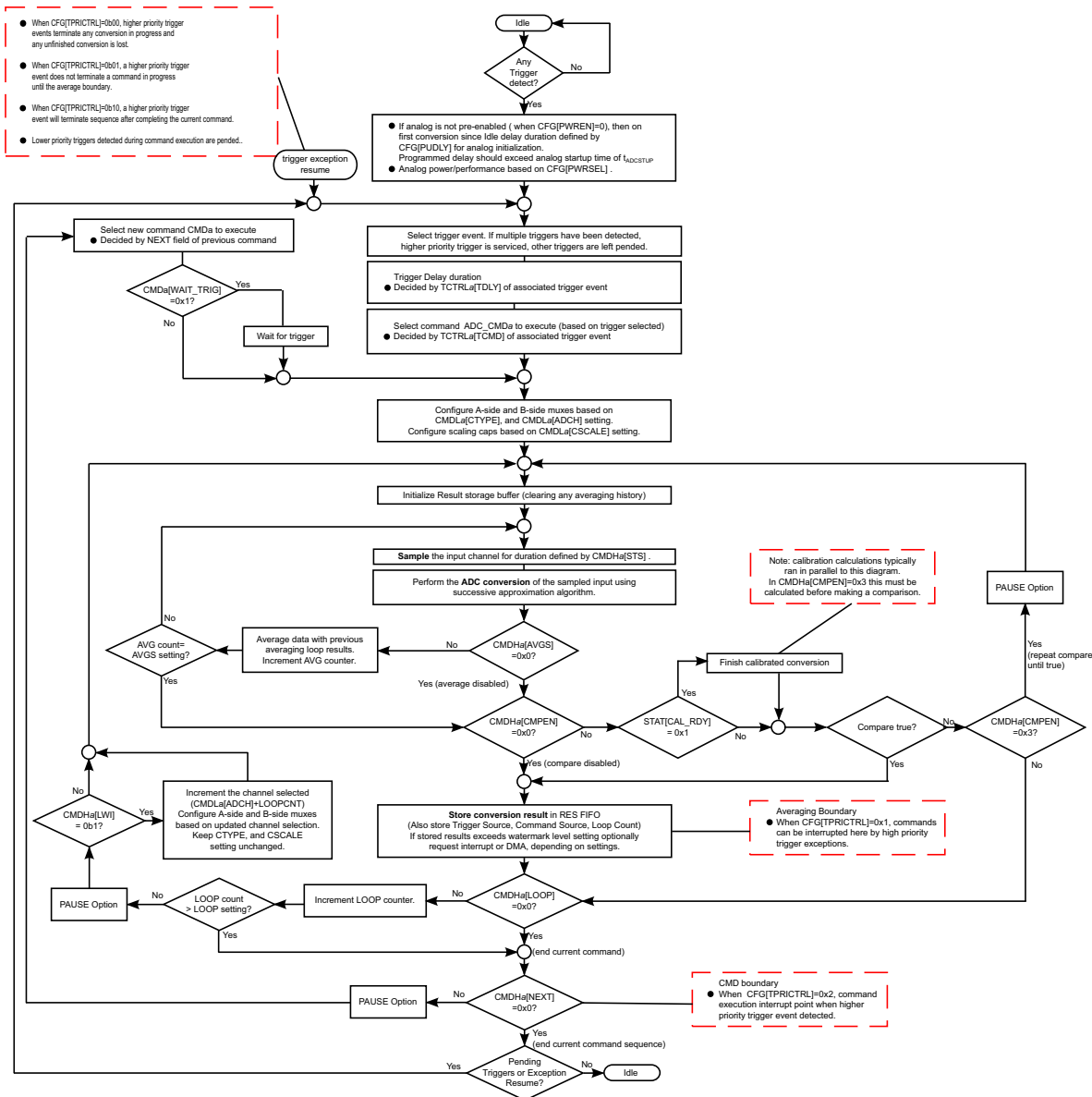
Fig 126. ADC command sequencing
