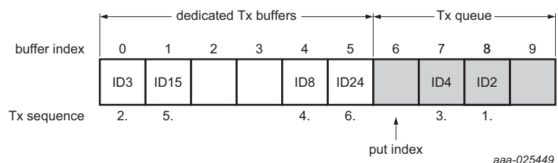
Fig 145. Example of mixed configuration dedicated Tx buffers / Tx queue
