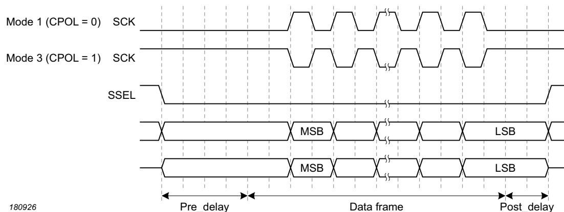
Fig 100. Pre_delay and Post_delay
