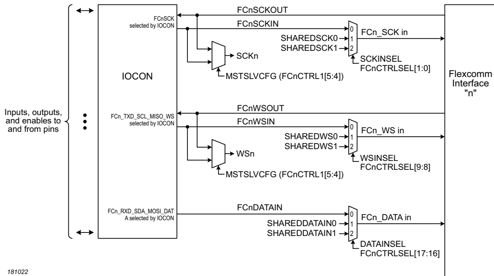
Fig 104. Shared signal connections for each Flexcomm Interface
