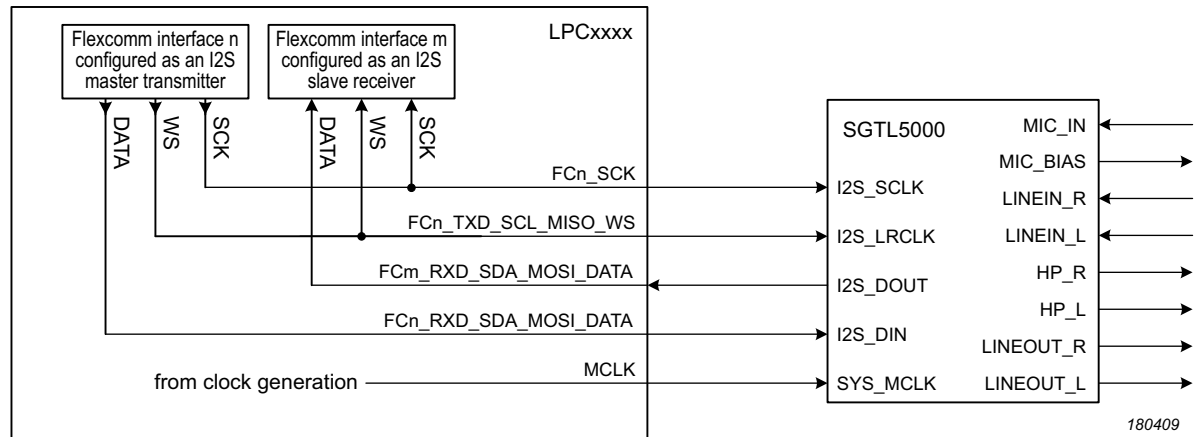
Fig 106. Example connection to an I 2 S bidirectional codec
