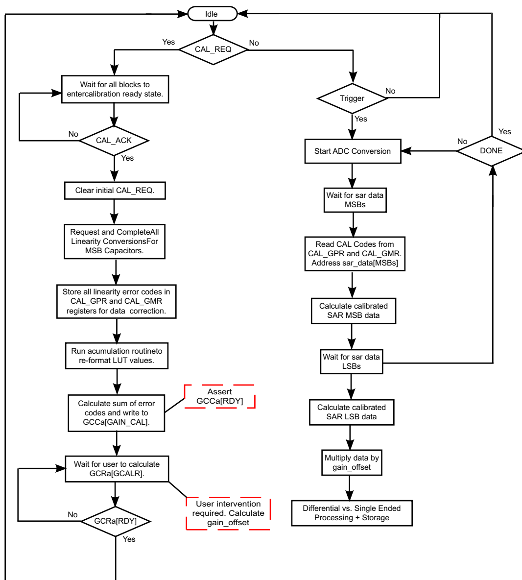
Fig 128. ADC calibration sequence
