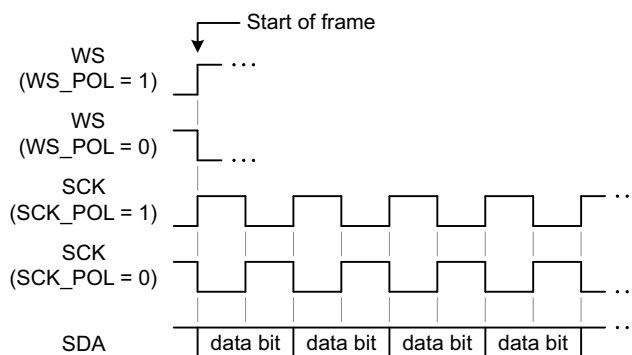
Fig 122. Data at the start of a frame, shown with both SCK and WS polarities
