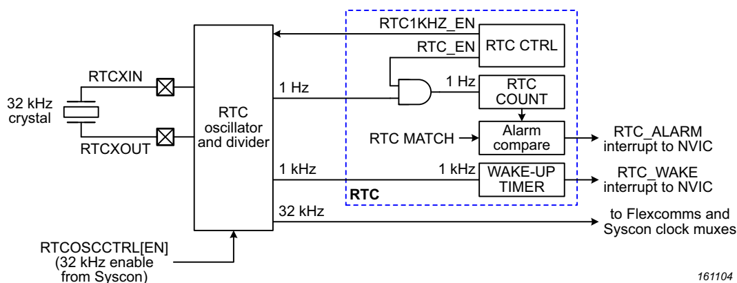
Fig 84. RTC clocking and block diagram
