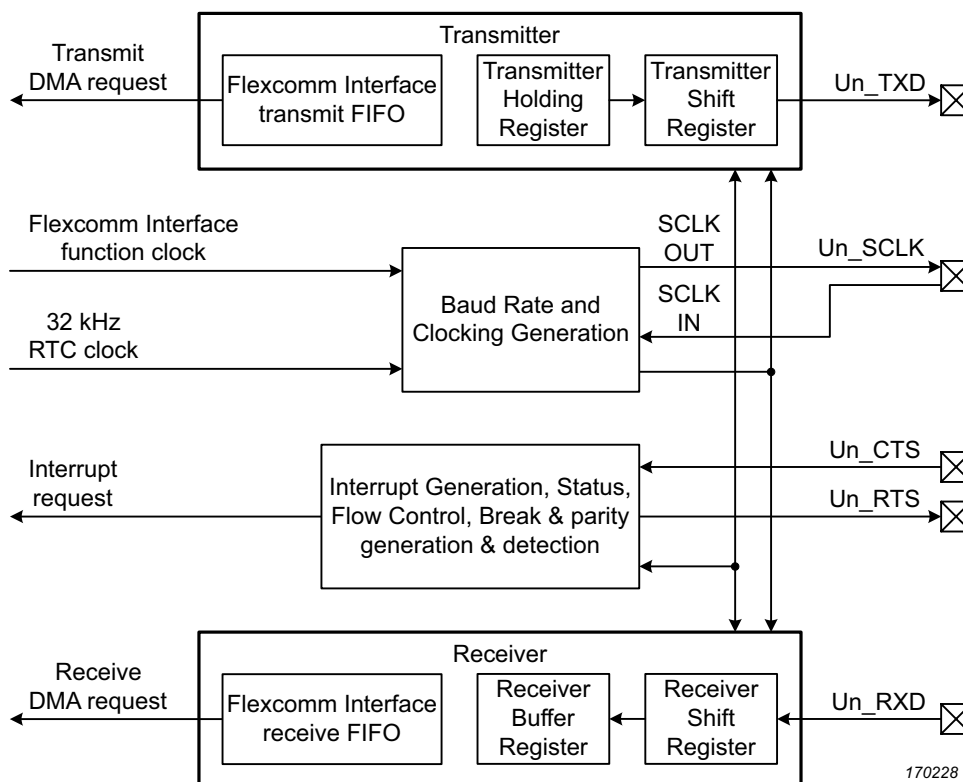
Fig 96. USART block diagram
