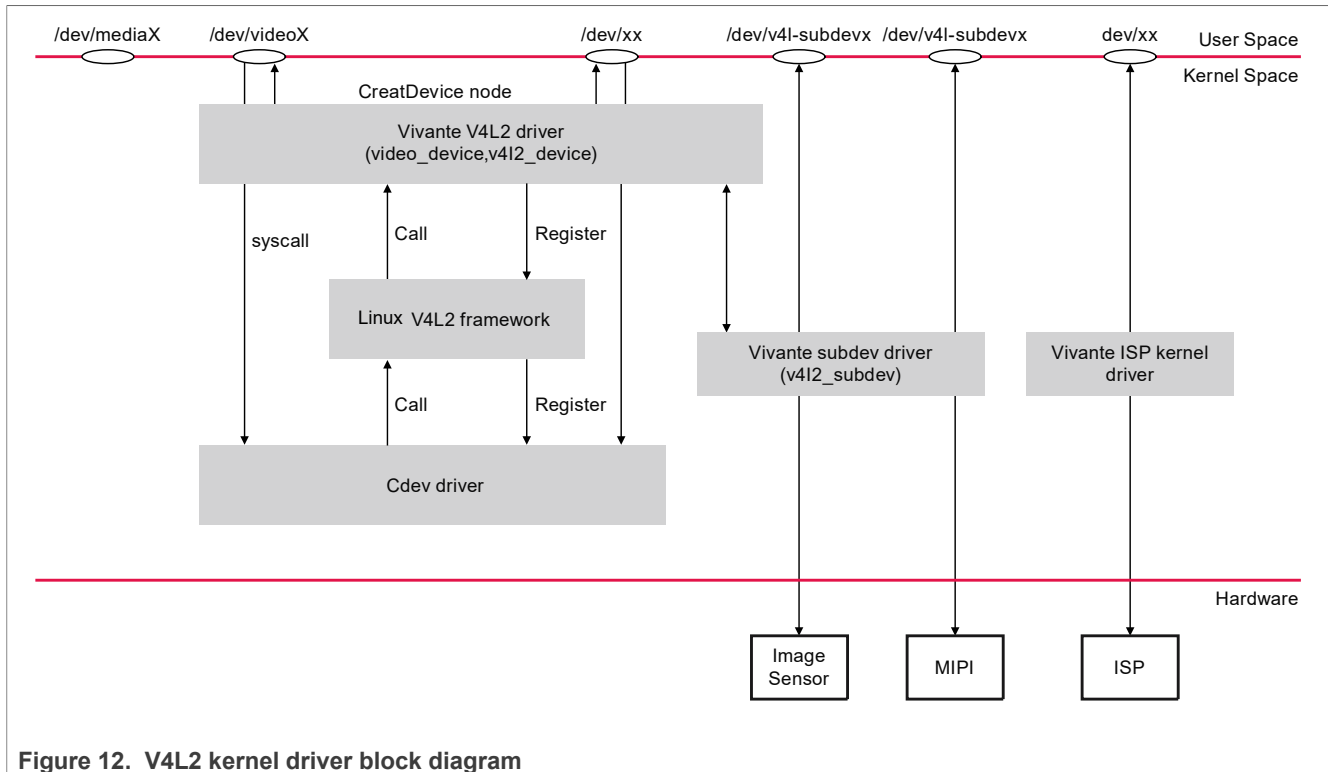
Figure 12. V4L2 kernel driver block diagram
