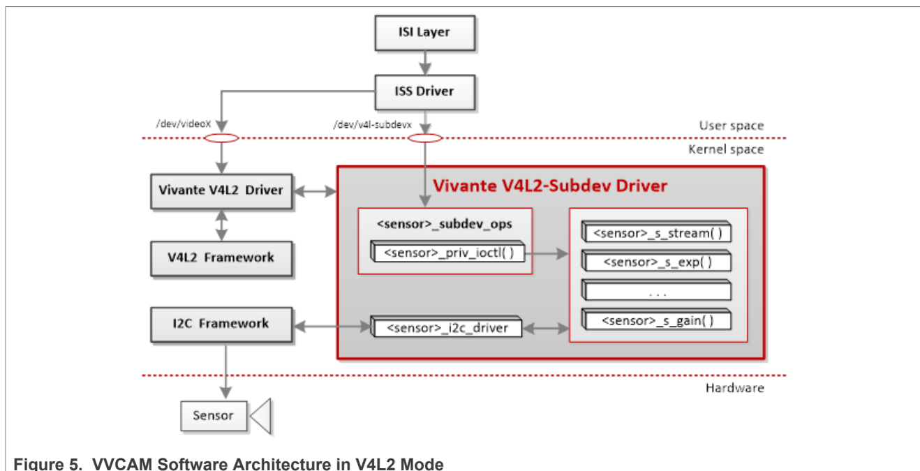
Figure 5. VVCAM Software Architecture in V4L2 Mode
