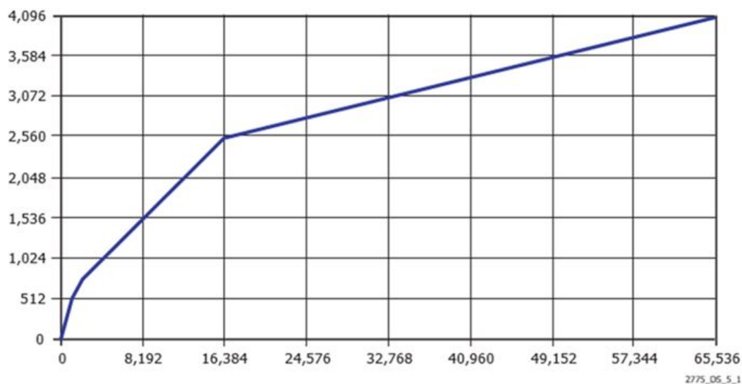
Figure 6. 16-bit to 12-bit PWL compression
