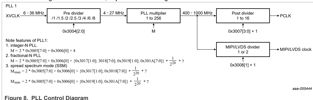
Figure 8. PLL Control Diagram
