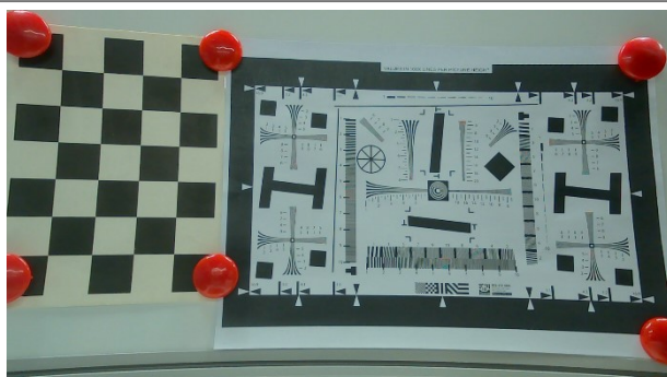
Figure 23. Dewarp Mode: FISHEYE DEWARP
