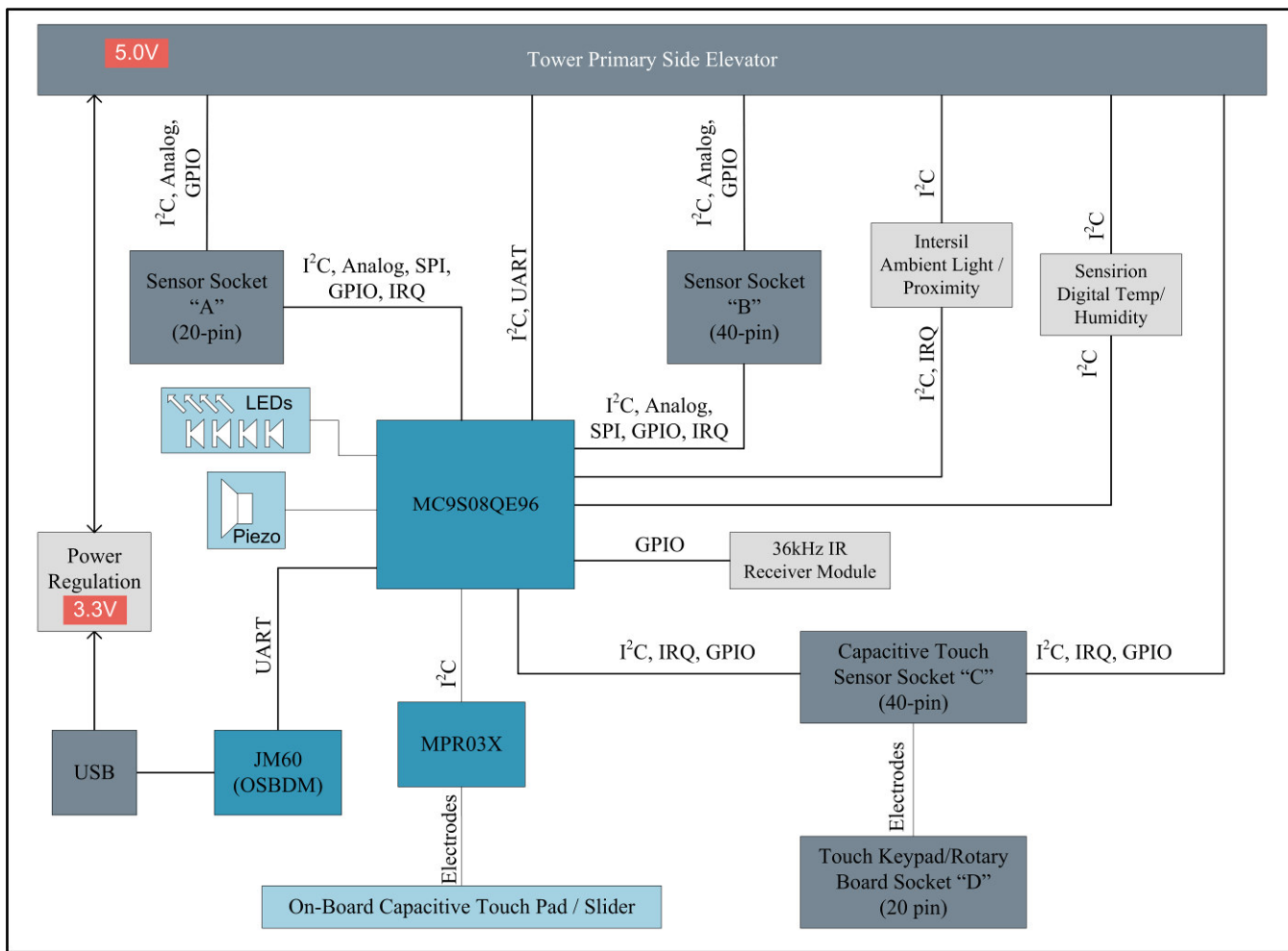
Figure 1 - TWR-SENSOR Block Diagram
