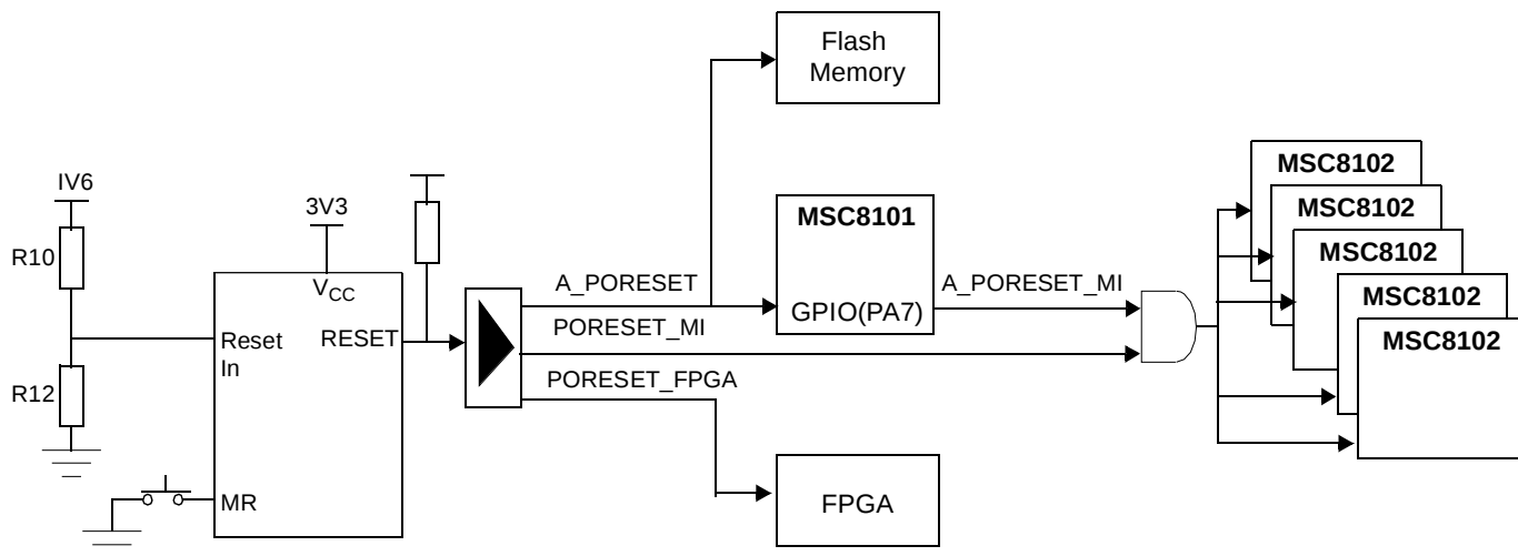
Figure 11. \overline{\text{PORESET}} Scheme
