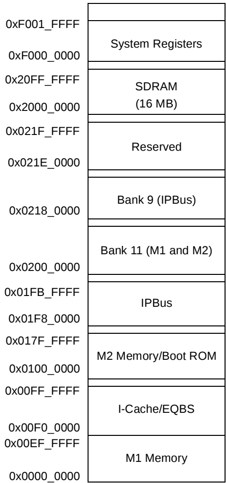
Figure 18. MSC8102 Memory Map
