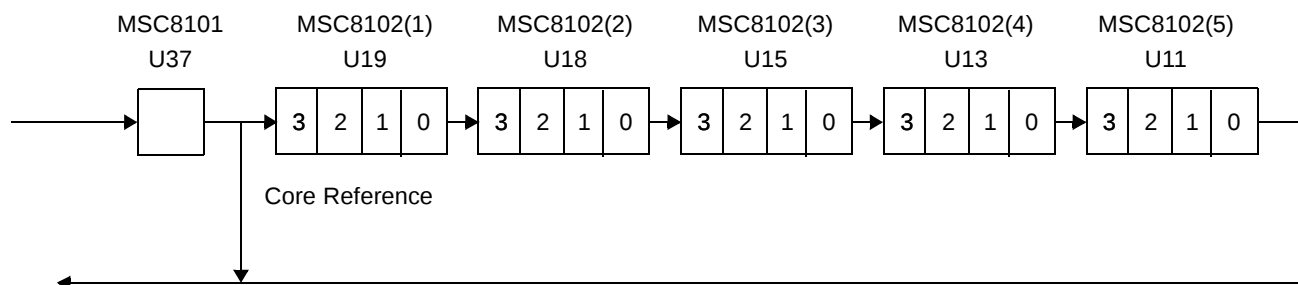
Figure 16. JTAG Chain
