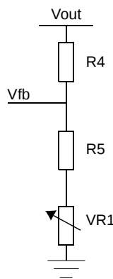
Figure 15. Setting Vout with Resistor-Divider
