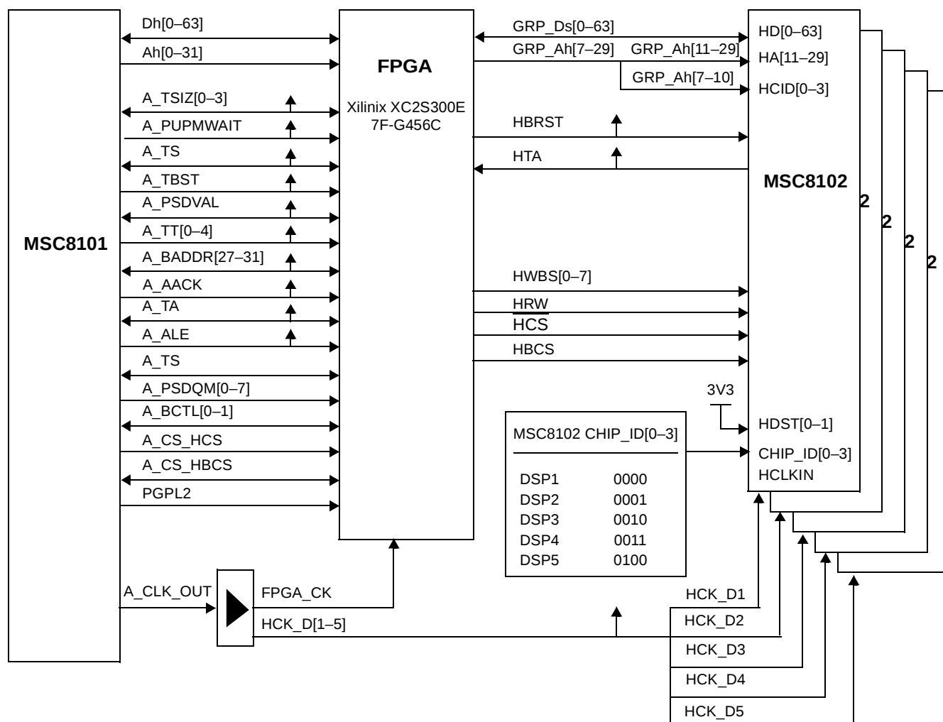
Figure 6. PFC-to-DSI Interface
