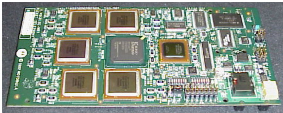
Figure 1. MSC8102 Packet Telephony Farm Card (MSC8102PFC)
