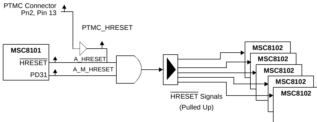
Figure 12. HRESET Scheme
