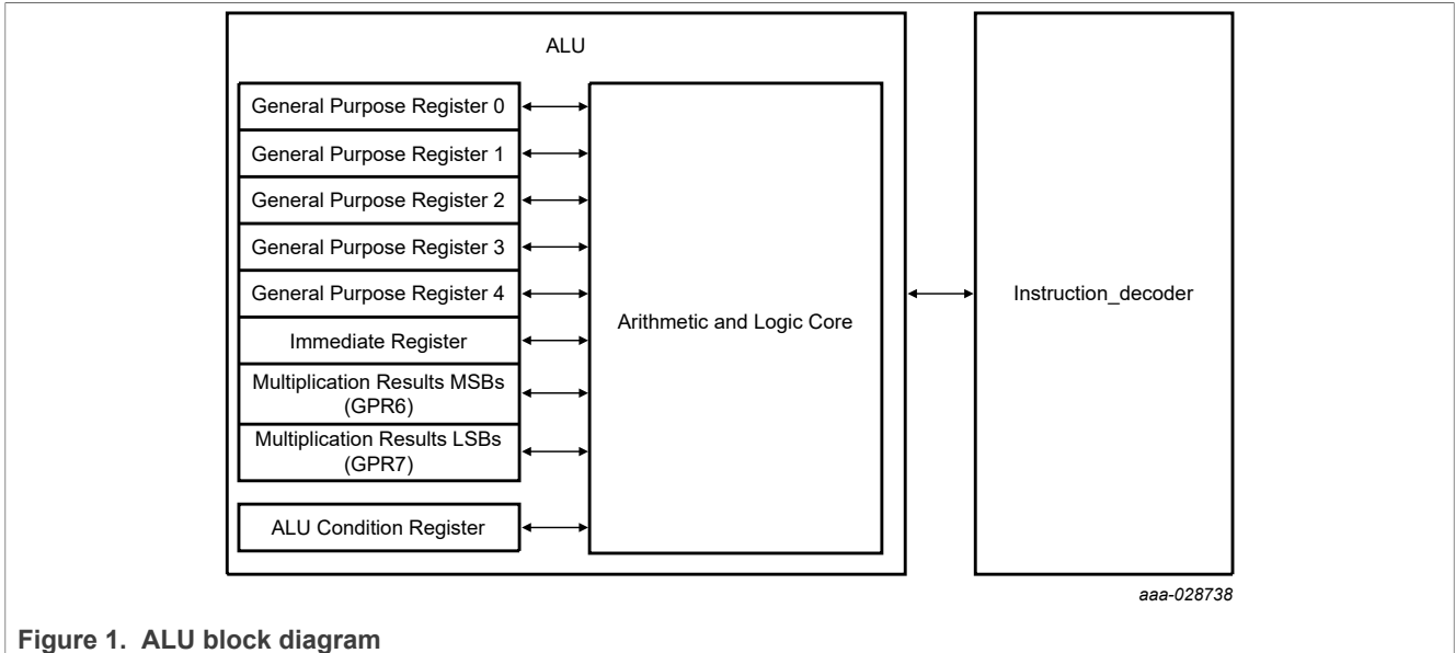
Figure 1. ALU block diagram
