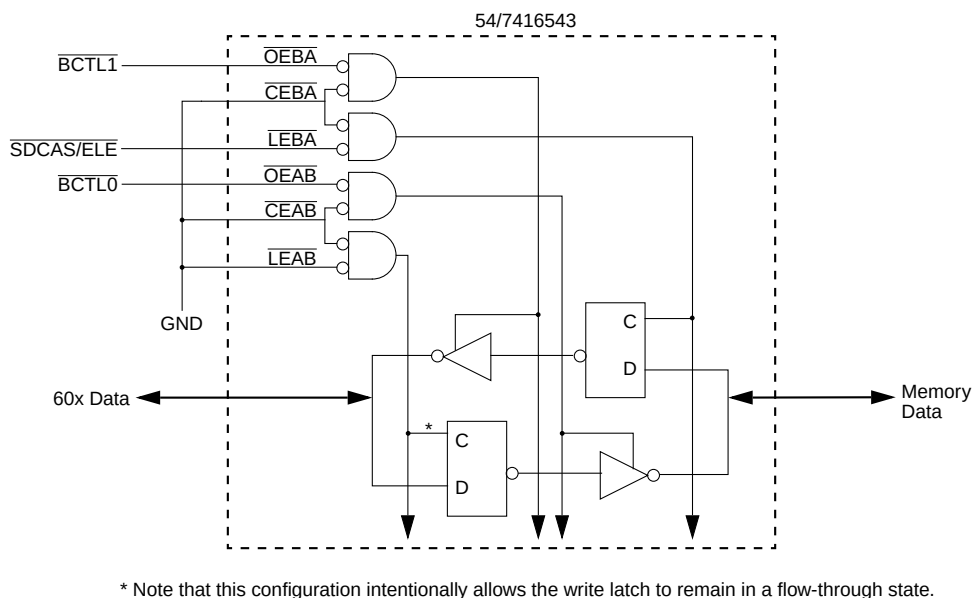
Figure 6-1. Transparent Latch-Type Buffer
