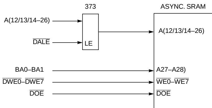
Figure 5-3. Asynchronous SRAM Interface
