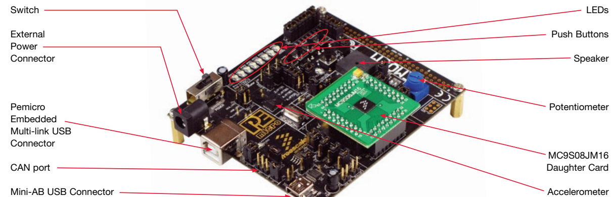
Figure 1. DEMOJM baseboard with MC9S08JM16 daughter card
