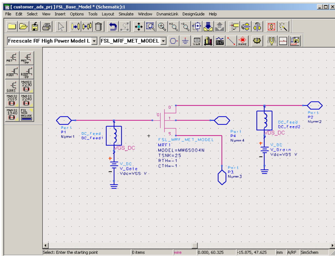
Figure 1. Schematic of FSL_Base_Model.dsn
