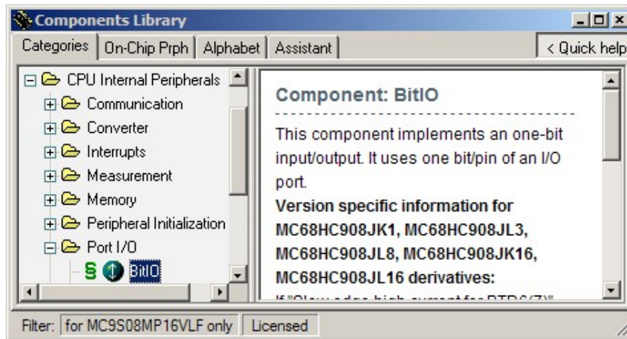
Figure 2.7 - Components Library with Quck Help panel
