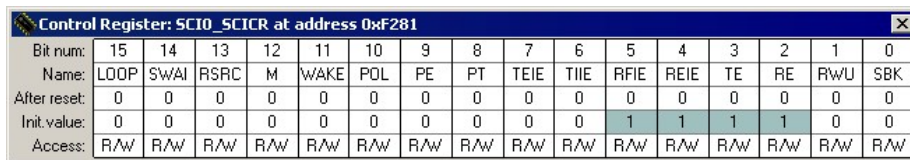
Figure 2.46 - Register Content Details
