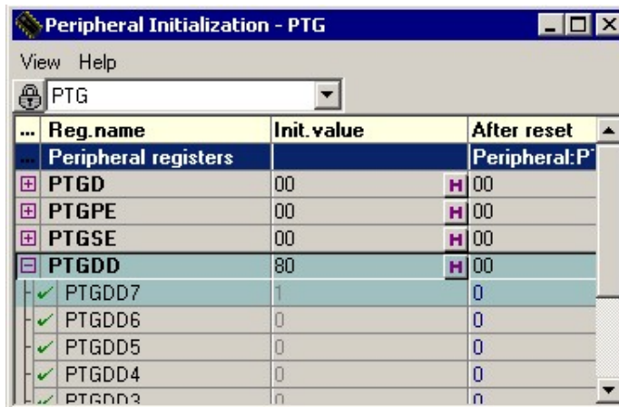
Figure 2.45 - Register List in the Peripheral Initialization window
