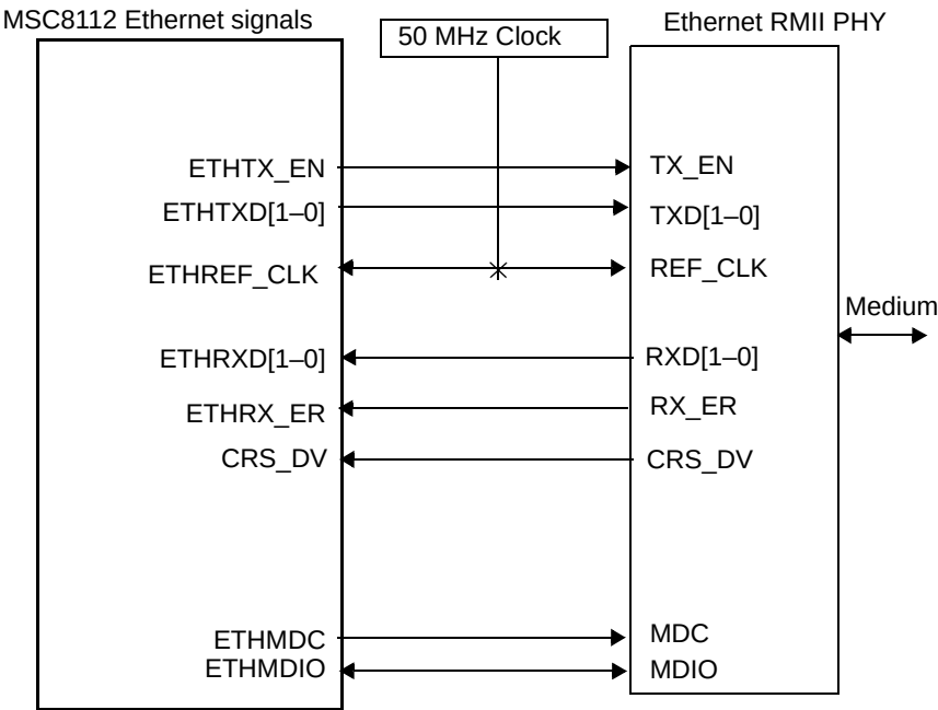
Figure 25-27. Ethernet Controller-to-PHY Connection in RMI Mode
