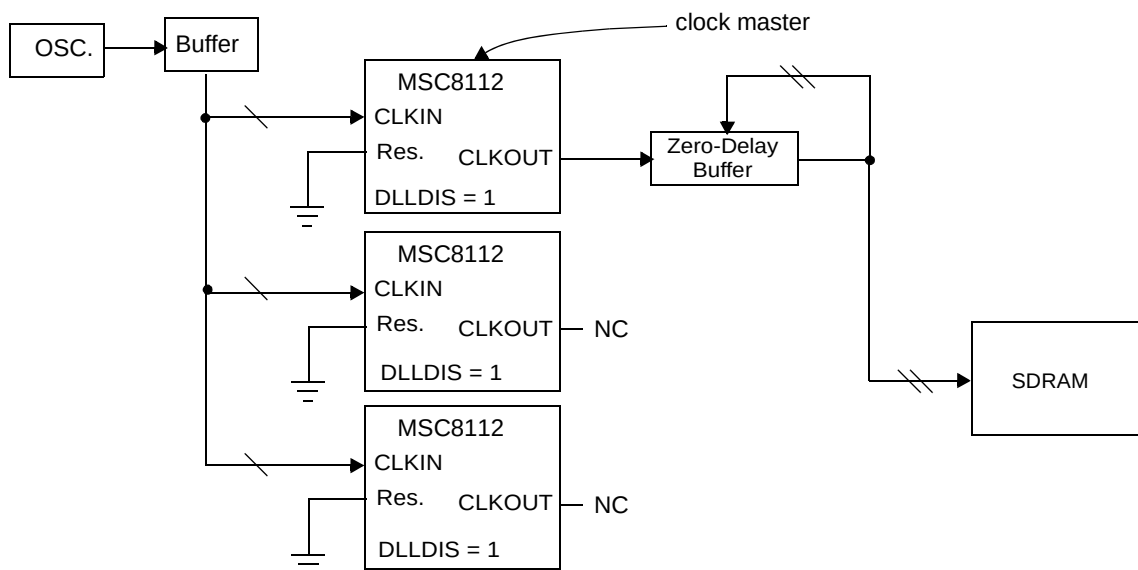
Figure 7-6. MSC8112 Clock Distribution Using CLKOUT in Multi Master Mode
