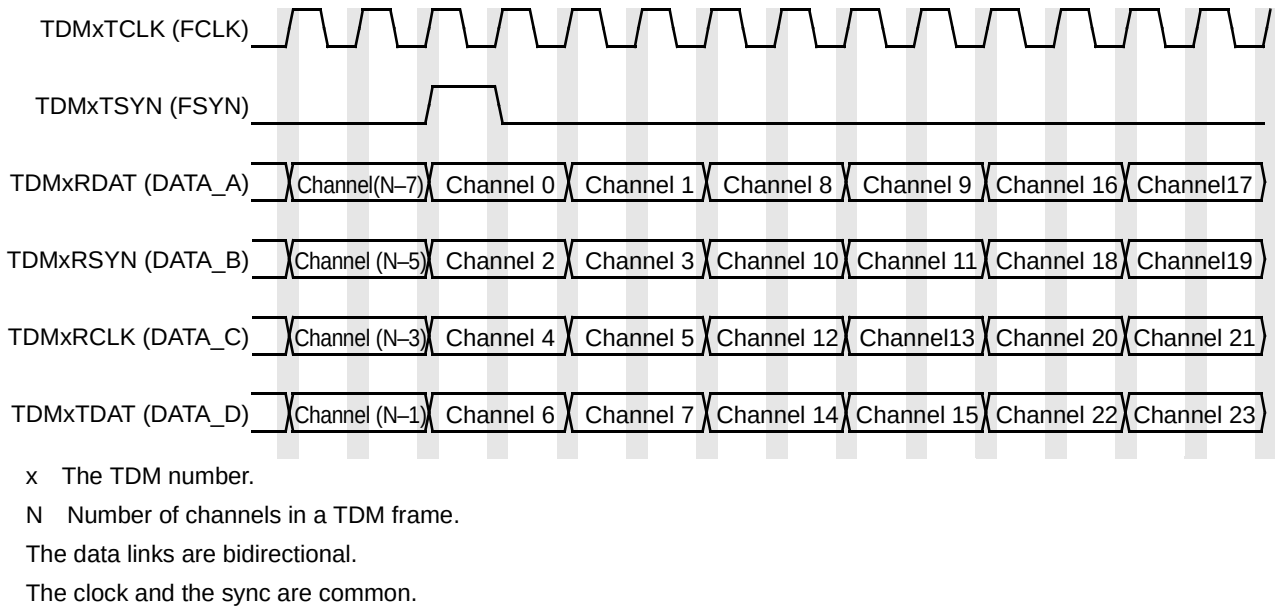
Figure 20-14. Receive and Transmit Share Sync, Clock, and Data (Four Active Links)
