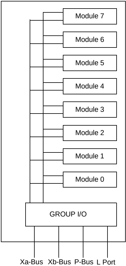
Figure 9-3. Memory Group
