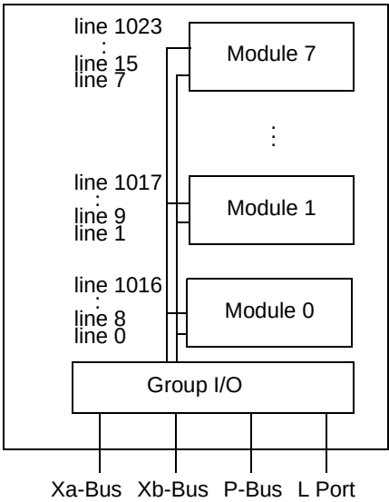
Figure 9-4. Memory Interleaving
