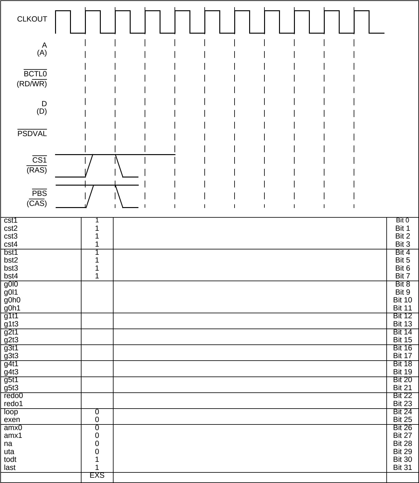
Figure 12-63. Exception Cycle
