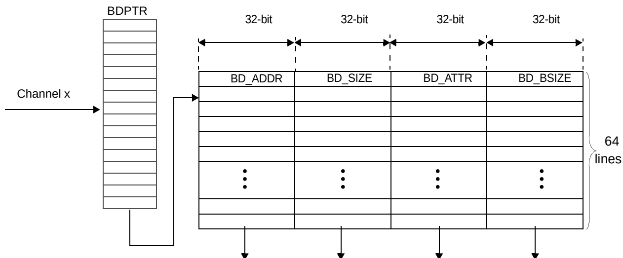
Figure 16-26. DCPRAM Structure
