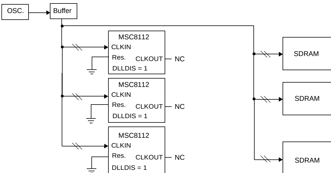
Figure 7-7. MSC8112 Clock Distribution in Multi-Master Mode Using CLKIN Example
