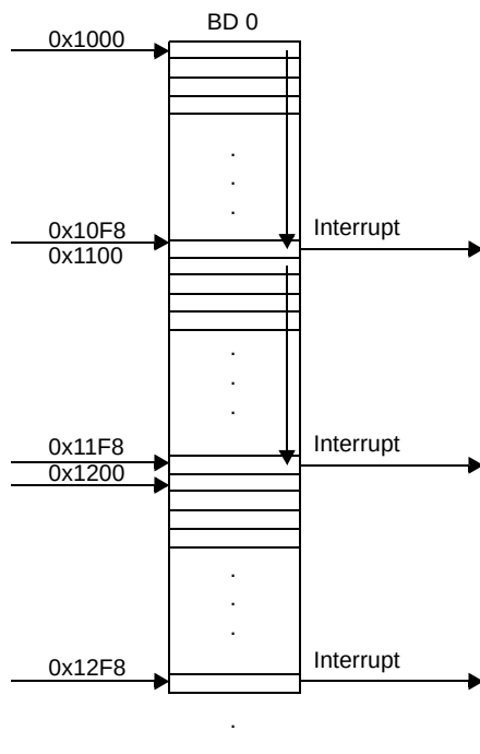
Figure 16-18. Incremental Buffer
