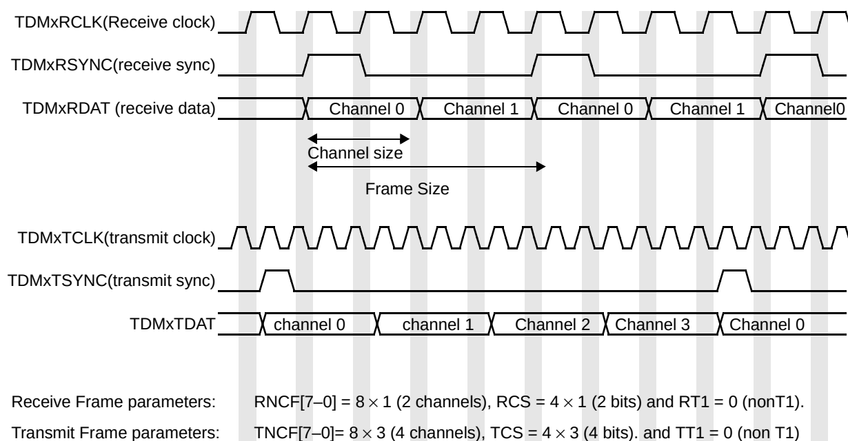
Figure 20-6. TDM Frames
