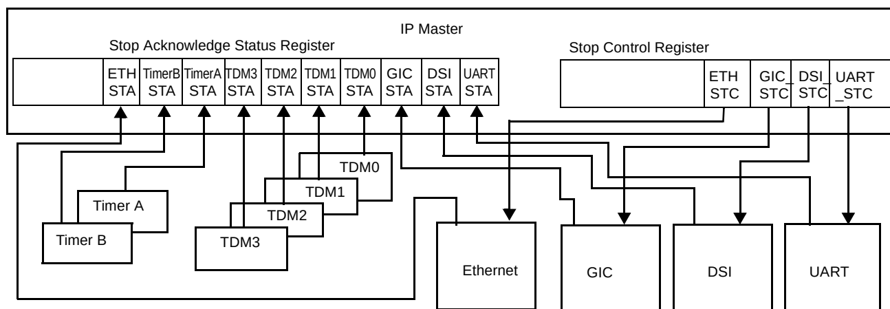
Figure 19-2. Stop Mode for Different IPBus Modules
