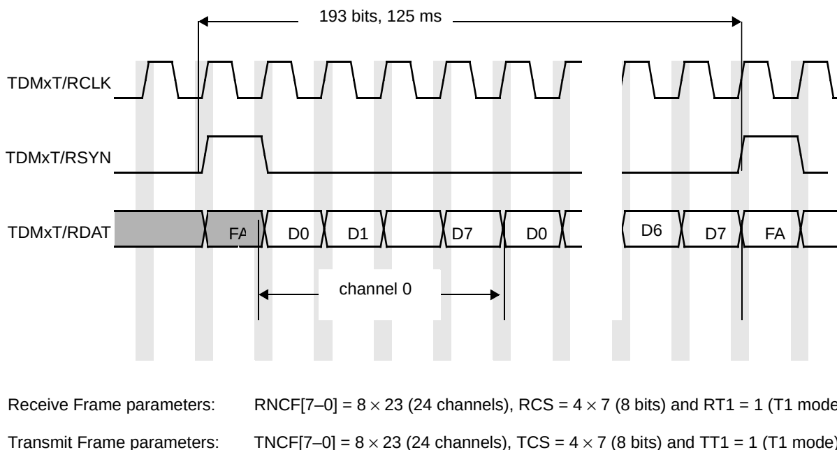
Figure 20-7. T1 Frame
