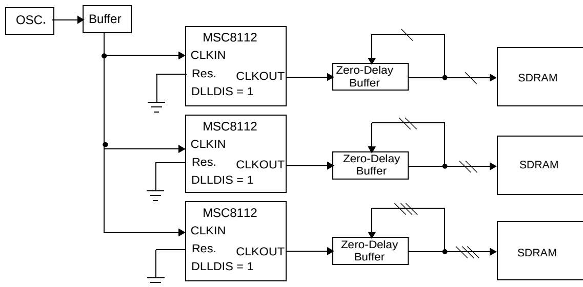
Figure 7-3. MSC8112 Clock Distribution In Single-Master Mode Using CLKOUT With Zero-Delay Buffers
