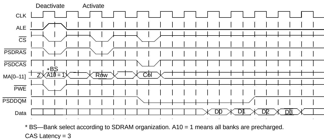
Figure 12-21. SDRAM Four-Beat Burst Read, Page Miss, CL = 3
