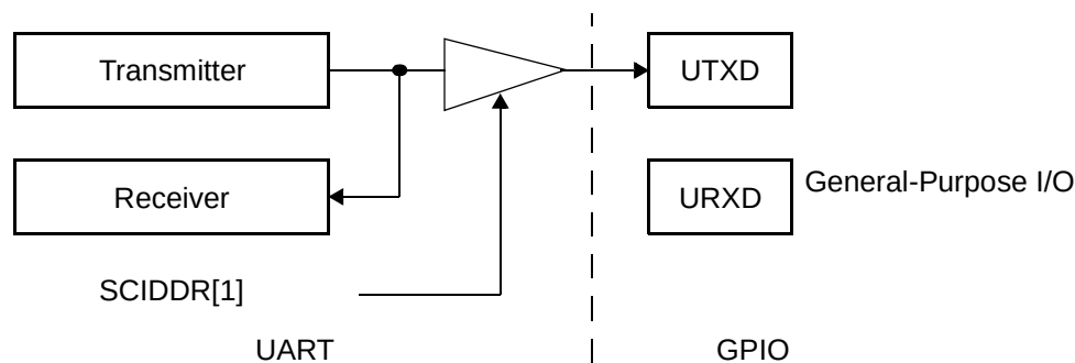
Figure 21-20. Loop Operation (LOOPS = 1, RSRC = 0)
