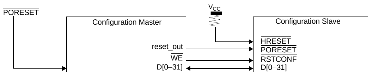
Figure 5-5. Single MSC8112 Slave Configuration
