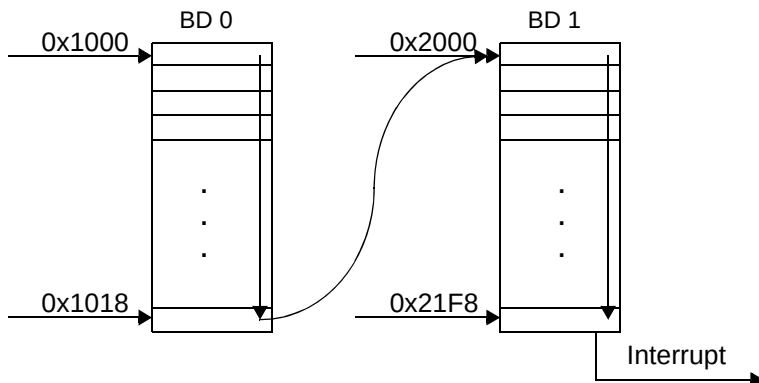
Figure 16-19. Chained Buffer
