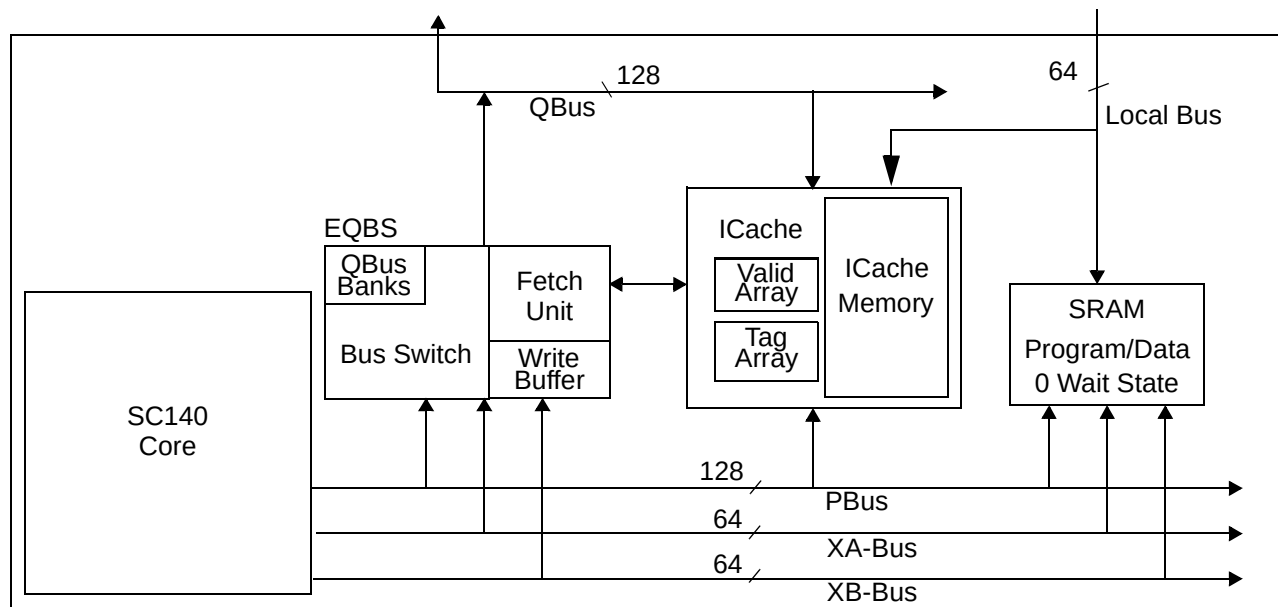
Figure 9-9. MSC8112 ICache System
