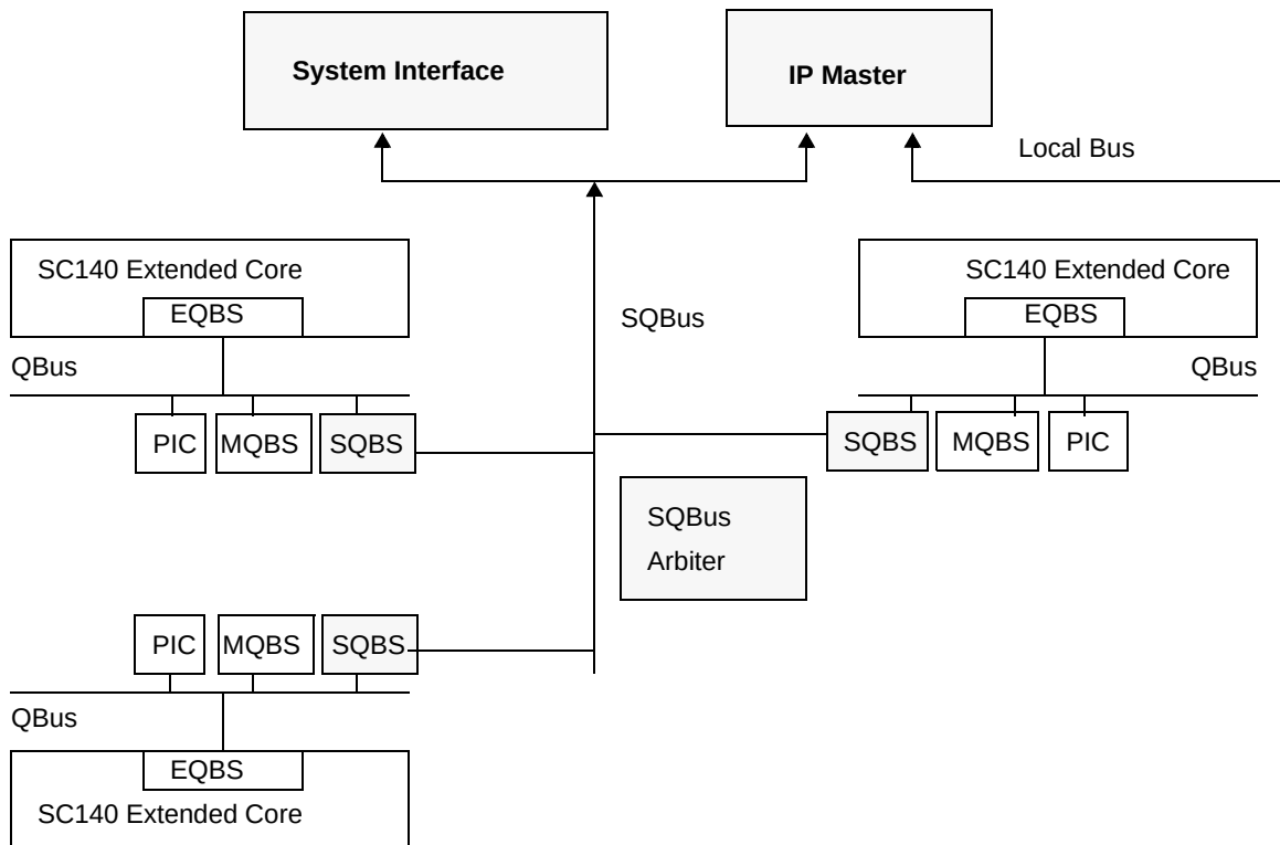
Figure 11-1. SQBus System
