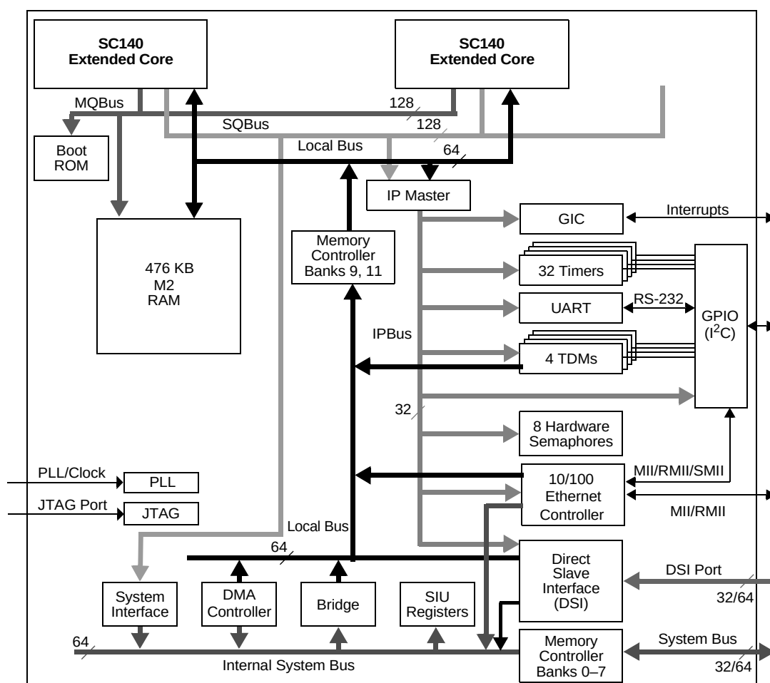
Figure 1-1. MSC8112 Block Diagram
