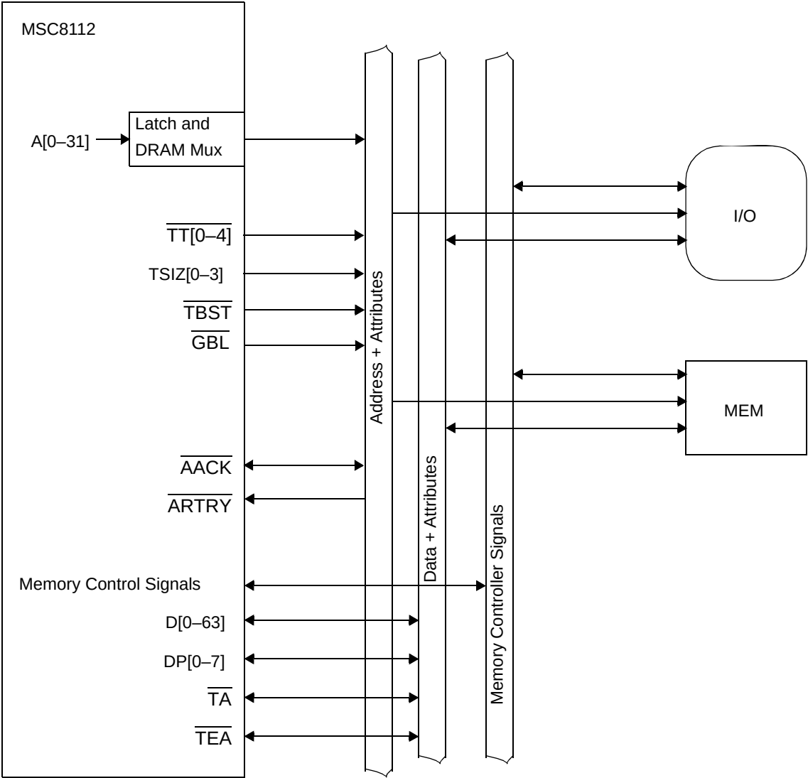
Figure 13-2. Single-MSC8112 Bus Mode
