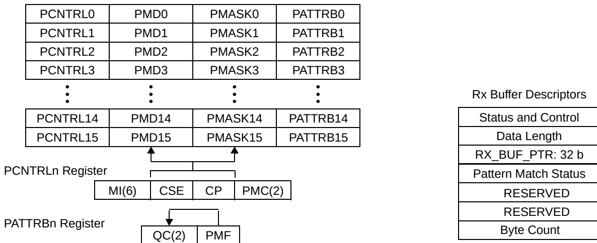
Figure 25-21. Pattern Matching Table
