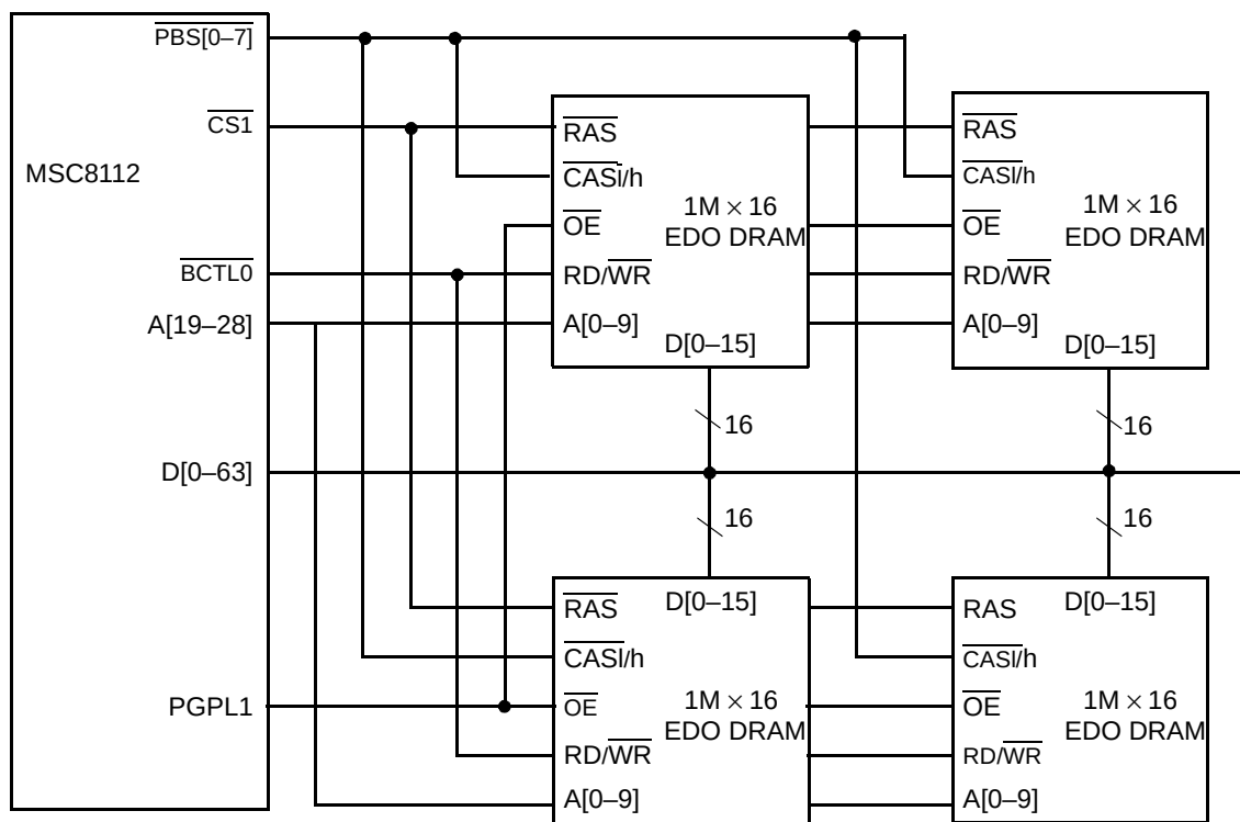
Figure 12-65. MSC8112/EDO Interface Connection to the System Bus (64-Bit Port Size)
