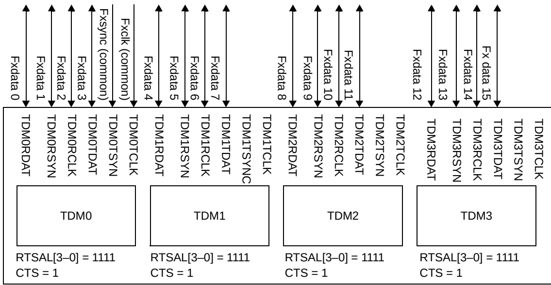
Figure 20-10. Shared Frame Sync, Clock, and Data Links
