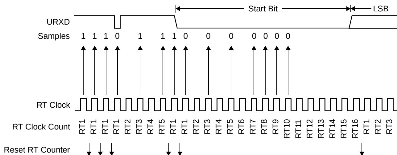
Figure 21-10. Start Bit Search Example 1
