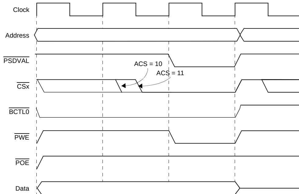
Figure 12-37. GPCM Relaxed-Timing Write (ACS = 1x, SCY = 0, CSNT = 0, TRLX = 1)
