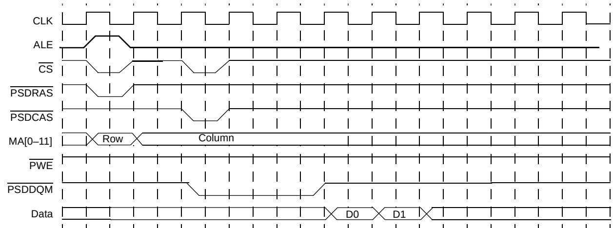
Figure 12-20. SDRAM Two-Beat Burst Read, Page Closed, CL = 3
