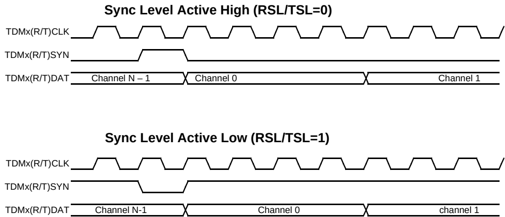
Figure 20-21. Frame Sync Polarity
