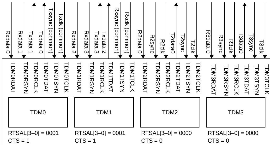
Figure 20-8. TDM Modules Model
