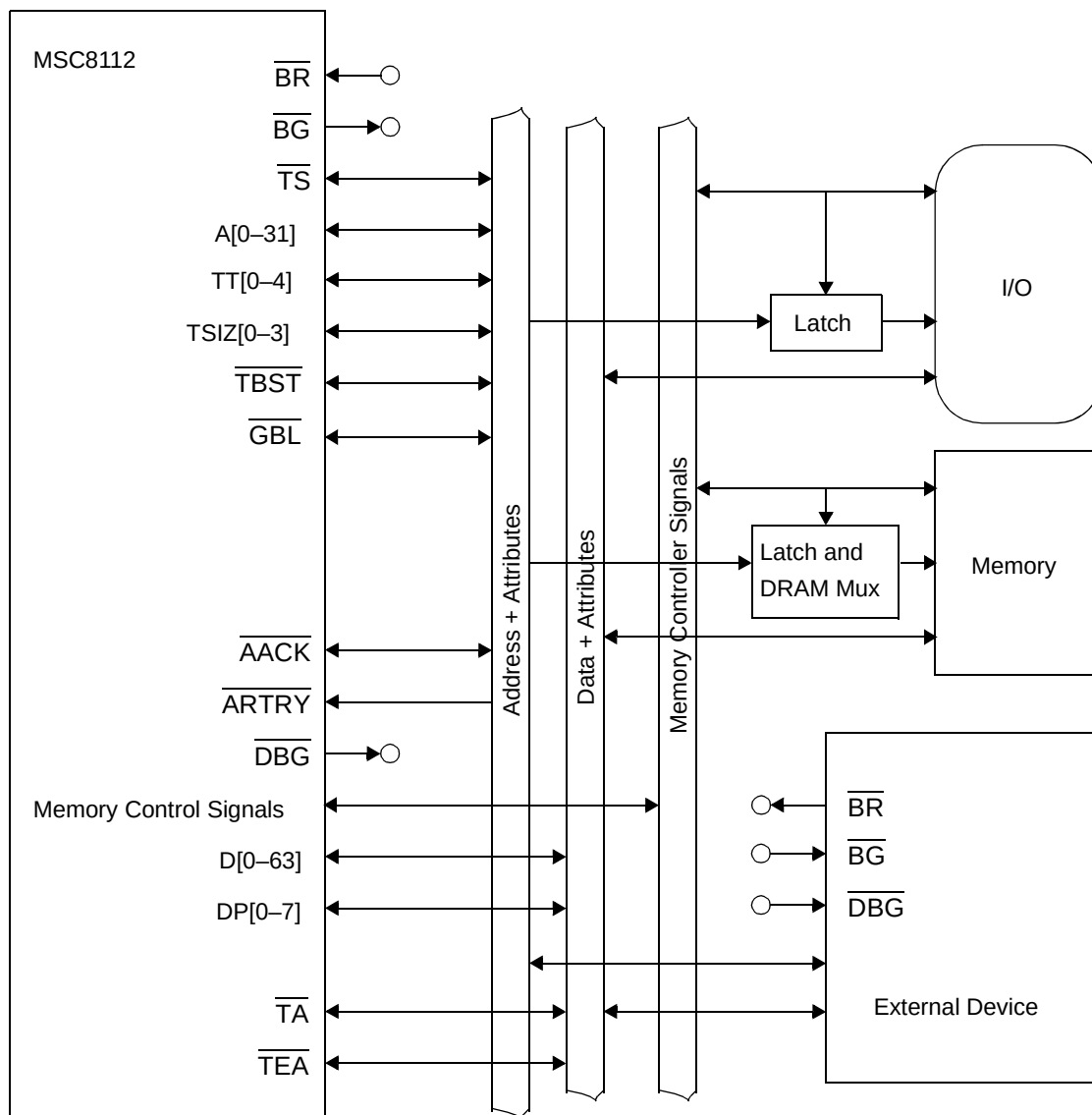
Figure 13-3. 60x-Compatible Bus Mode
