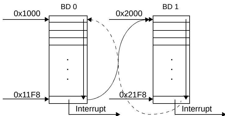
Figure 16-20. Dual Cyclic Buffers
