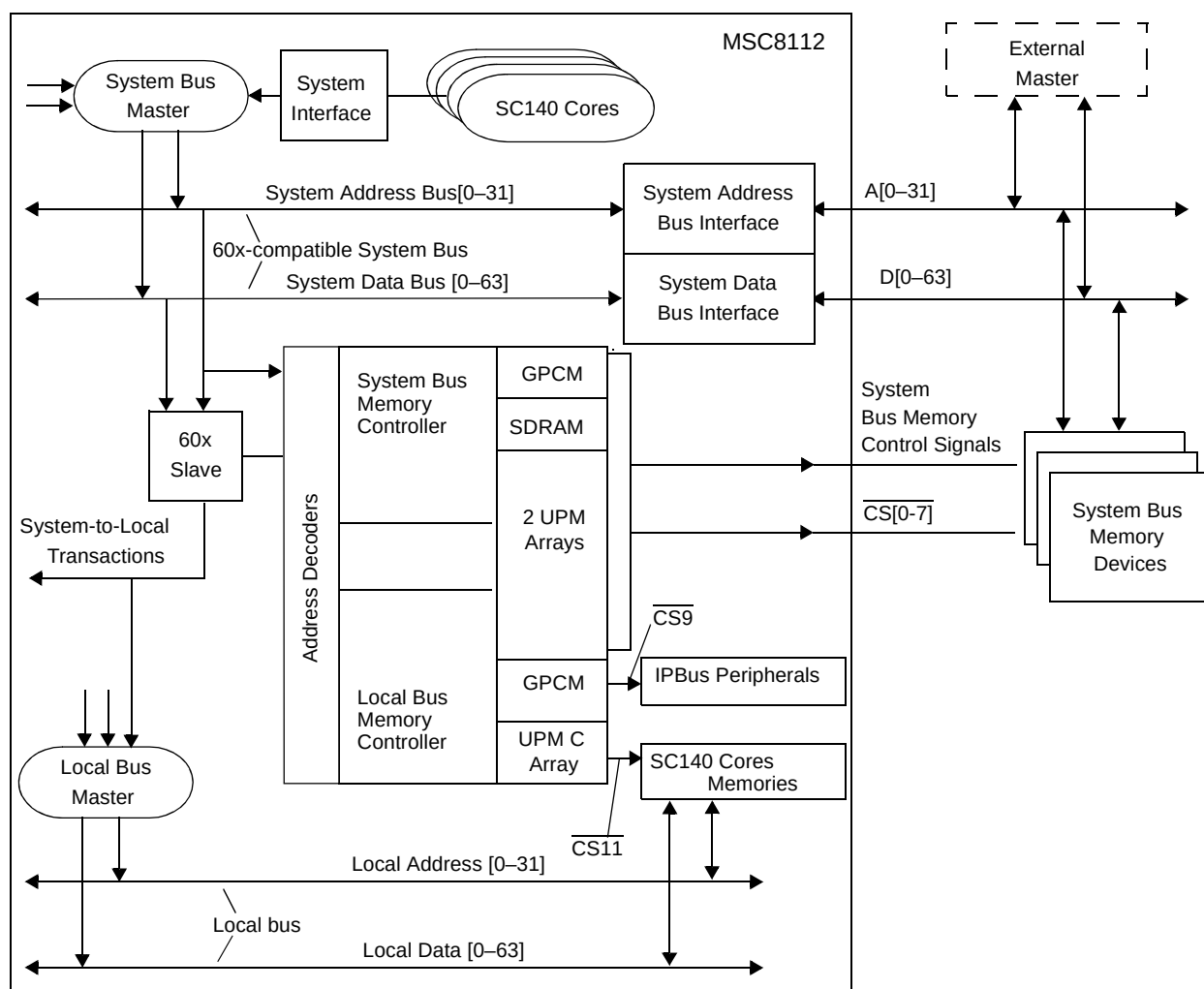
Figure 12-1. MSC8112 Dual-Bus Architecture
