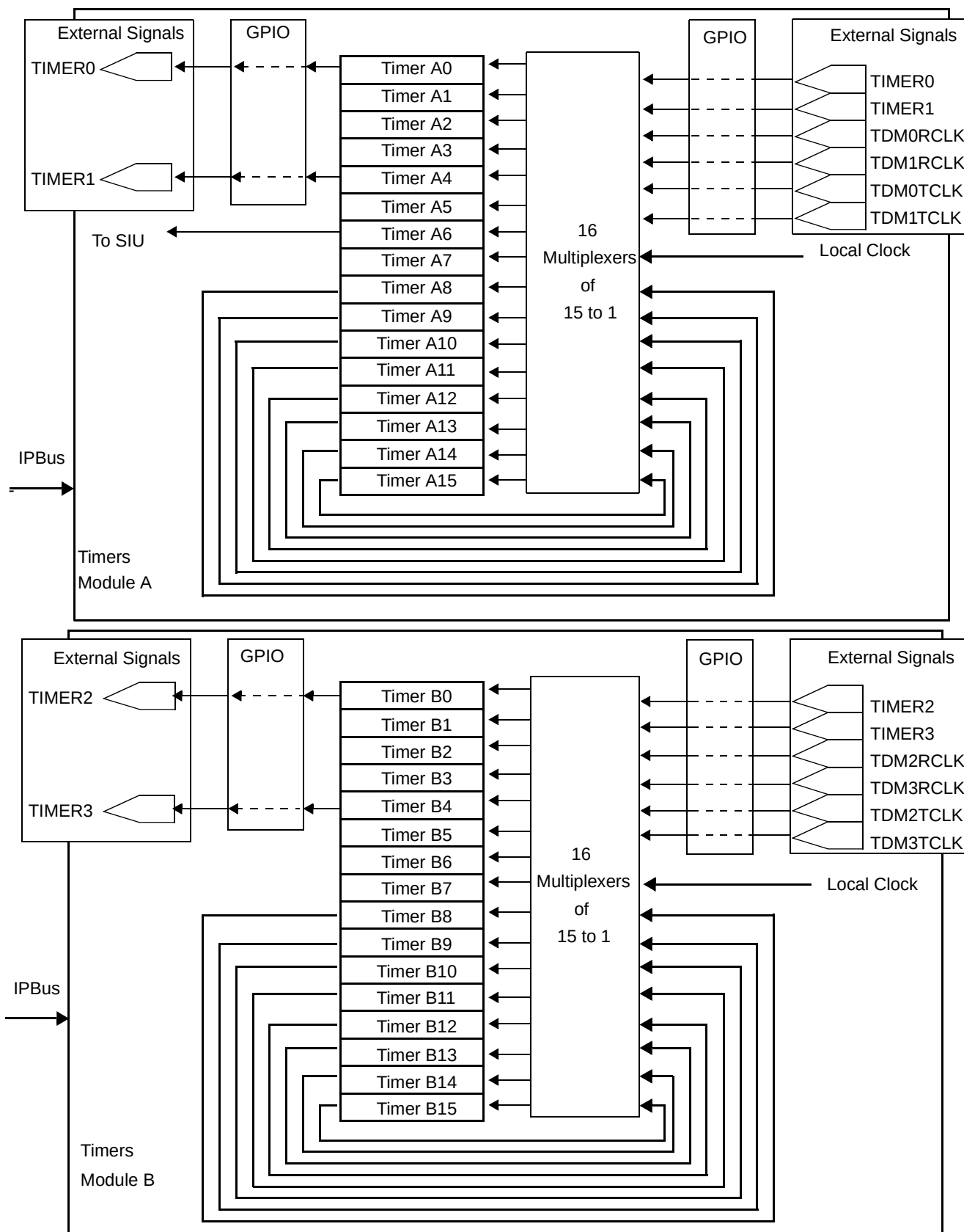
Figure 22-1. MSC8112 Timers
