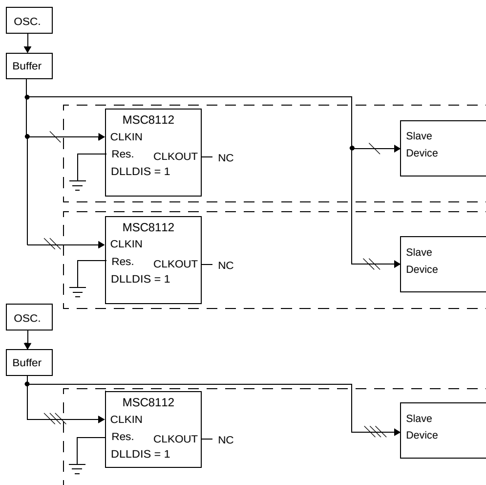
Figure 7-5. MSC8112 Clock Distribution in Single-Master Mode Using CLKIN
