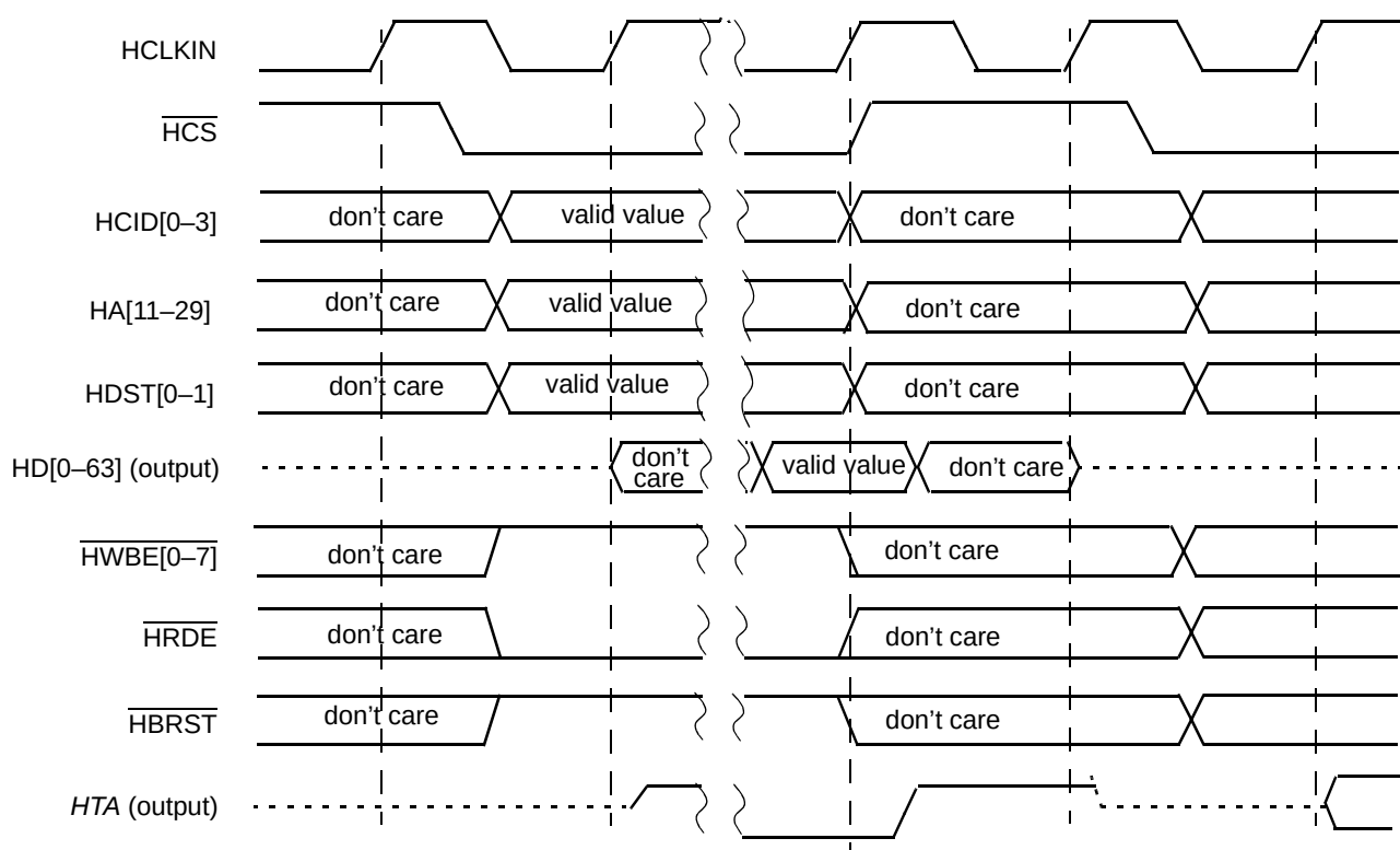
Figure 14-13. Synchronous Single Read Using Dual Strobe Mode
