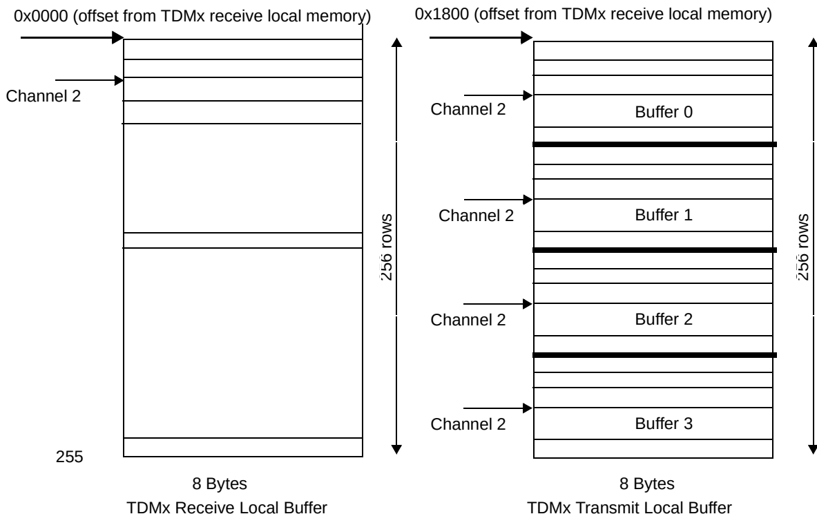
Figure 20-15. TDM Local Buffer (Receive and Transmit)
