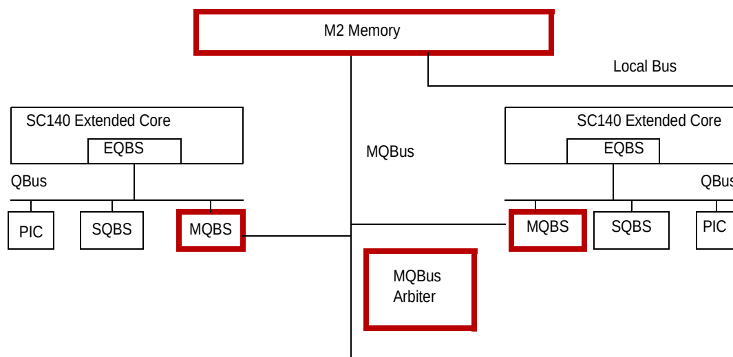
Figure 10-1. M2 Memory and MQBus System
