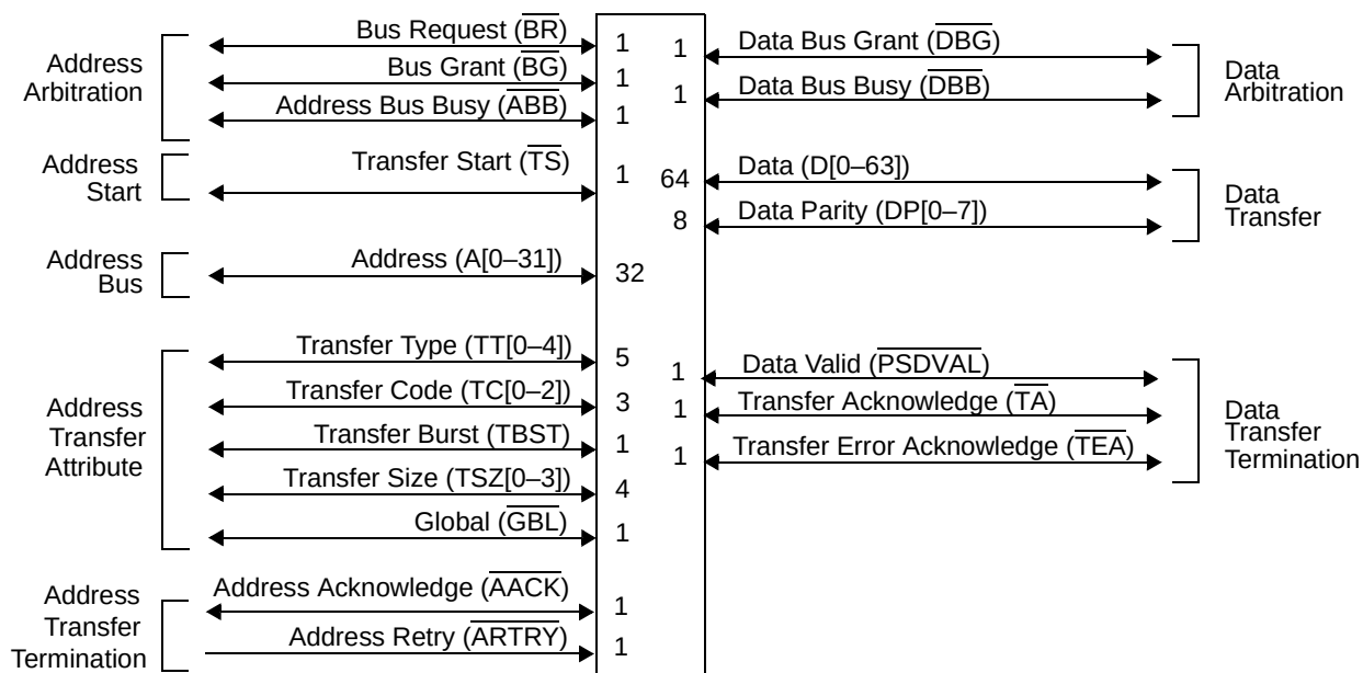
Figure 13-1. MSC8112 System Bus Groupings
