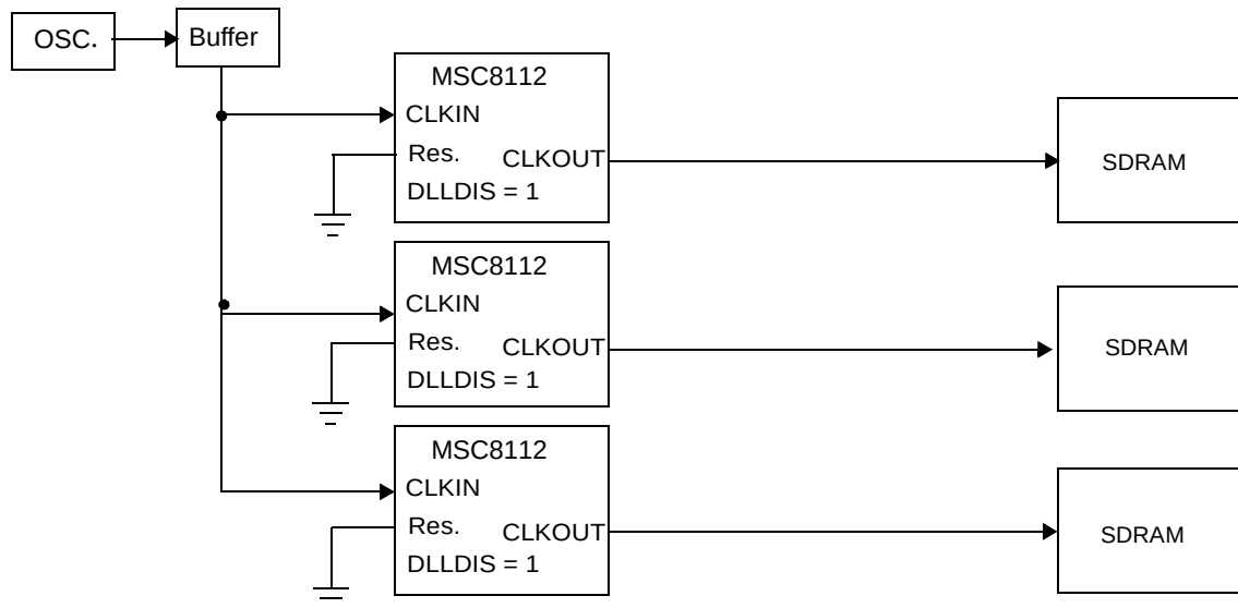
Figure 7-4. MSC8112 Clock Distribution And Synchronization In Single-Master Mode Using CLKOUT With No Zero-Delay Buffers
