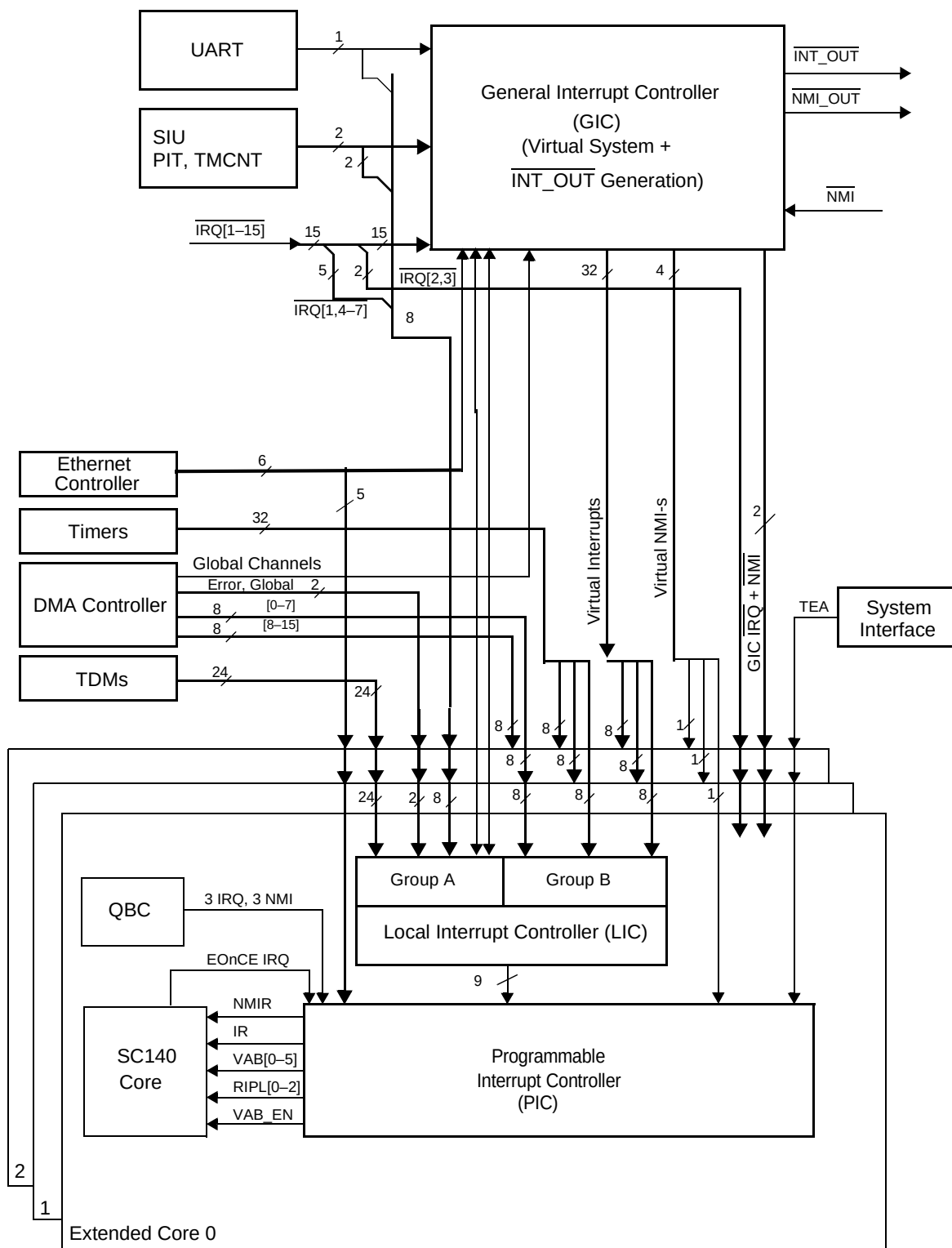
Figure 17-1. MSC8112 Interrupt Block Diagram
