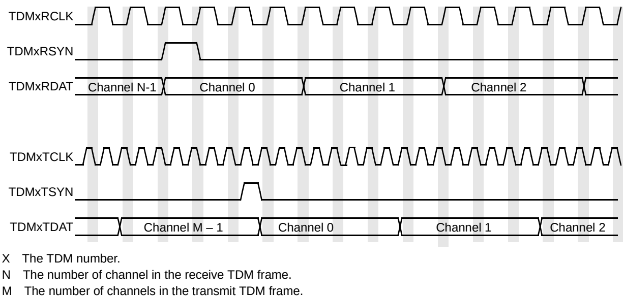
Figure 20-12. Receive and Transmit Totally Independent
