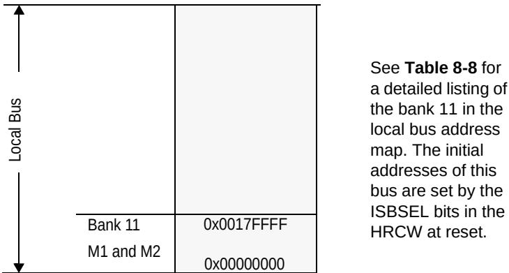
Figure 8-4. TDM View Memory Map
