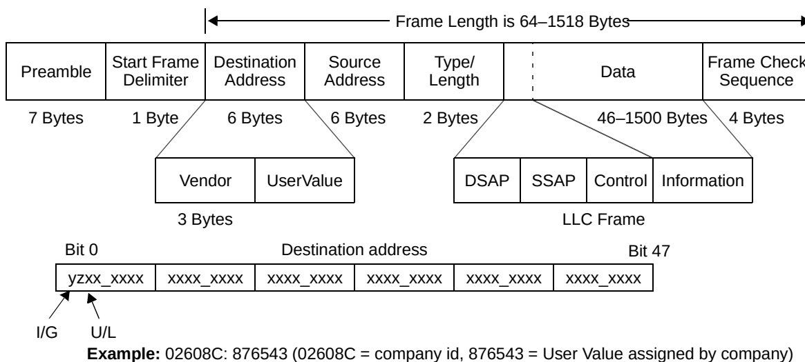
Figure 25-3. Ethernet/ IEEE Std. 802.3 Frame Structure With Details
