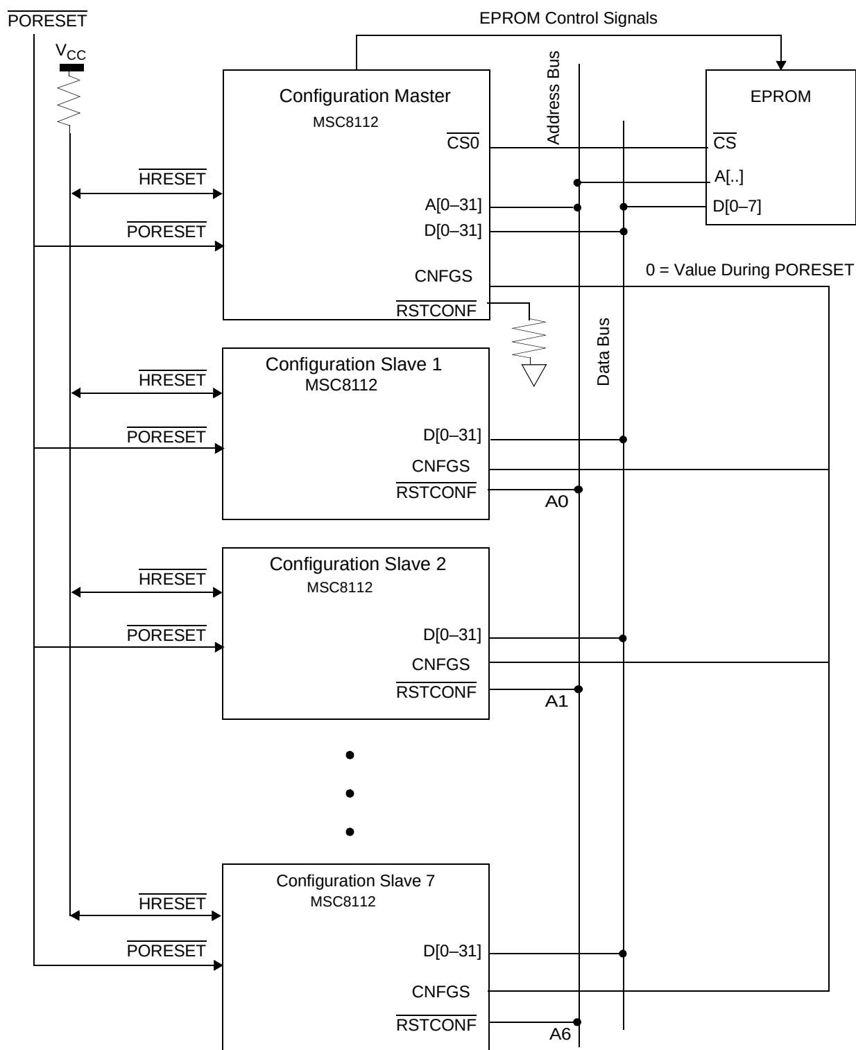
Figure 5-6. Configuring Multiple MSC8112 Devices
