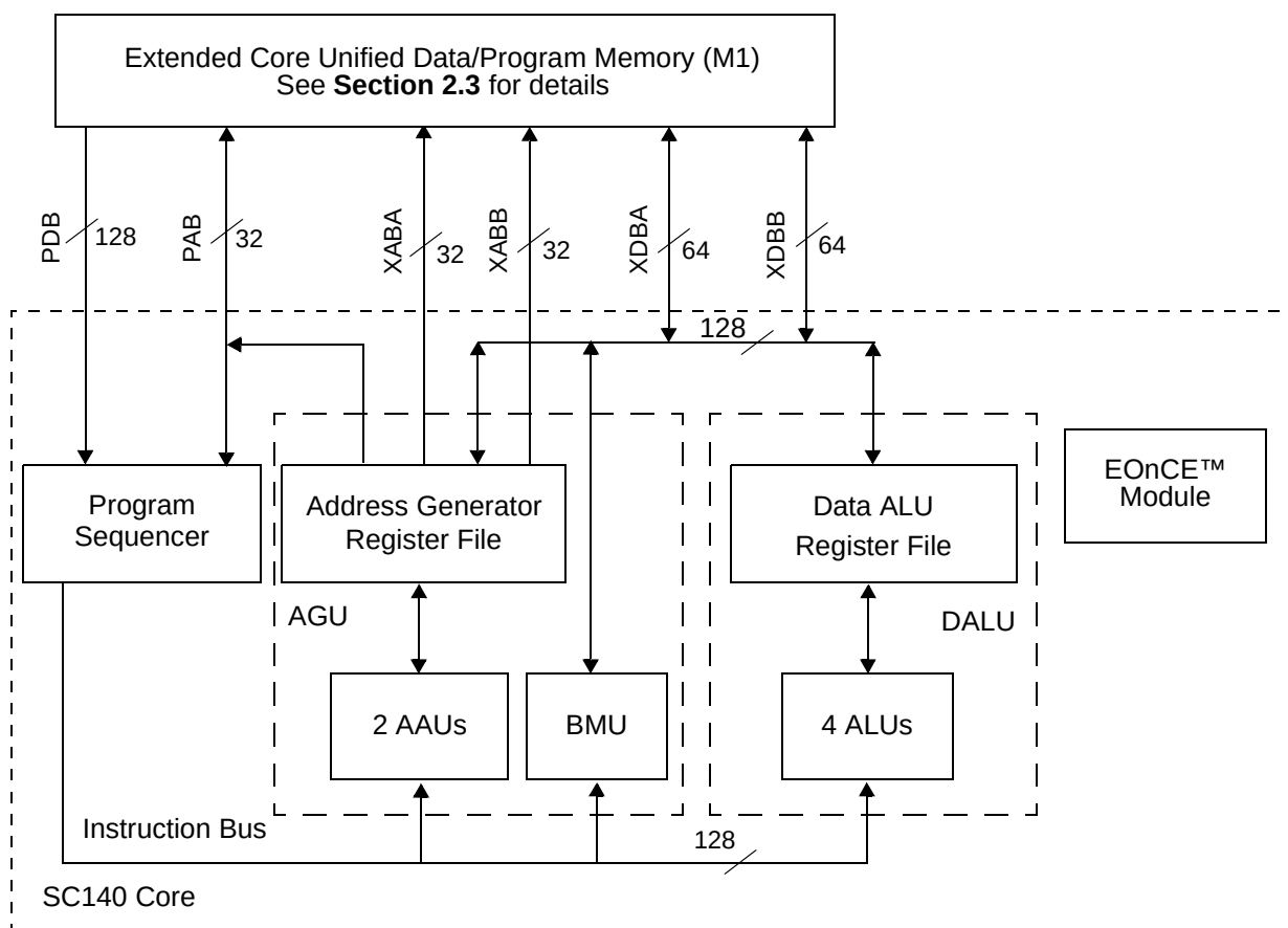
Figure 2-1. Block Diagram of the SC140 Core in the MSC8112
