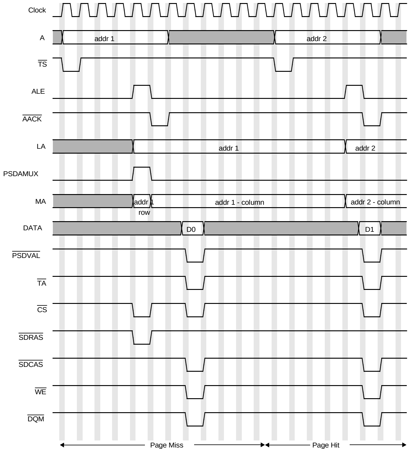
Figure 12-75. 60x-Compatible Mode SDRAM Access
