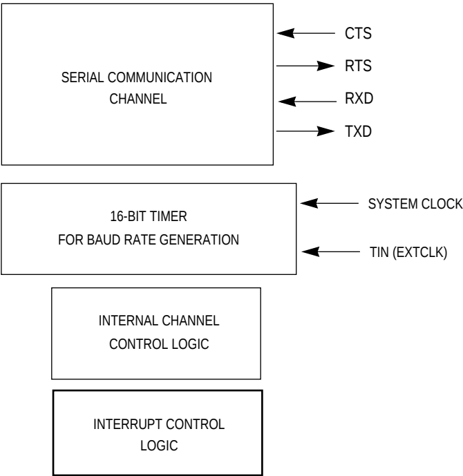
Figure 8-1. UART Block Diagram
