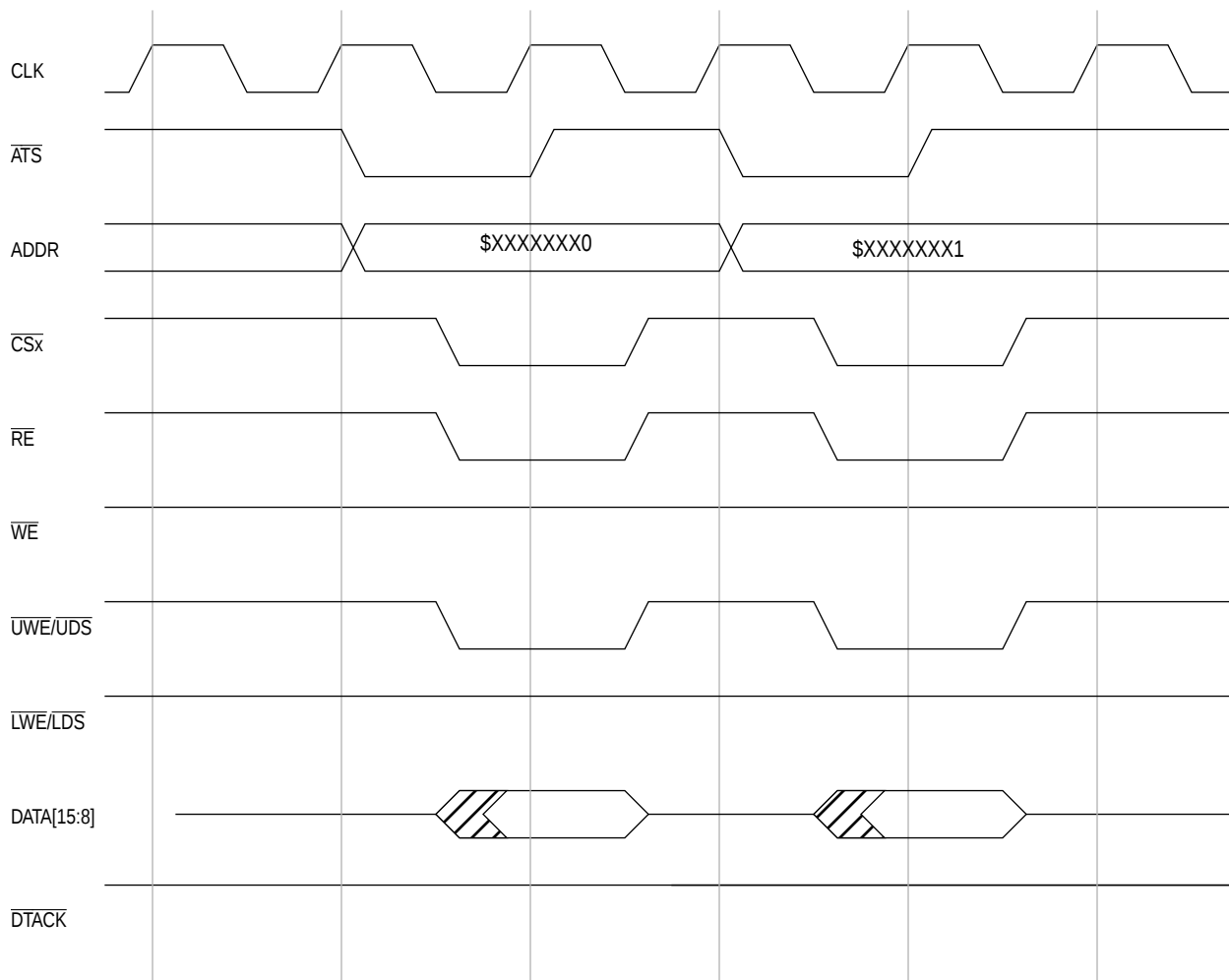
Figure 6-15. Read: Word, Byte Port, Internal Termination, Burst-Inhibited, “0” Wait State
