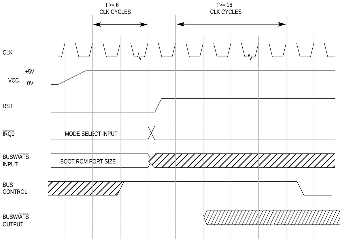
Figure 6-31. Reset Operation
