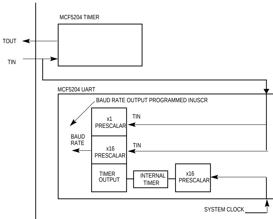
Figure 8-3. Baud Generator Diagram
