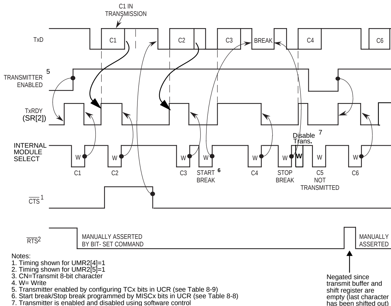
Figure 8-5. Transmitter Timing Diagram
