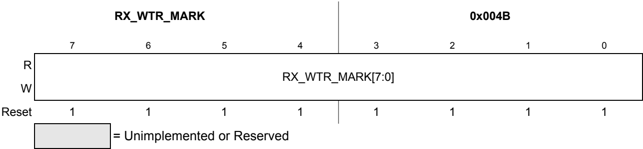
Figure 6-18. Receiver Byte Count Watermark Threshold
