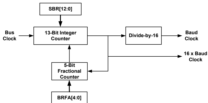
Figure 13-1. SCI Baud Rate Generator
