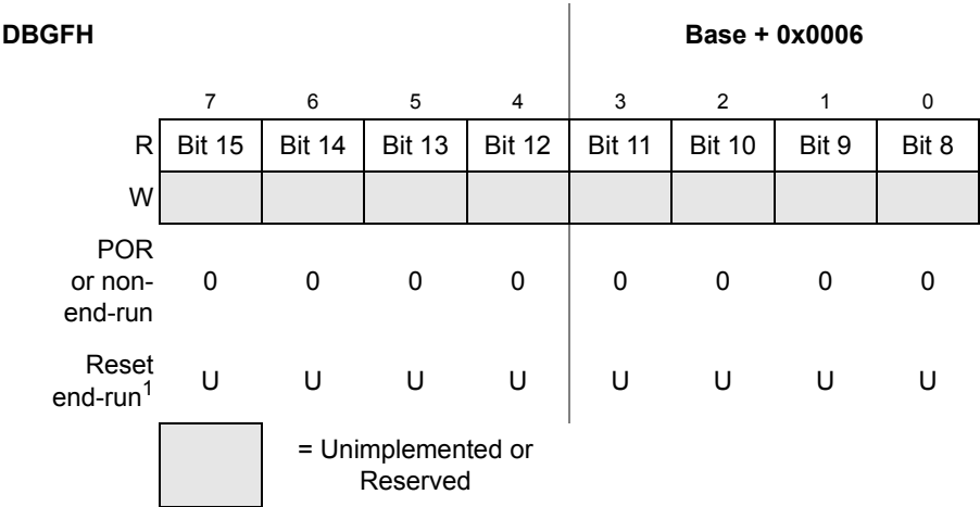
Figure 17-19. Debug FIFO High Register (DBGFH)
