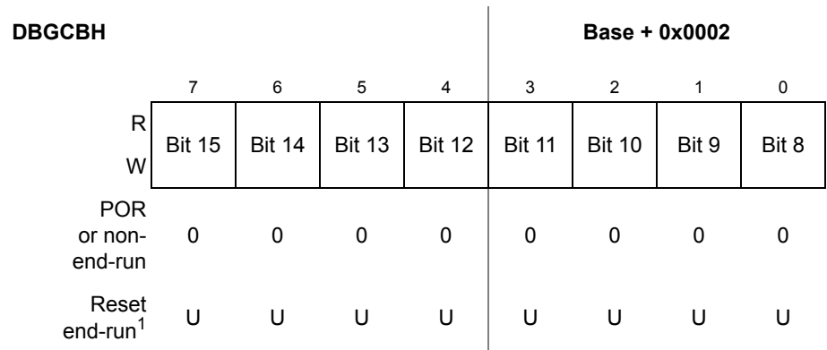
Figure 17-15. Debug Comparator B High Register (DBGCBH)
