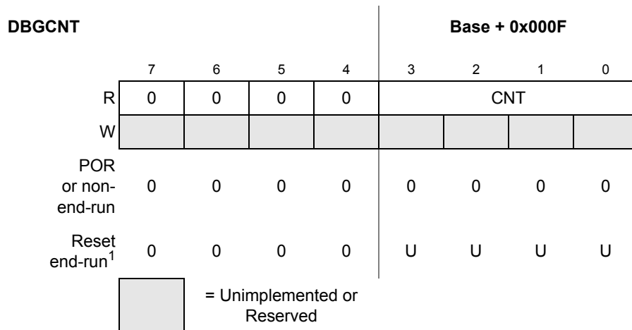
Figure 17-28. Debug Count Status Register (DBGCNT)
