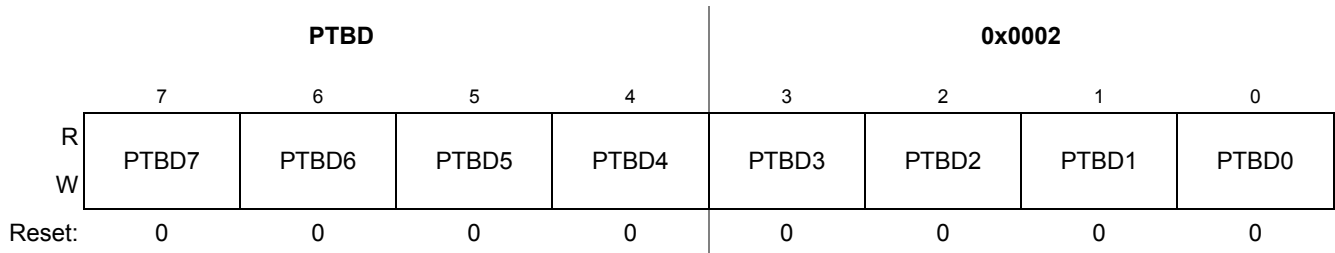
Figure 9-7. Port B Data Register (PTBD)
