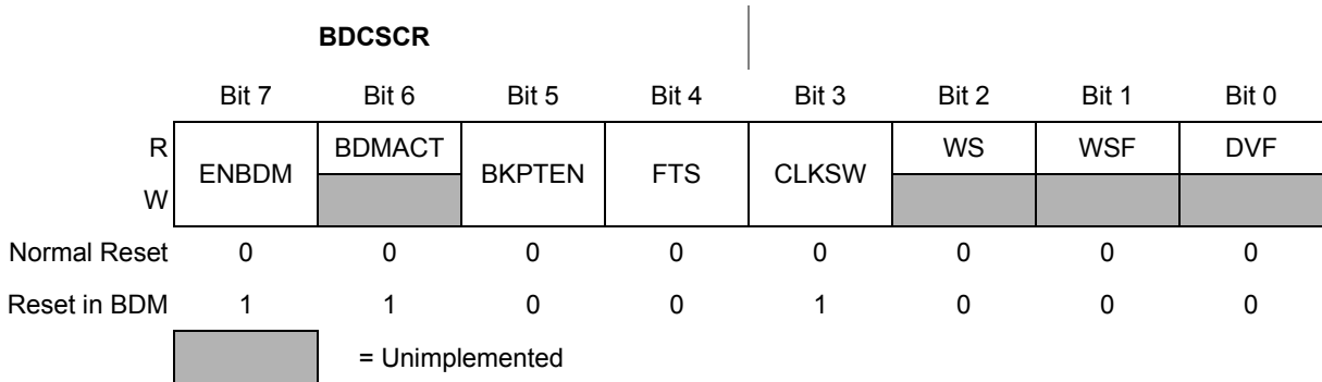
Figure 17-11. BDC Status and Control Register (BDCSCR)
