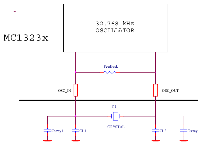
Figure 3-7. MC1323x 32.768 kHz Oscillator Model
