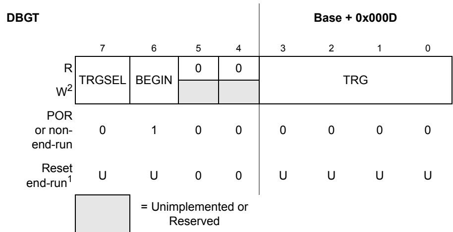
Figure 17-26. Debug Trigger Register (DBGT)
