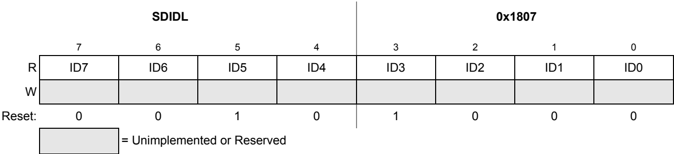
Figure 5-10. System Device Identification Register — Low (SDIDL) Table 5-14. SDIDL Register Field Descriptions
