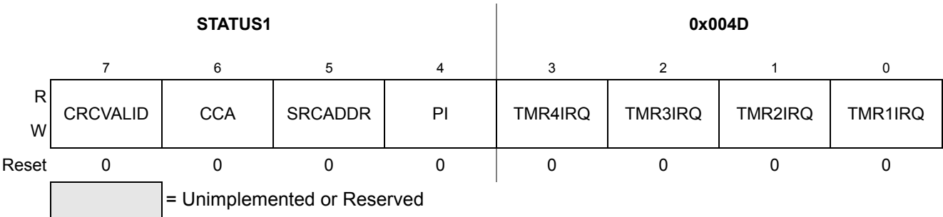
Figure 6-20. Status Register 1
