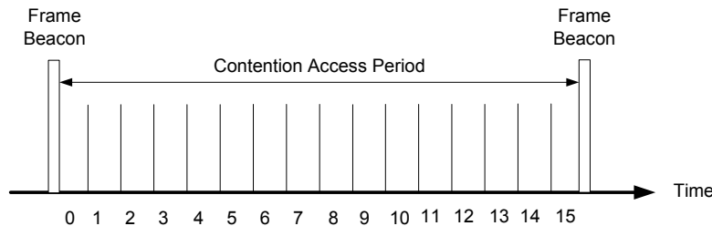
Figure A-1. Simple Superframe Structure
