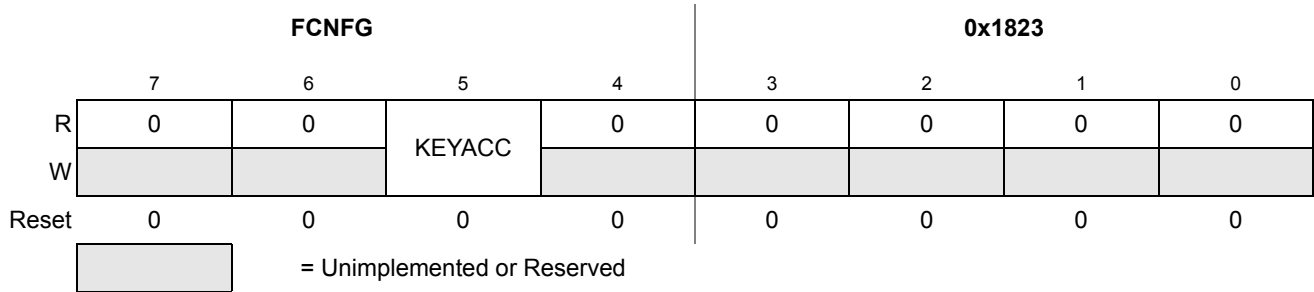
Figure 4-8. FLASH Configuration Register (FCNFG)
