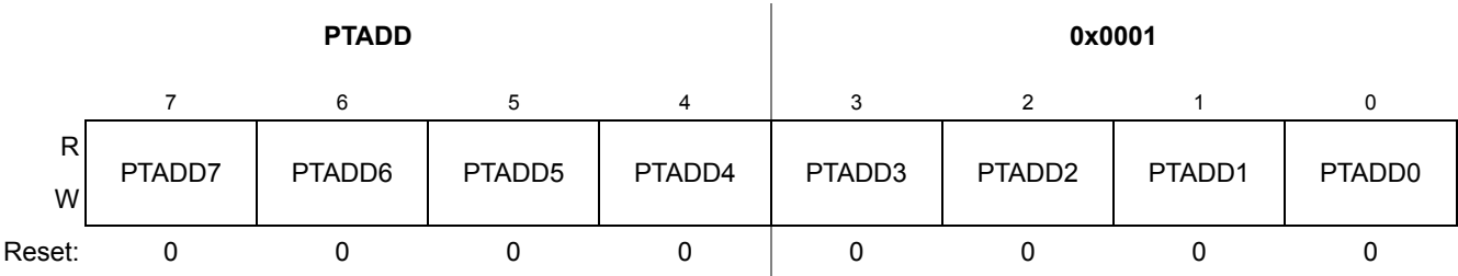
Figure 9-3. Port A Data Direction Register (PTADD)
