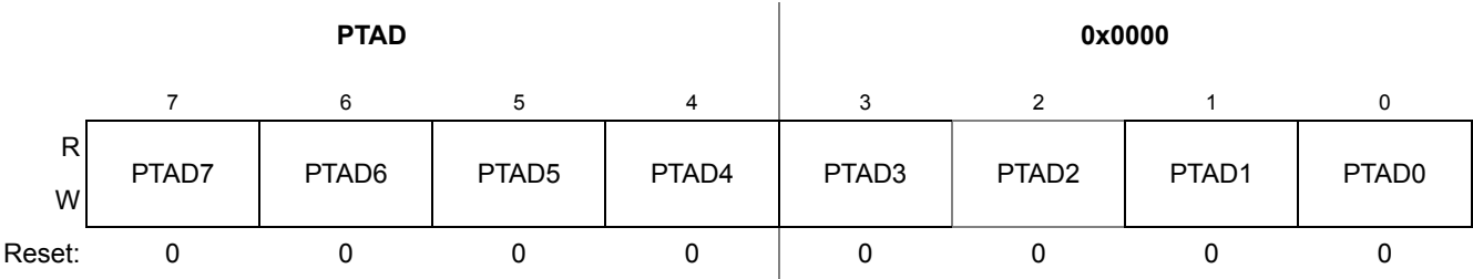
Figure 9-2. Port A Data Register (PTAD)
