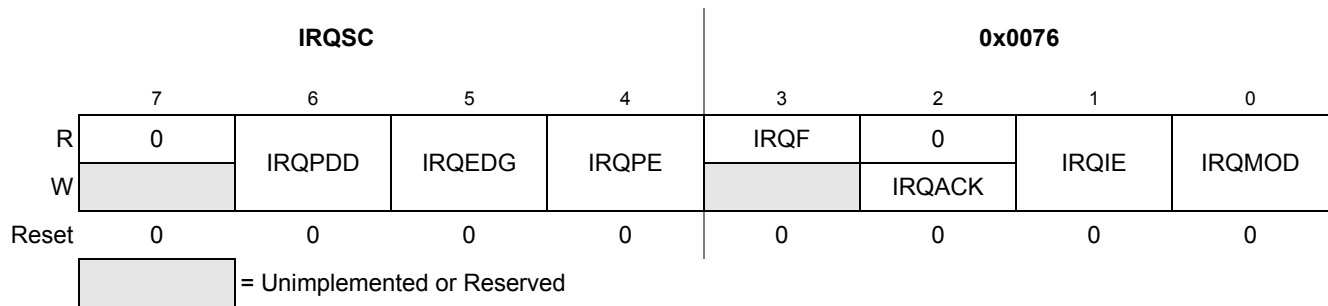
Figure 5-4. Interrupt Request Status and Control Register (IRQSC)
