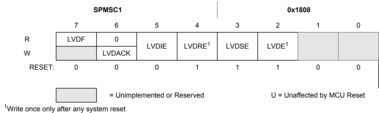
Figure 5-11. System Power Management Status & Control 1 Register (SPMSC1)
