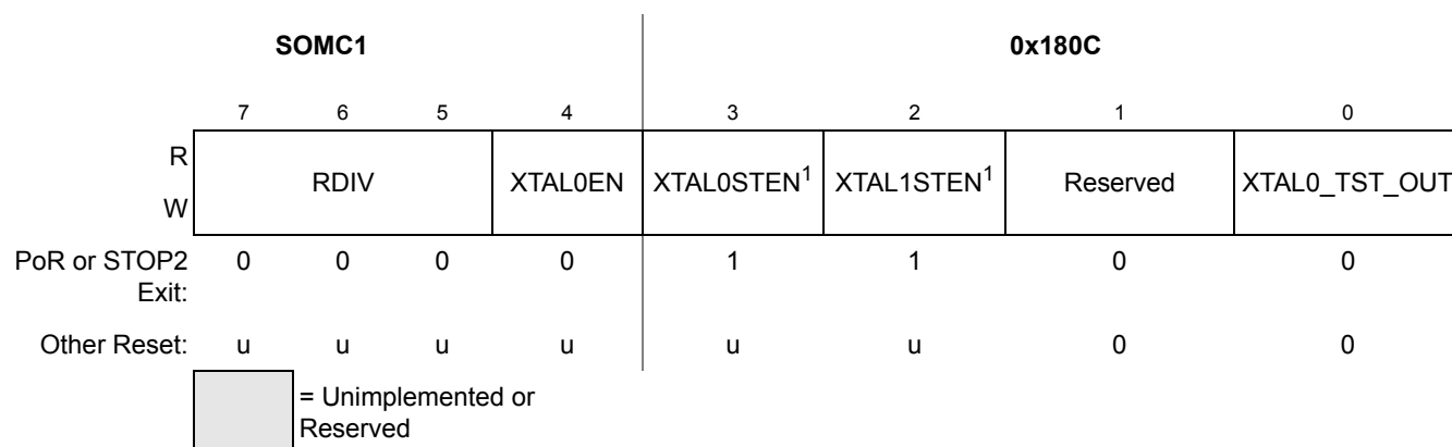
Figure 5-14. System Oscillator Management and Control Register 1 (SOMC1)
