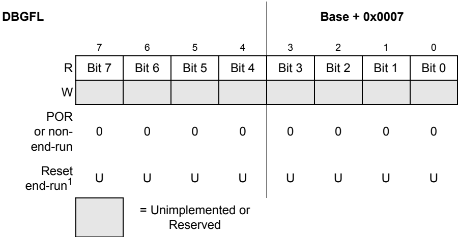
Figure 17-20. Debug FIFO Low Register (DBGFL)
