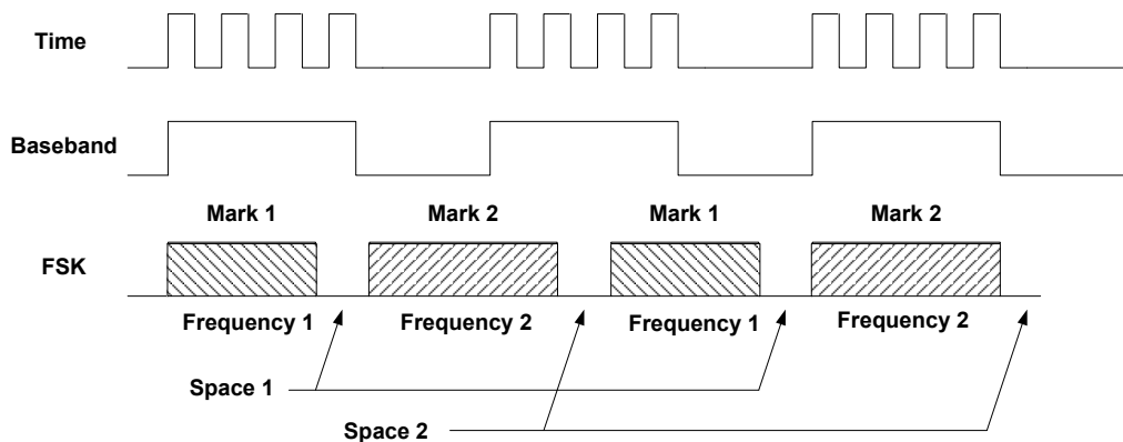
Figure 16-2. CMT Operating Modes
