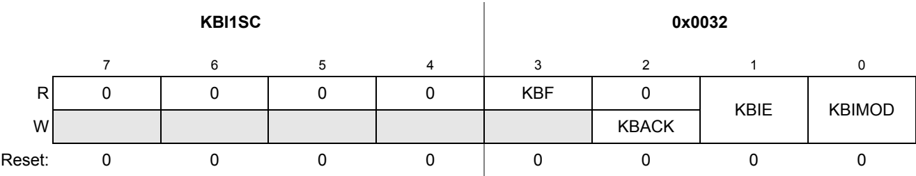
Figure 11-2. KBI1 Interrupt Status and Control Register (KBI1SC)
