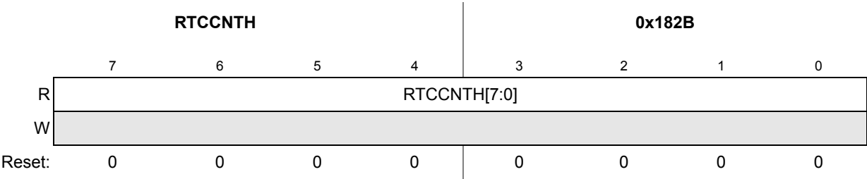
Figure 10-3. RTC Counter Register (RTCCNT)
