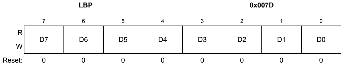
Figure 4-5. Linear Byte Post Increment Register (LBP)
