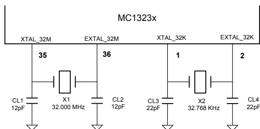
Figure 3-3. MC1323x External Clock Connections
