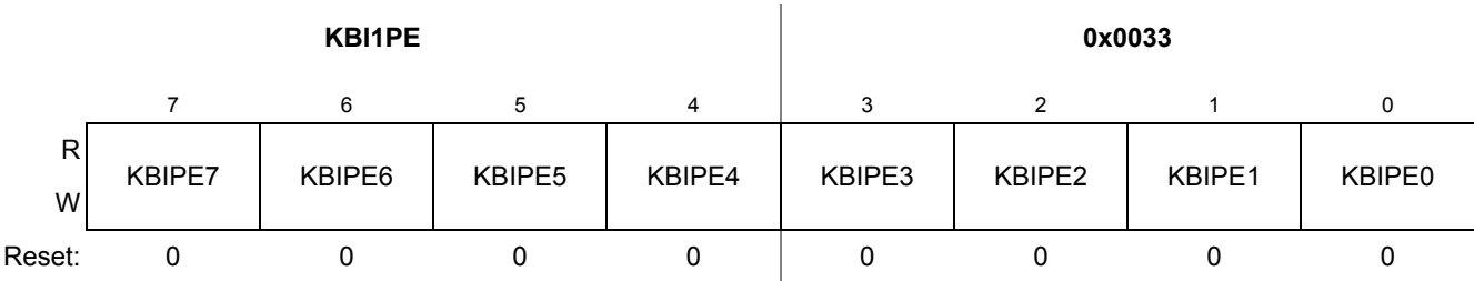
Figure 11-3. KBI1 Interrupt Pin Select Register (KBI1PE)
