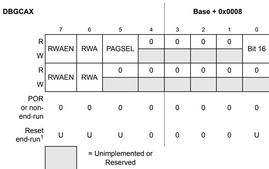
Figure 17-21. Debug Comparator A Extension Register (DBGCAx)
