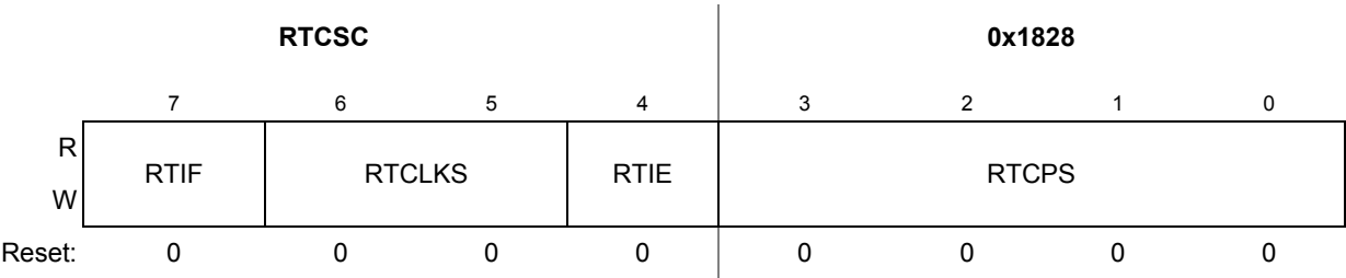
Figure 10-2. RTC Status and Control Register (RTCCSC)
