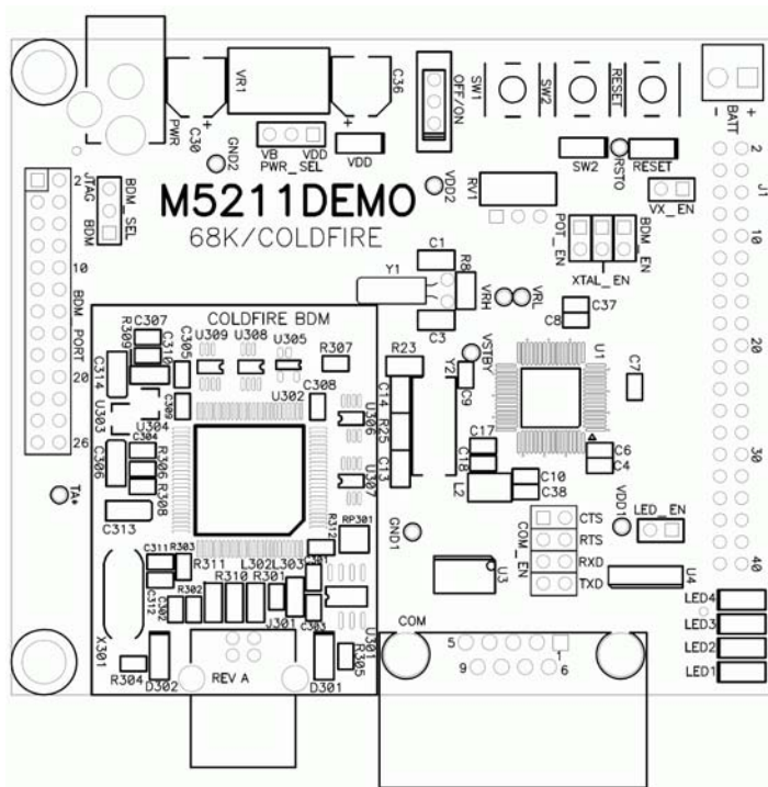
Figure 1. M5211DEMO Board
