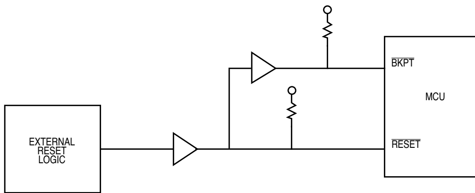
Figure 10-6 Sample BDM Enable Circuit
