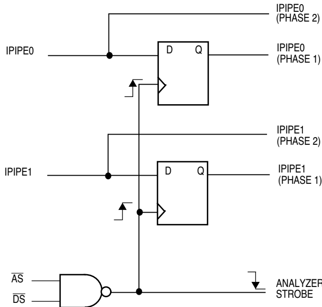
Figure 10-2 IPIPE DEMUX Logic
