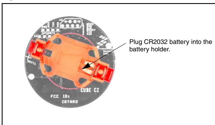
Figure 4. Battery Holder Location
