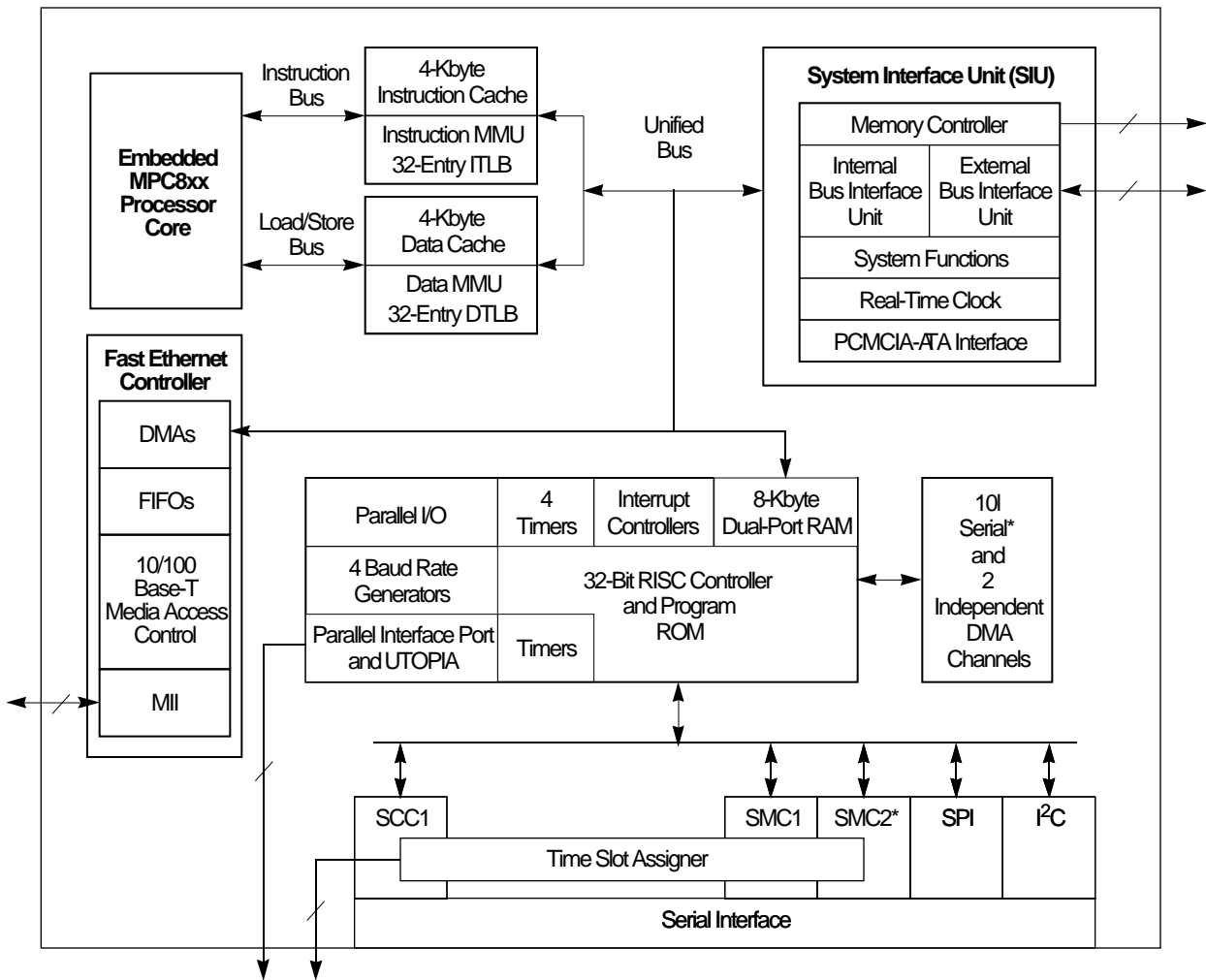
Figure 1-1. MPC857T Block Diagram
