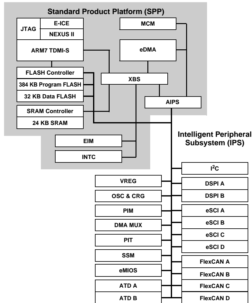
Figure 1. MAC71x4 Device Block Diagram
