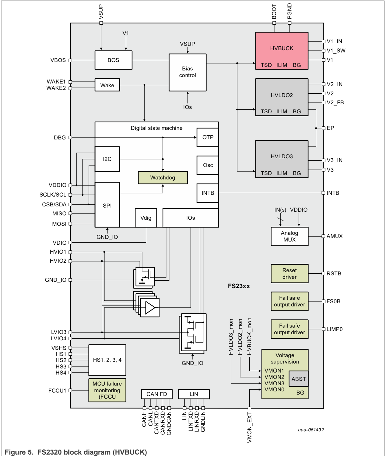
Figure 5. FS2320 block diagram (HVBUCK)
