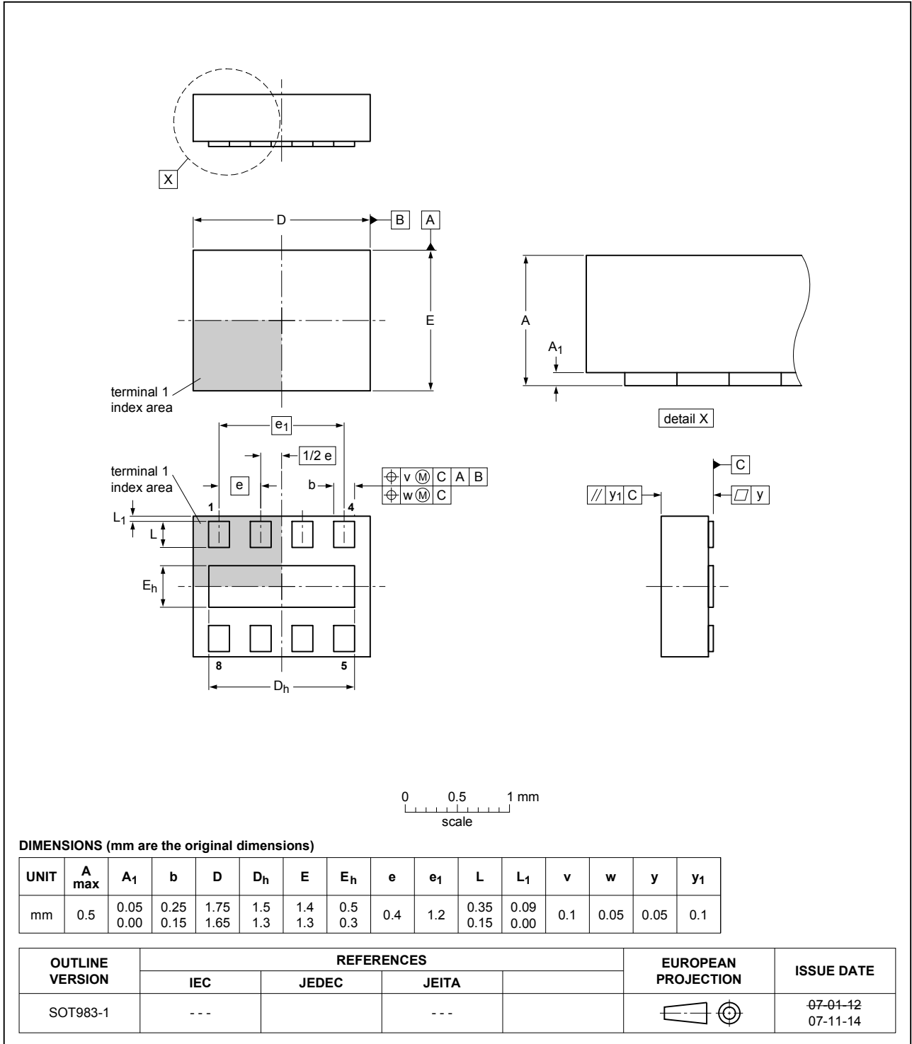
Fig. 1. Package outline DFN1714U-8 (SOT983-1)
