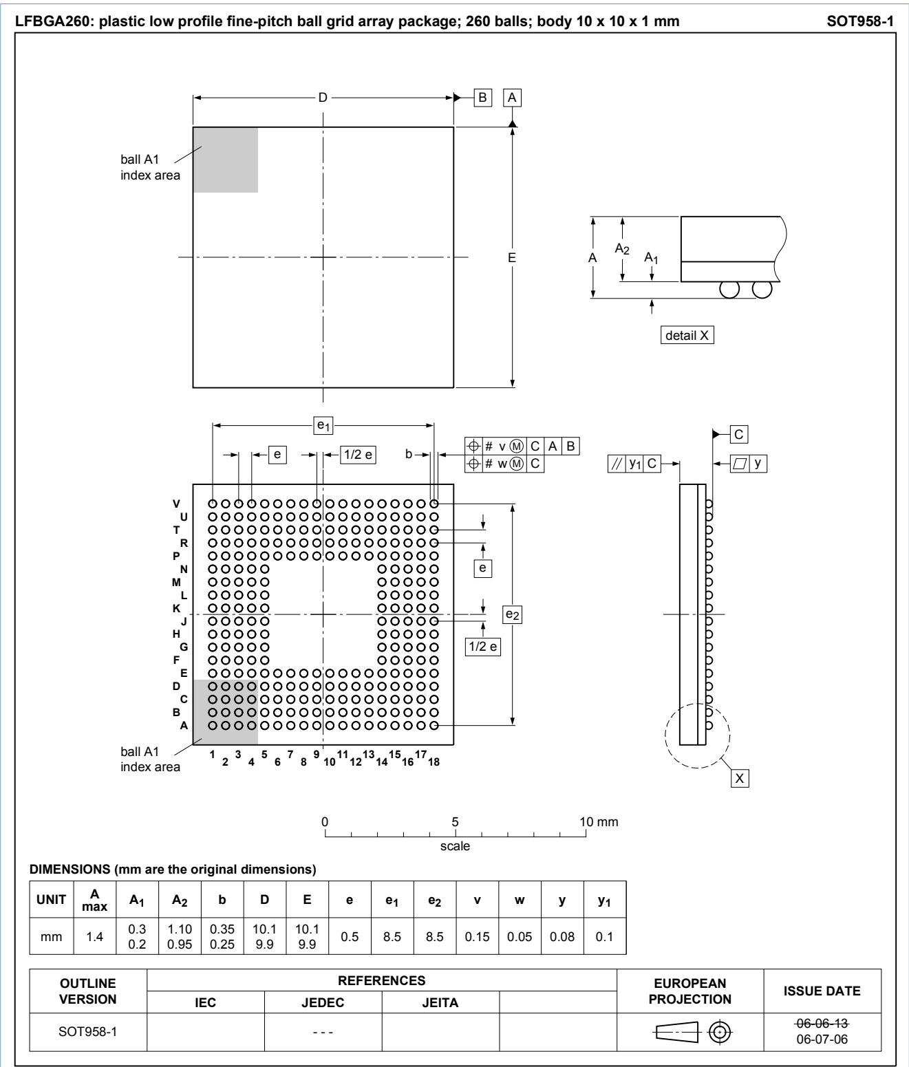
Fig. 1. Package outline LFBGA260 (SOT958-1)
