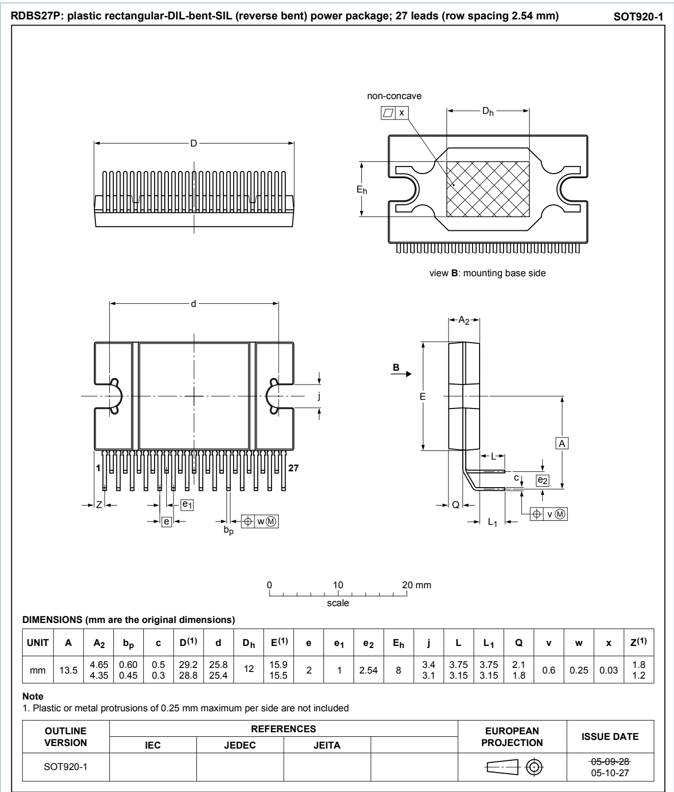
Fig. 1. Package outline RDBS27P (SOT920-1)
