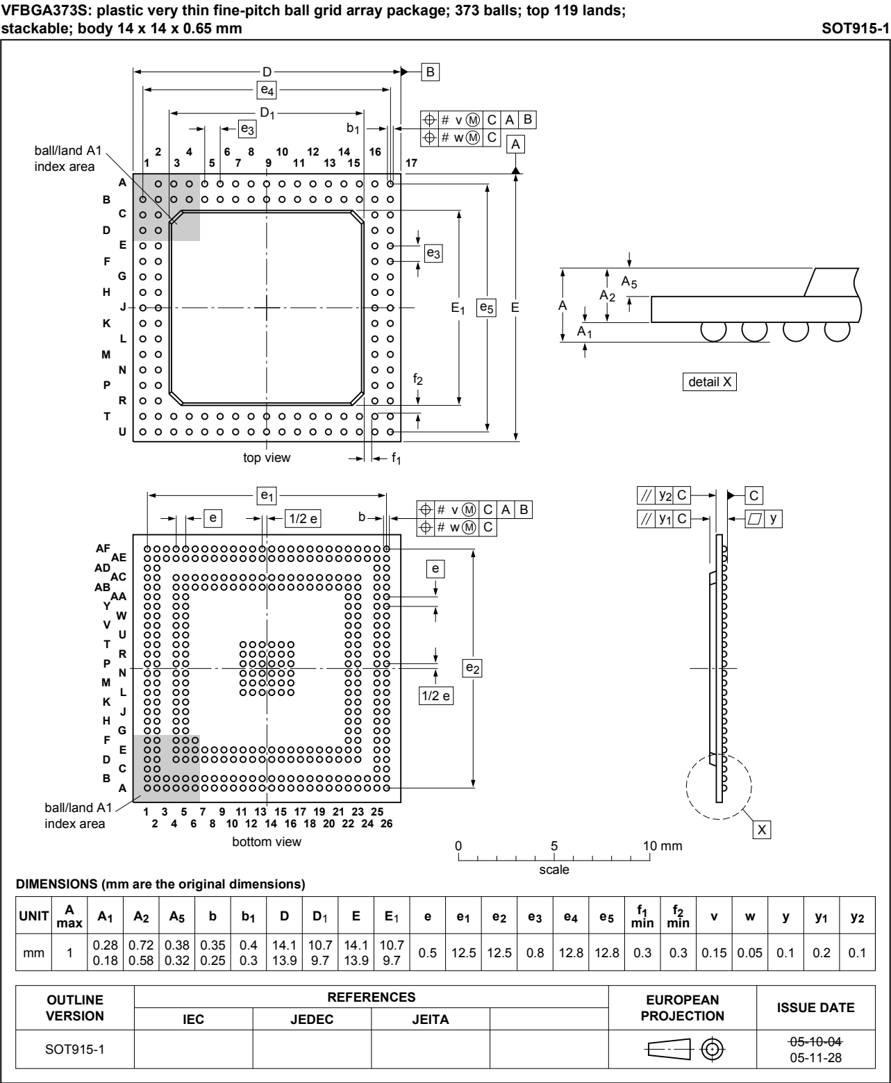
Fig. 1. Package outline VFPGA373S (SOT915-1)
