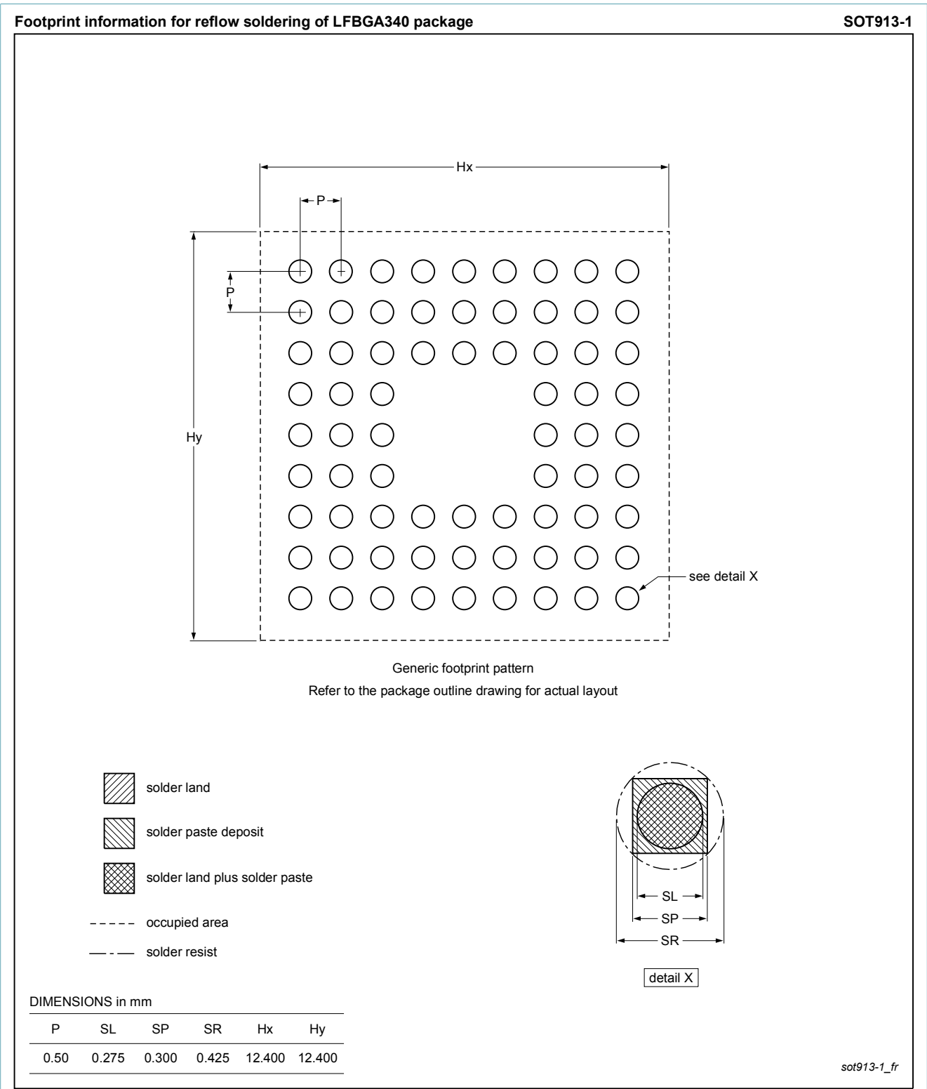
Fig. 2. Reflow soldering footprint for LFBGA340 (SOT913-1)
