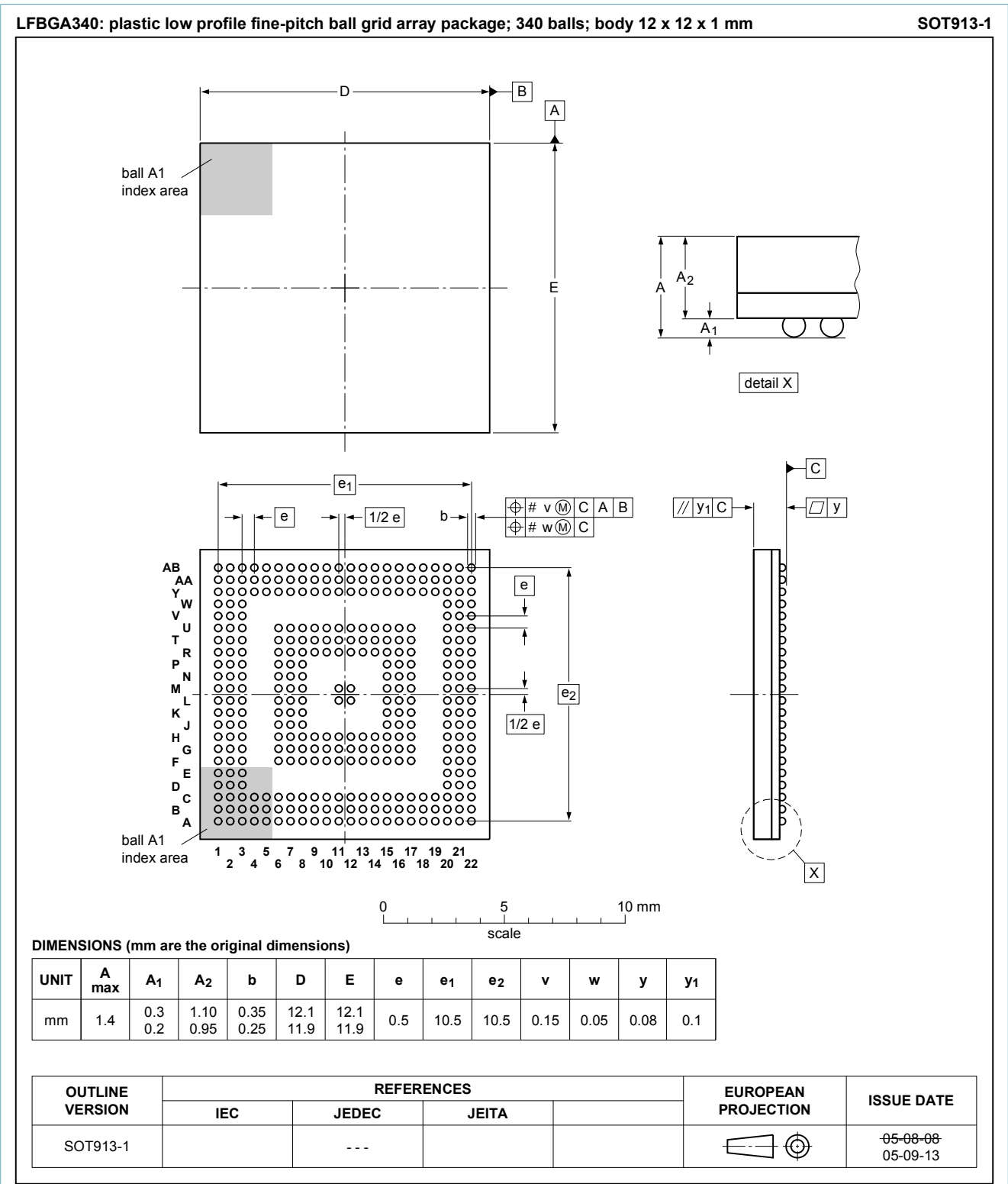
Fig. 1. Package outline LFBGA340 (SOT913-1)
