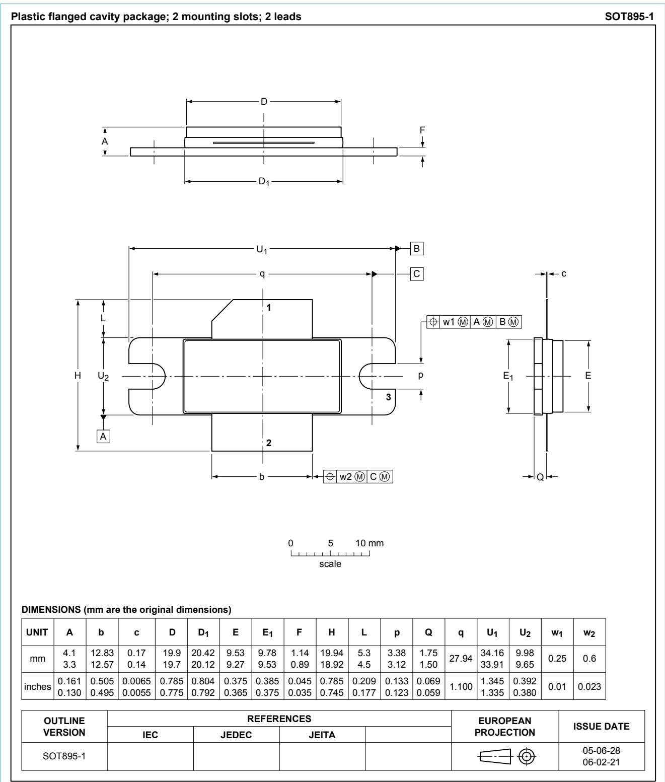
Fig. 1. Package outline DFM2 (SOT895-1)
