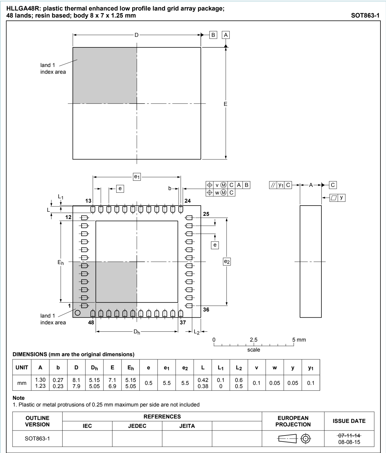
Fig. 1. Package outline HLLGA48R (SOT863-1)
