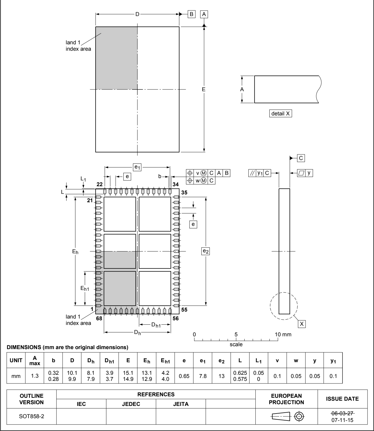
Fig. 1. Package outline HLLGA68R (SOT858-2)
