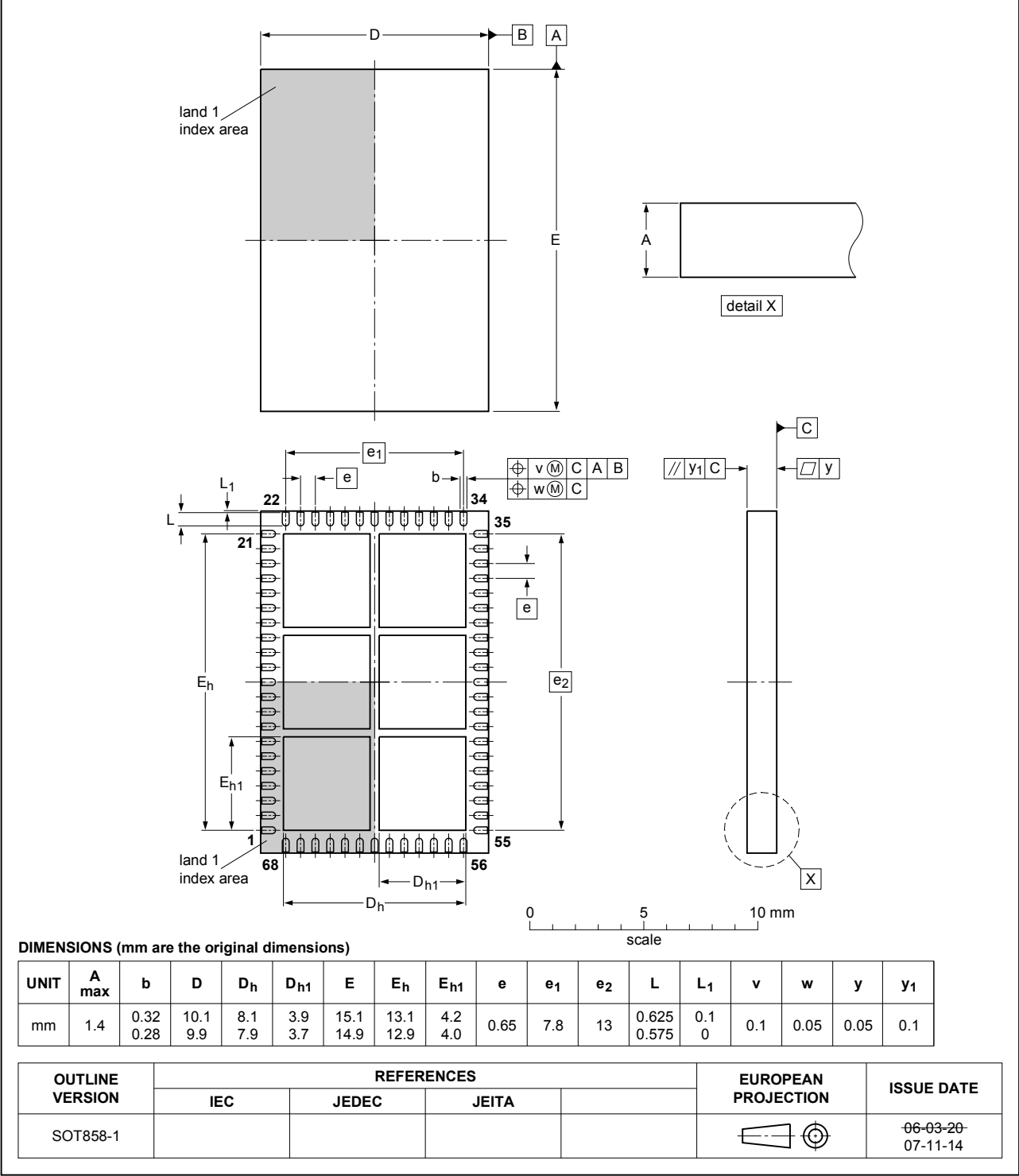
Fig. 1. Package outline HLLGA68R (SOT858-1)
