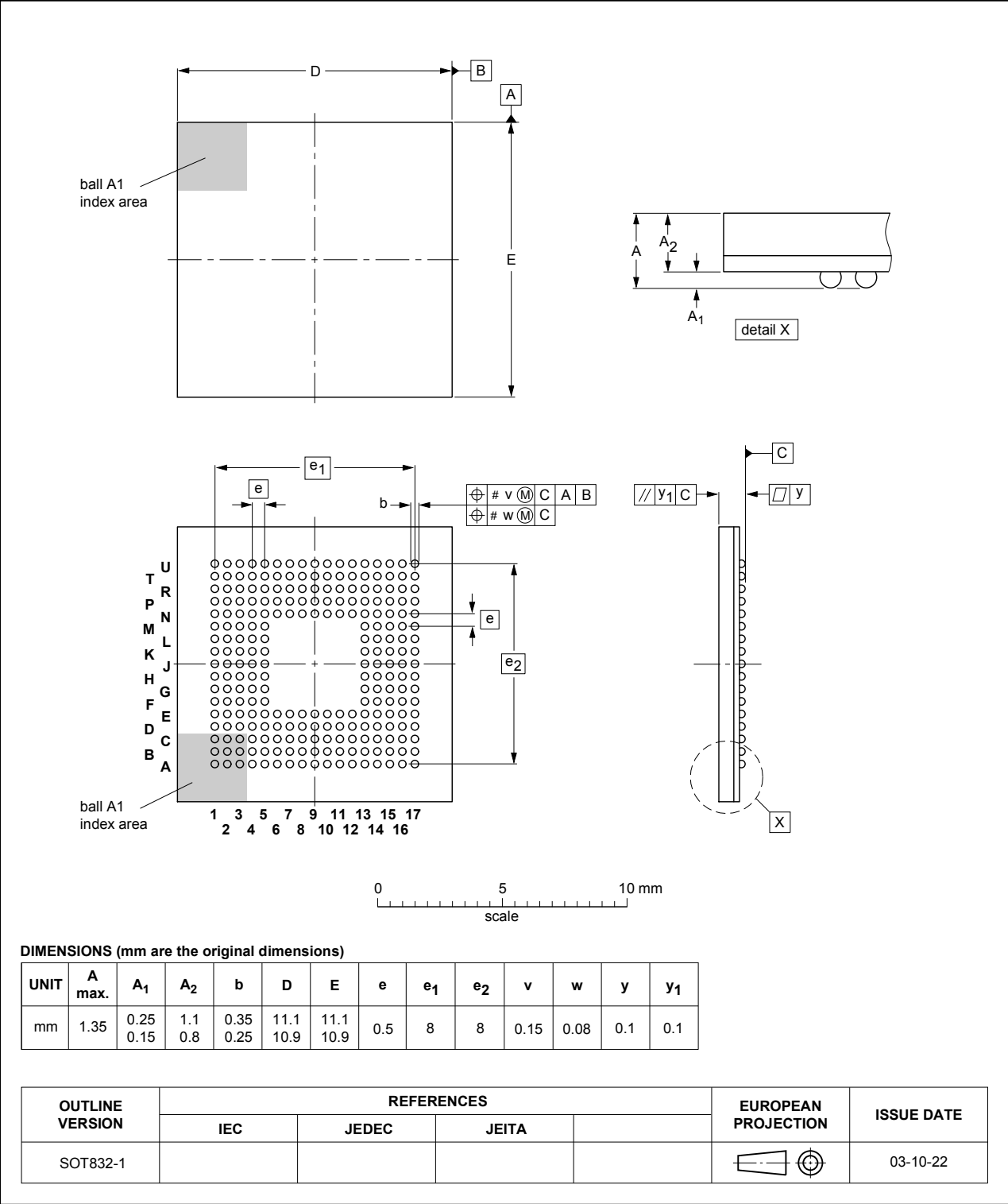
Fig. 1. Package outline LFBGA240 (SOT832-1)
