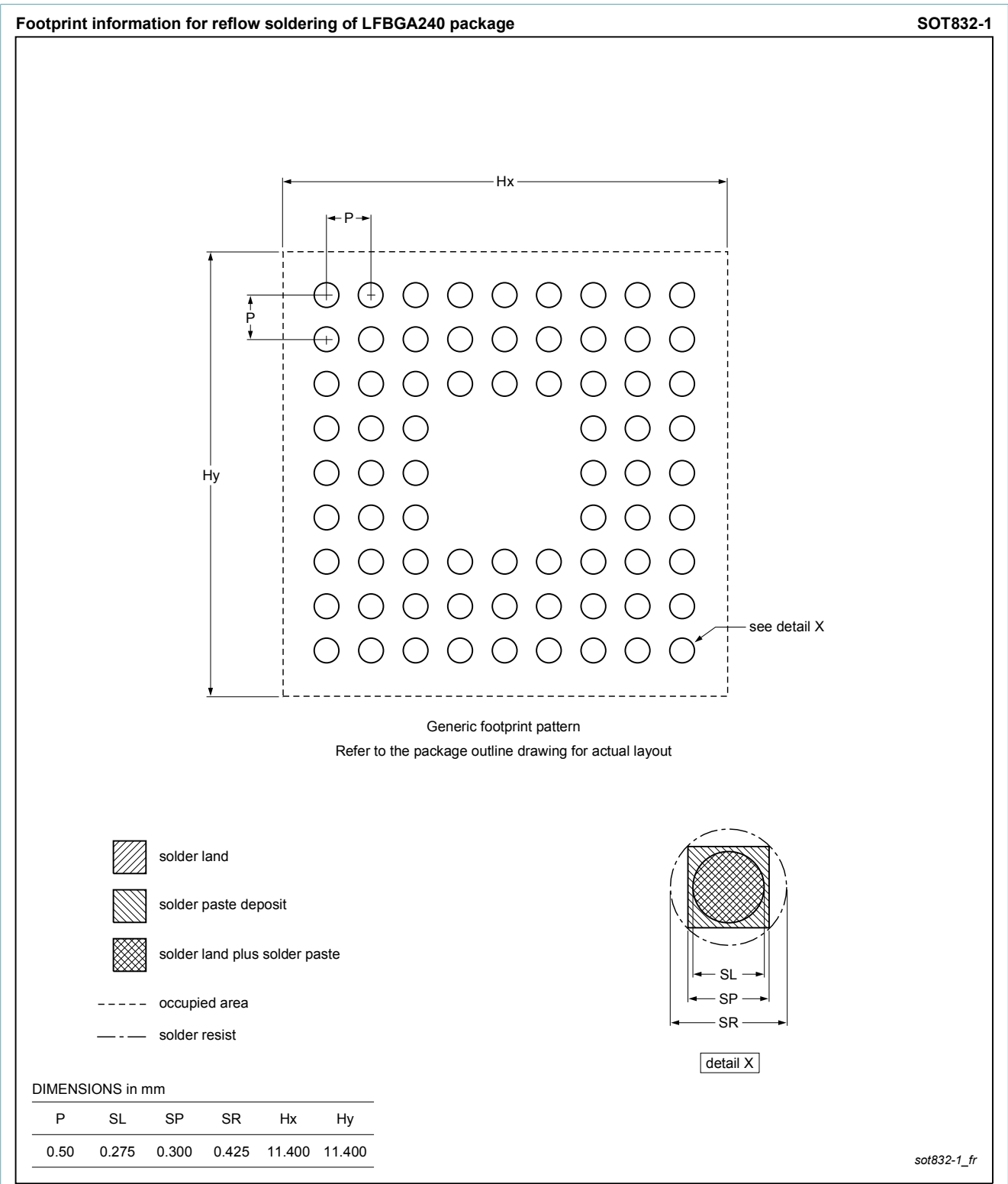
Fig. 2. Reflow soldering footprint for LFBGA240 (SOT832-1)
