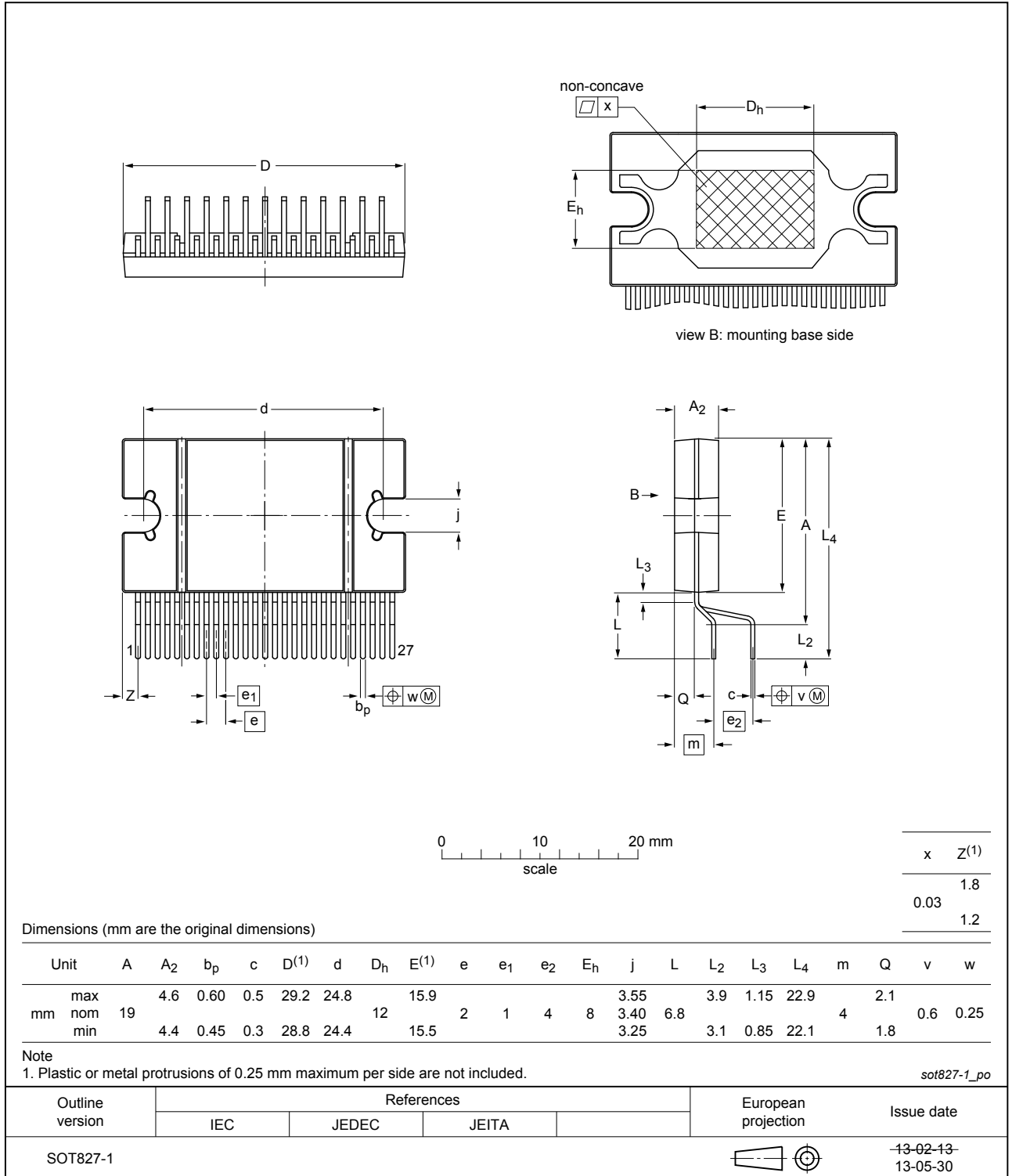
Fig. 1. Package outline DBS27P (SOT827-1)
