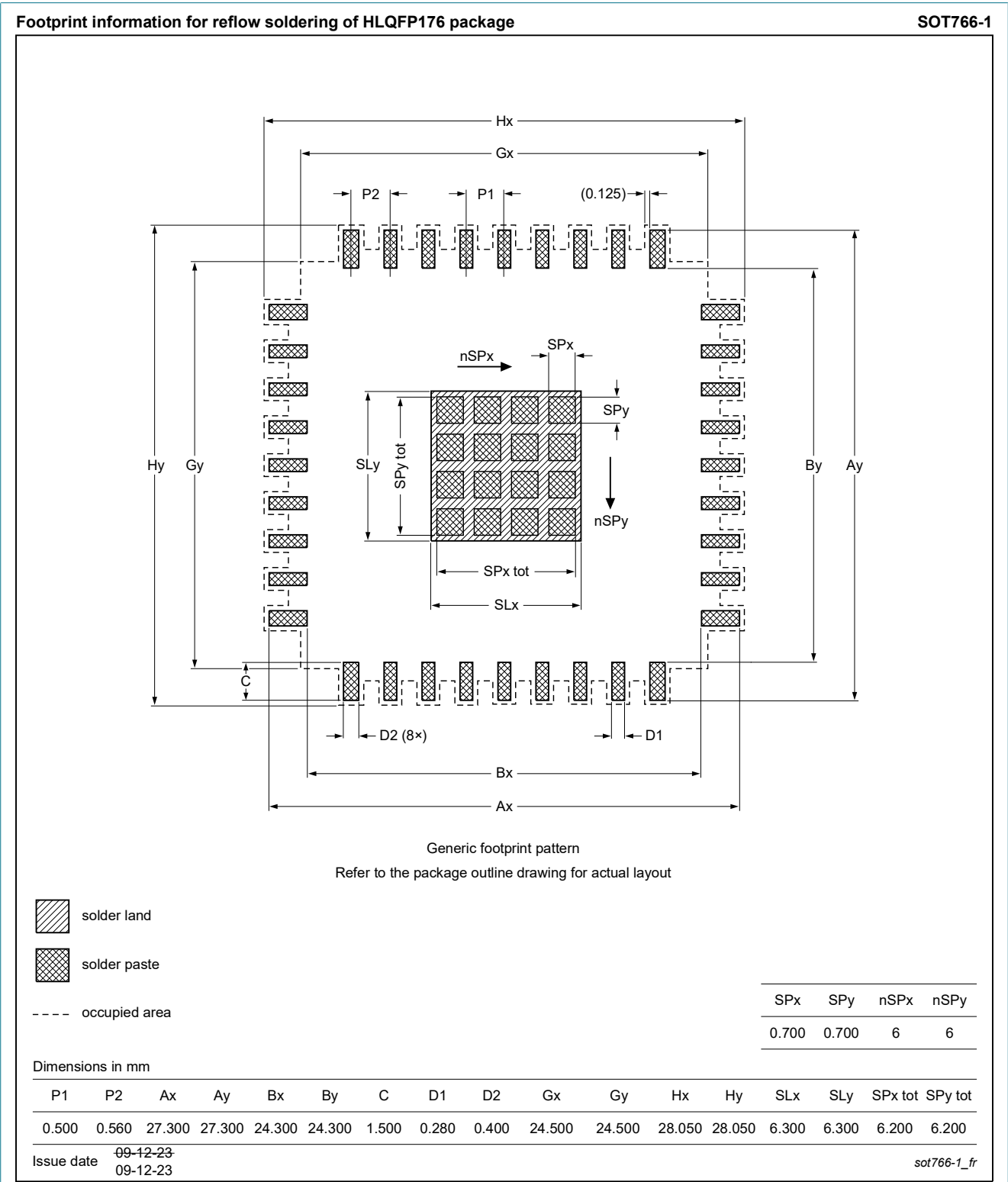
Fig. 2. Reflow soldering footprint for HLQFP176 (SOT766-1)
