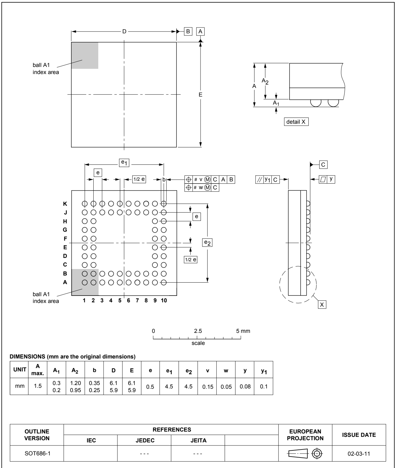
Fig. 1. Package outline LFBGA64 (SOT686-1)
