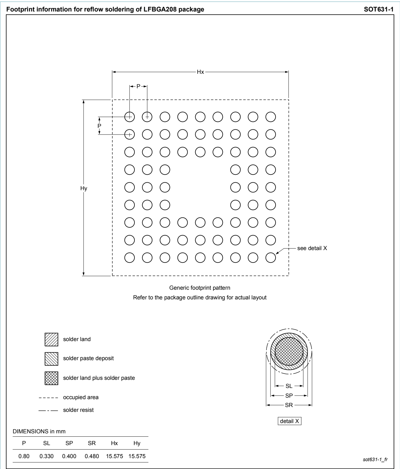
Fig. 2. Reflow soldering footprint for LFBGA208 (SOT631-1)
