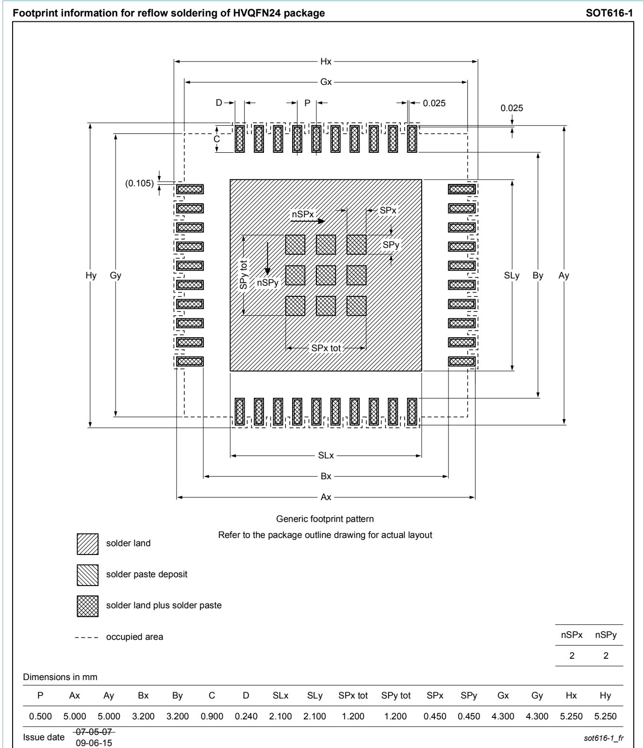
Fig. 2. Reflow soldering footprint for HVQFN24 (SOT616-1)
