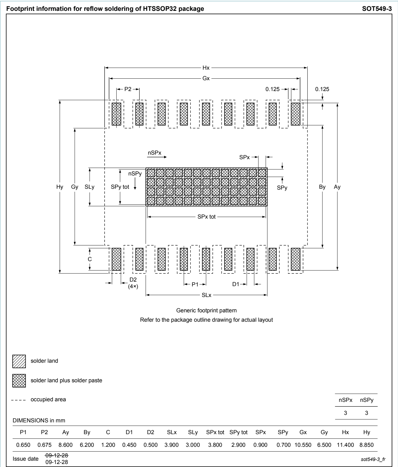
Fig. 2. Reflow soldering footprint for HTSSOP32 (SOT549-3)
