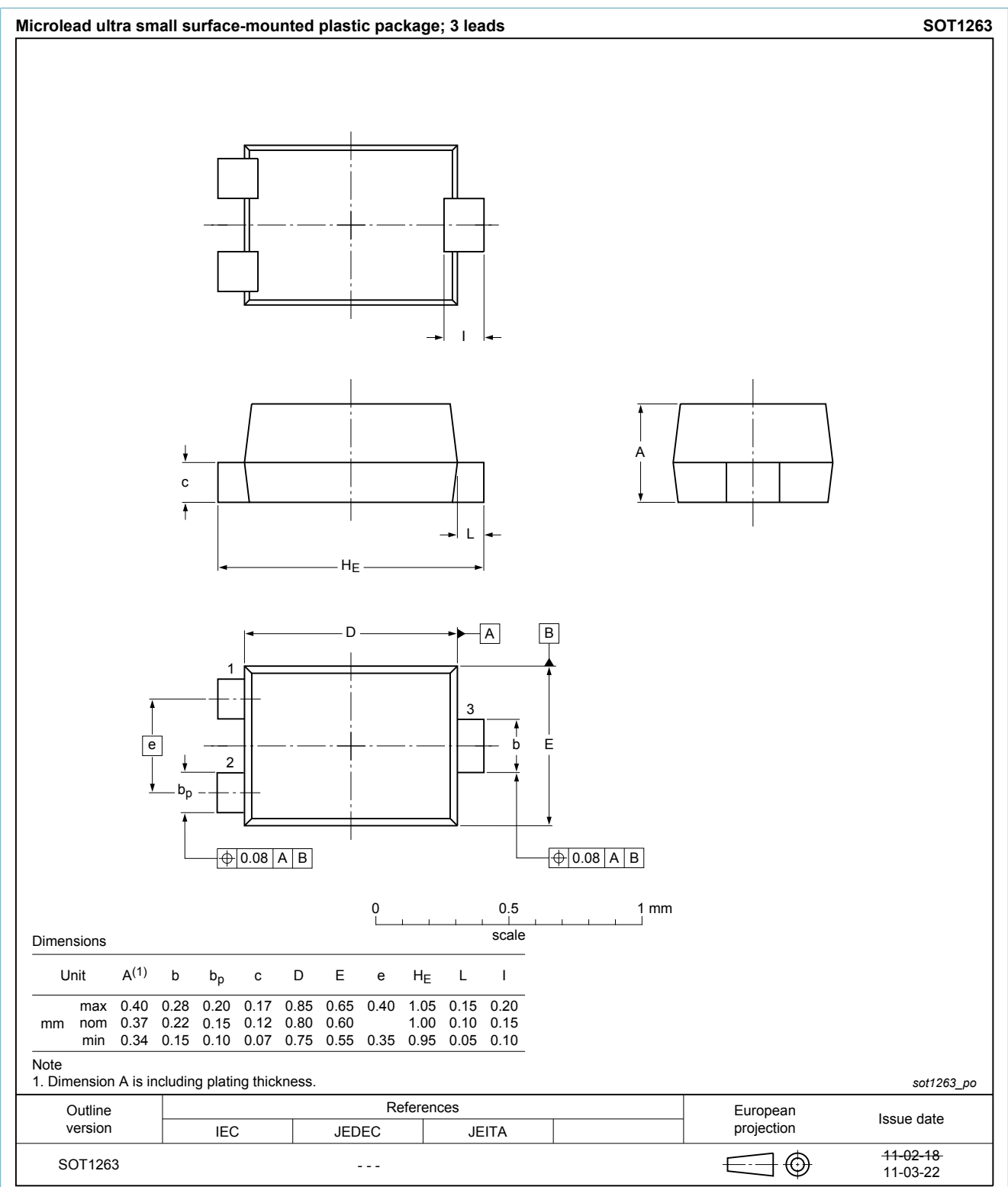
Fig. 1. Package outline SOT1263
