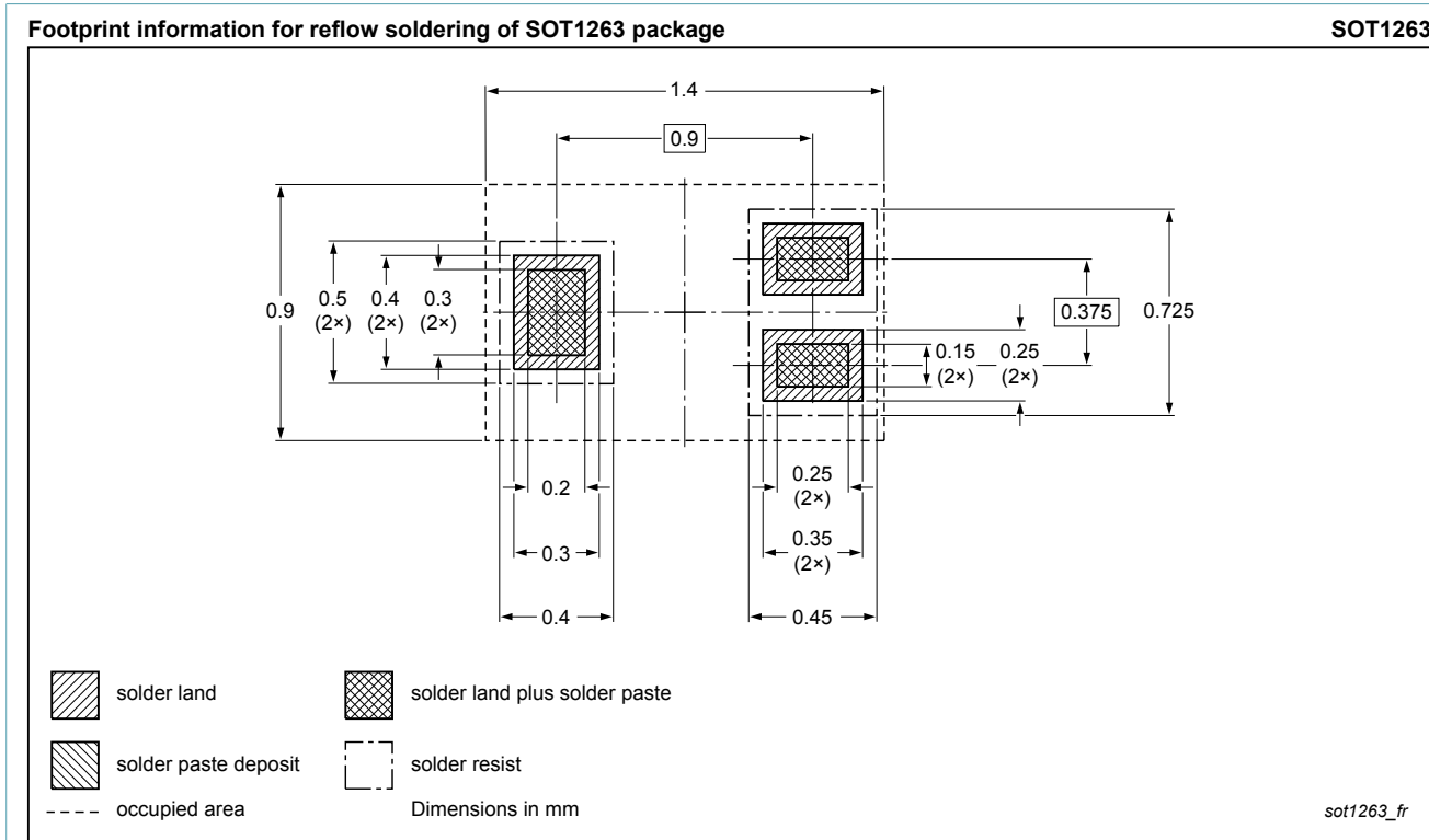
Fig. 2. Reflow soldering footprint for SOT1263
