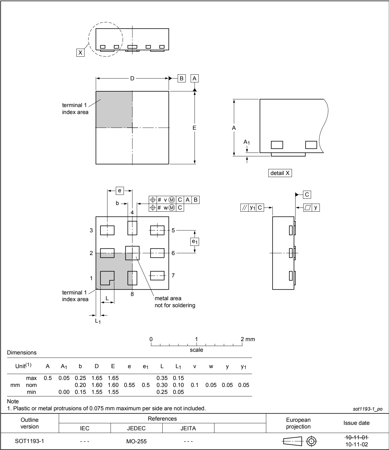
Fig. 1. Package outline XQFN8 (SOT1193-1)
