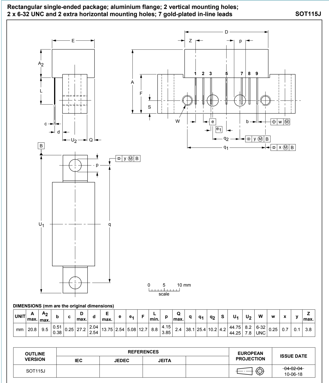
Figure 1. Package outline SFM7 (SOT115JA)
