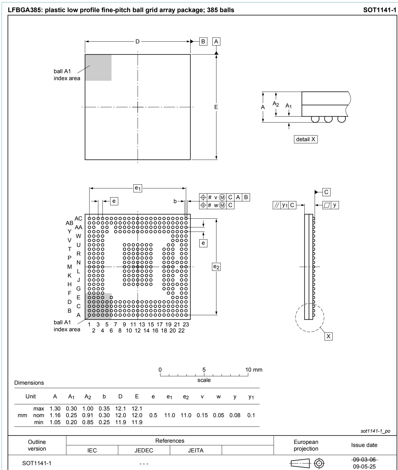
Fig. 1. Package outline LFBGA385 (SOT1141-1)
