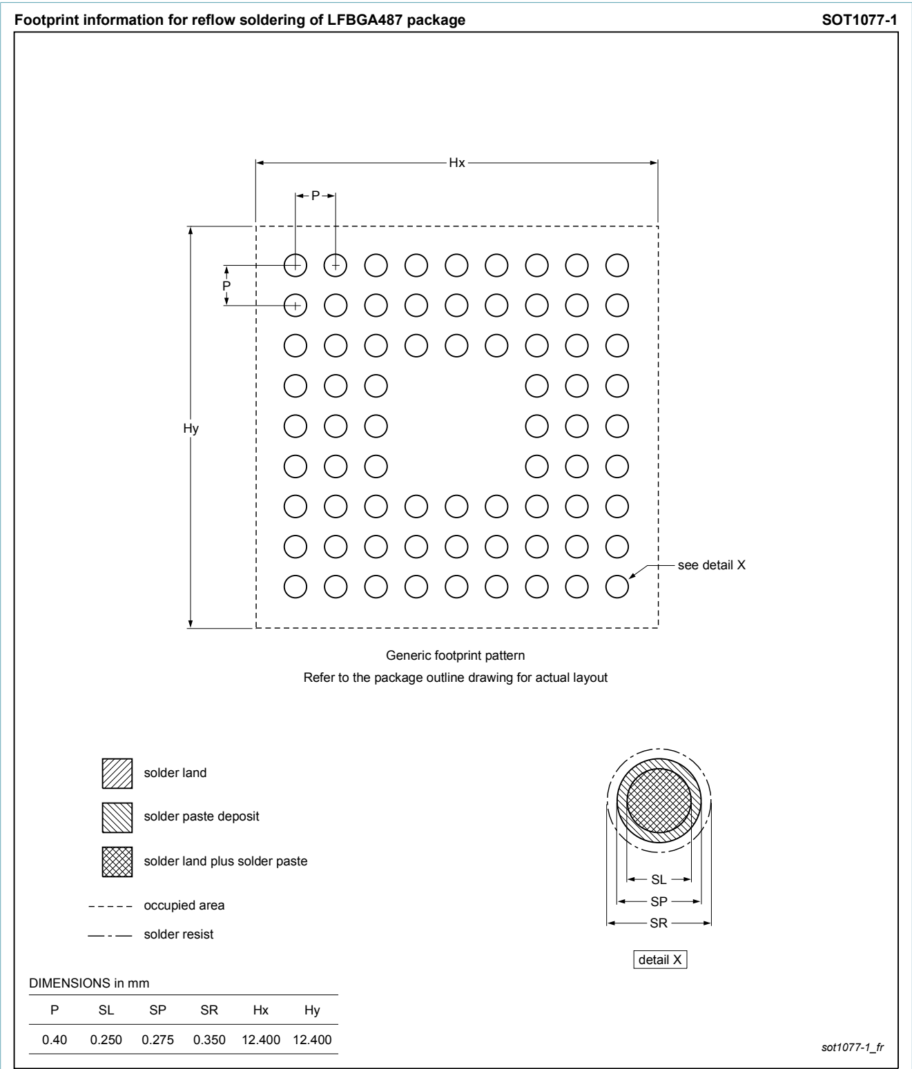
Fig. 2. Reflow soldering footprint for LFBGA487 (SOT1077-1)
