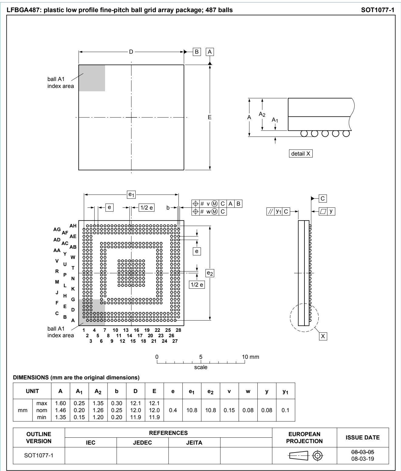
Fig. 1. Package outline LFBGA487 (SOT1077-1)
