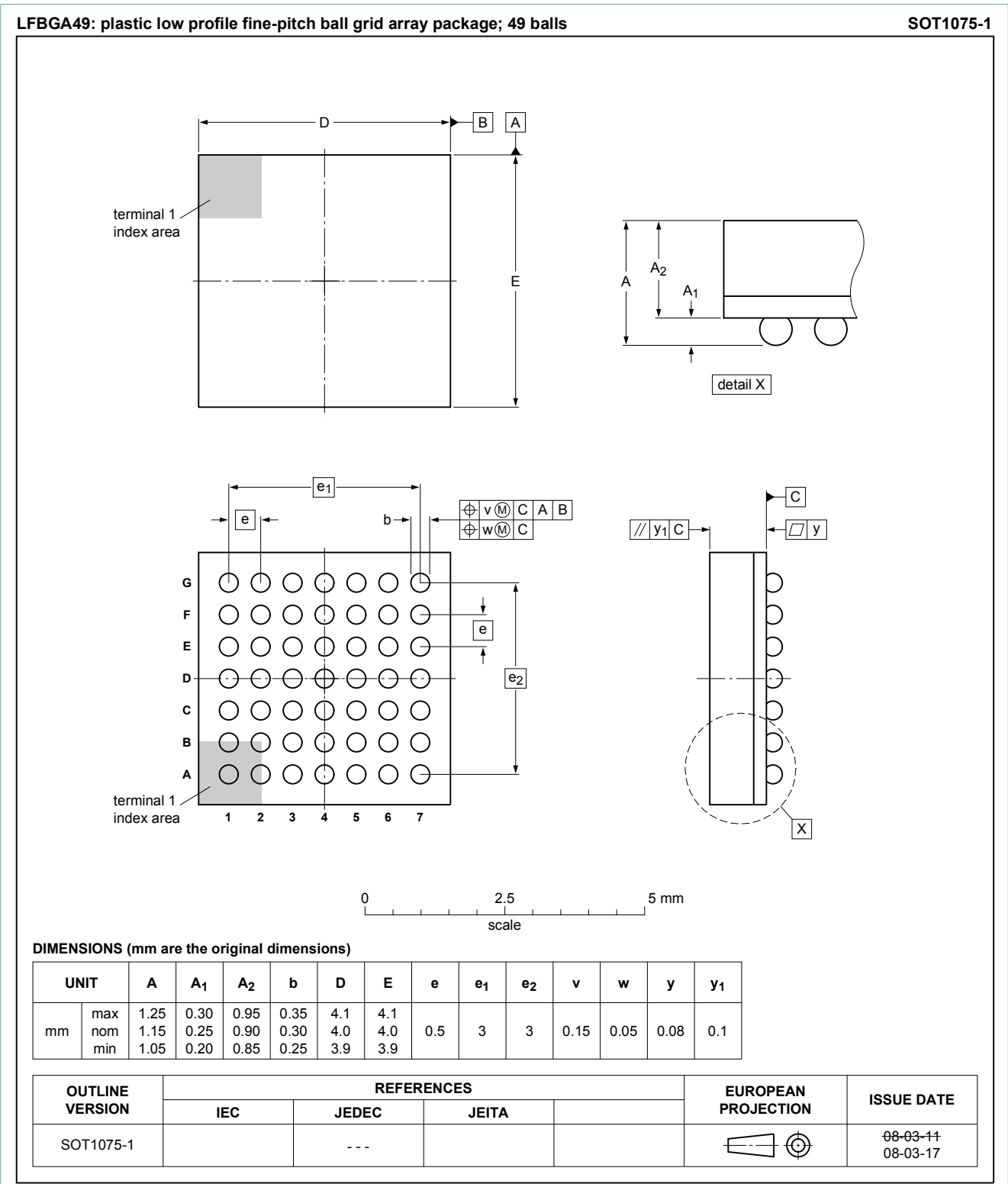
Fig. 1. Package outline LFBGA49 (SOT1075-1)
