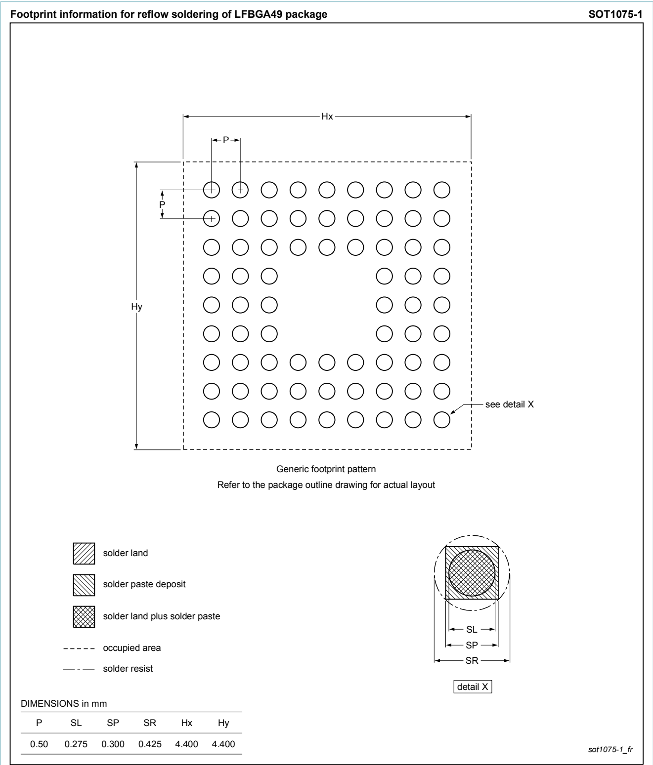
Fig. 2. Reflow soldering footprint for LFBGA49 (SOT1075-1)
