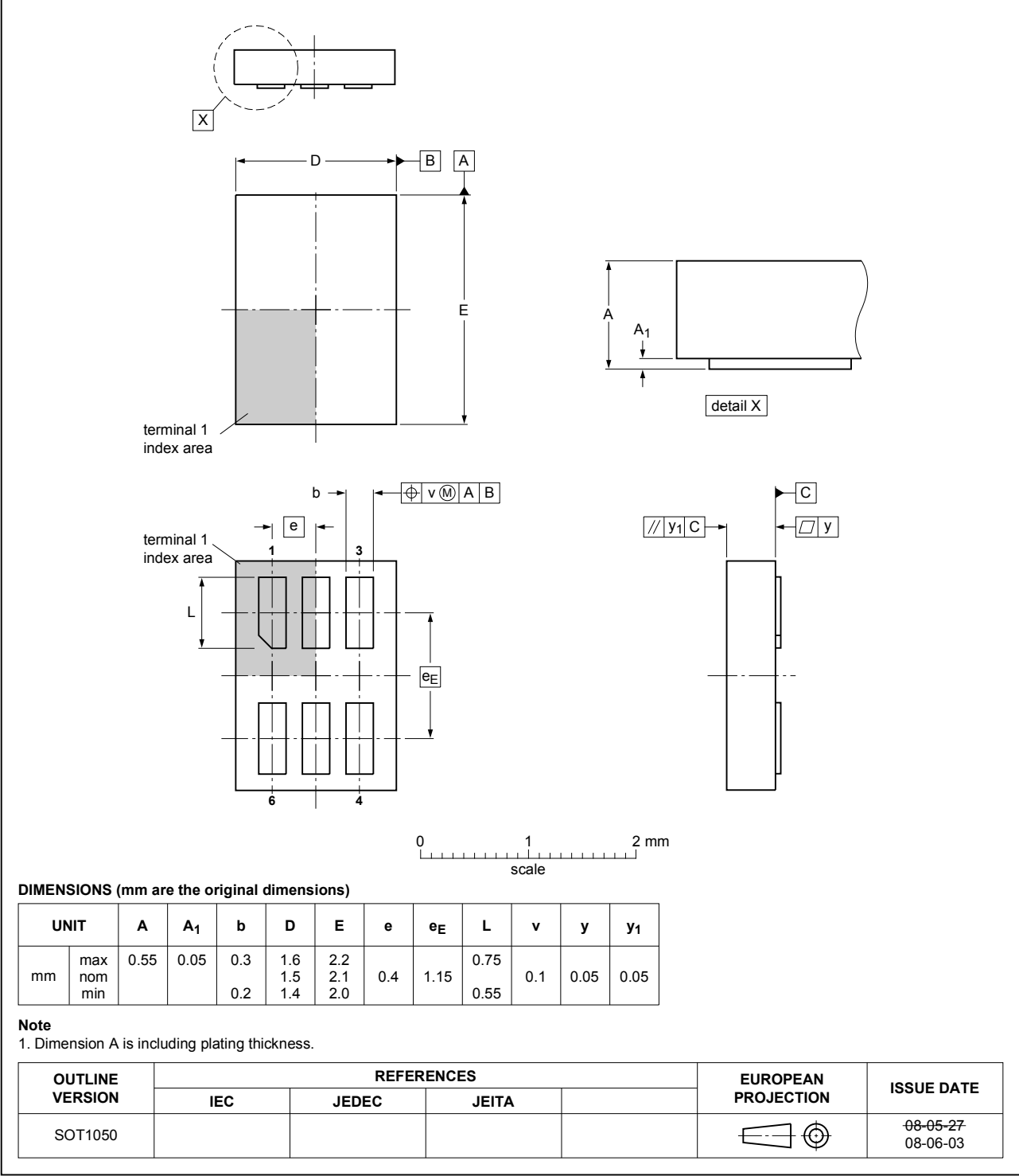
Fig. 1. Package outline USON6 (SOT1050)
