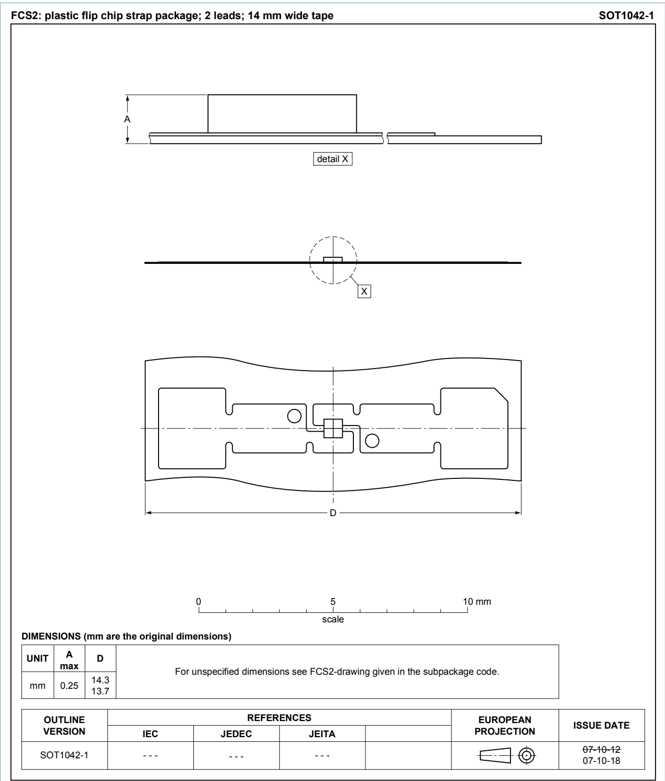
Fig. 1. Package outline FCS2 (SOT1042-1)
