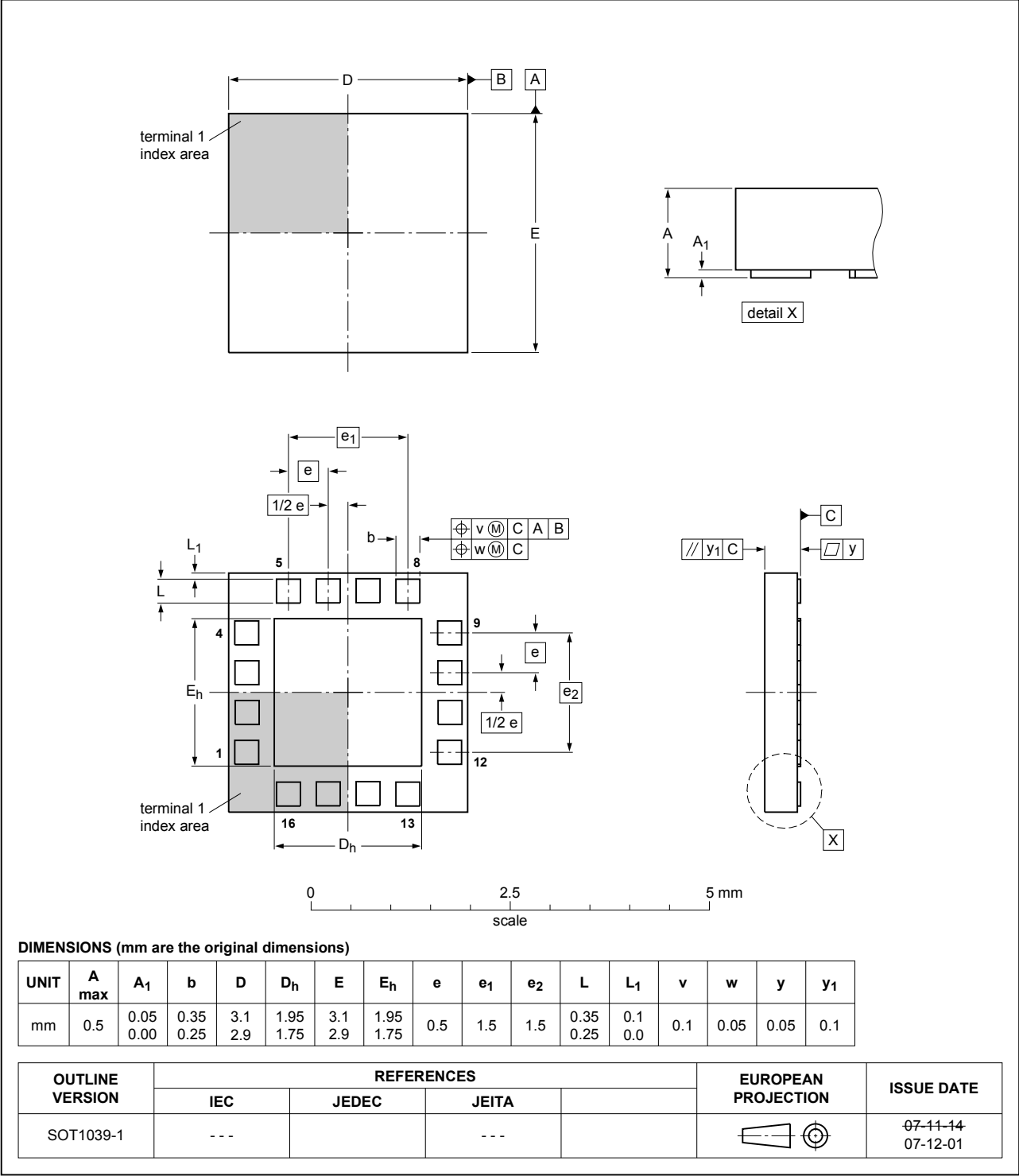
Fig. 1. Package outline HXQFN16U (SOT1039-1)
