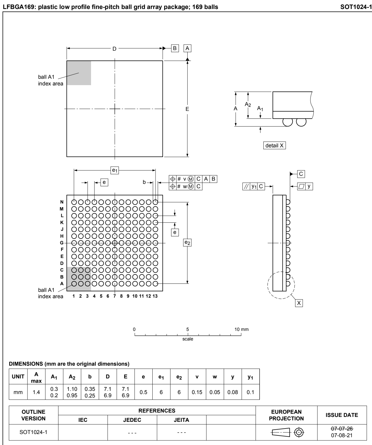
Fig. 1. Package outline LFBGA169 (SOT1024-1)
