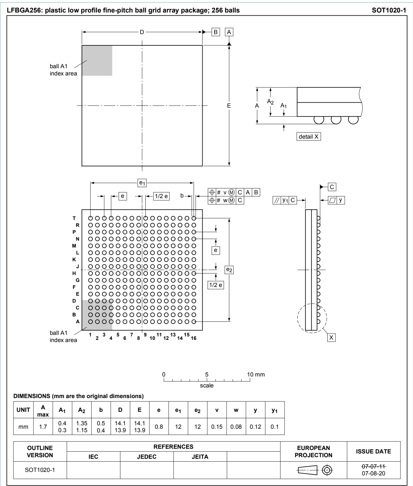
Fig. 1. Package outline LFBGA256 (SOT1020-1)
