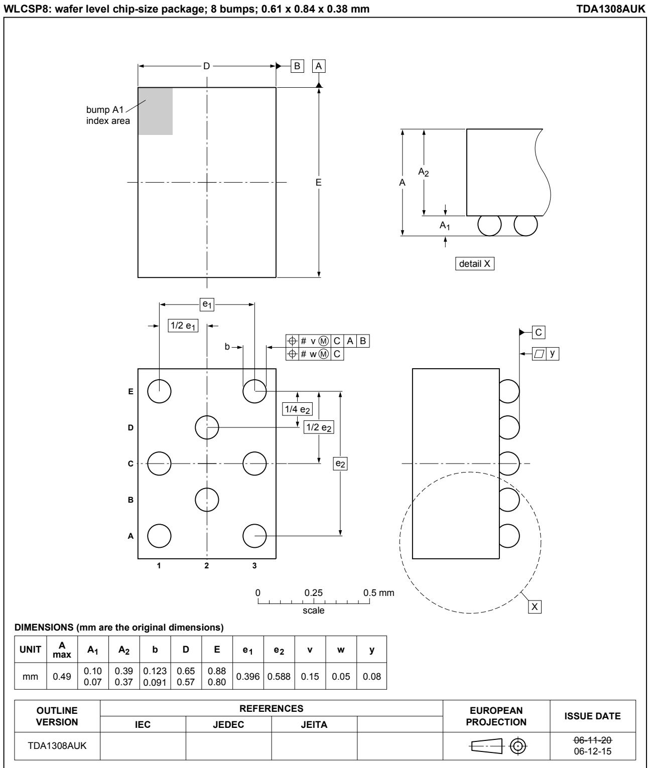
Fig. 1. Package outline WLCSP (OL-TDA1308AUK)
